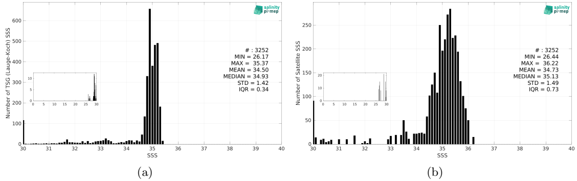
Figure 3: Histograms of SSS from TSG (Lauge-Koch) (a) and SMOS SSS L3 v332 - 9 Days (CATDS-CPDC) (b) considering all match-up pairs per bins of 0.1 over the Global Ocean Pi-MEP region and for the full satellite product period.
