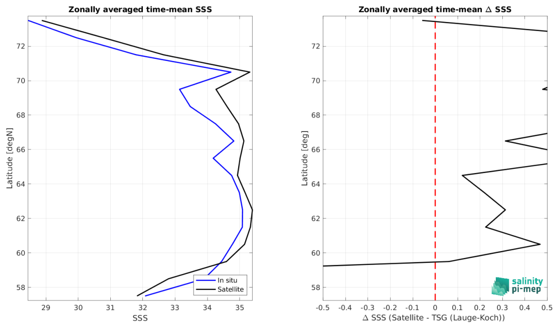
Figure 9: Left panel: Zonal mean SSS from SMOS SSS L3 v332 - 9 Days (CATDS-CPDC) satellite product (black) and from TSG (Lauge-Koch) (blue). Right panel: Zonal mean of \Delta SSS (Satellite - TSG (Lauge-Koch)) for all the collected Pi-MEP match-up pairs estimated over the full satellite product period.
