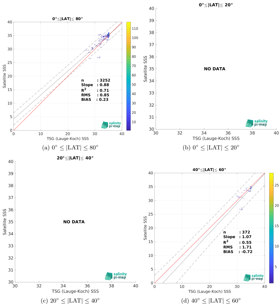
Figure 10: Contour maps of the concentration of SMOS SSS L3 v332 - 9 Days (CATDS-CPDC) SSS (y-axis) versus TSG (Lauge-Koch) SSS (x-axis) at match-up pairs for different latitude bands. For each plot, the red line shows x=y . The black thin and dashed lines indicate a linear fit through the data cloud and the \pm 95\% confidence levels, respectively. The number match-up pairs n , the slope and R^2 coefficient of the linear fit, the root mean square (RMS) and the mean bias between satellite and in situ data are indicated for each latitude band in each plots.
