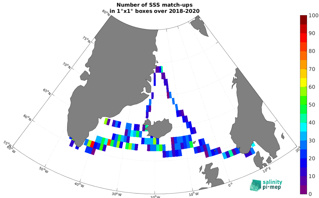
Figure 5: Number of SSS match-ups between TSG (Lauge-Koch) SSS and the SMOS SSS L3 v332 - 9 Days (CATDS-CPDC) SSS product for the Global Ocean Pi-MEP region over 1^\circ \times 1^\circ boxes and for the full satellite product period.
