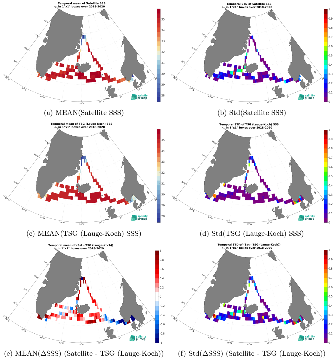
Figure 7: Temporal mean (left) and Std (right) of SSS from SMOS SSS L3 v332 - 9 Days (CATDS-CPDC) (top), TSG (Lauge-Koch) (middle), and of \Delta SSS (Satellite - TSG (Lauge-Koch)). Only match-up pairs are used to generate these maps.
