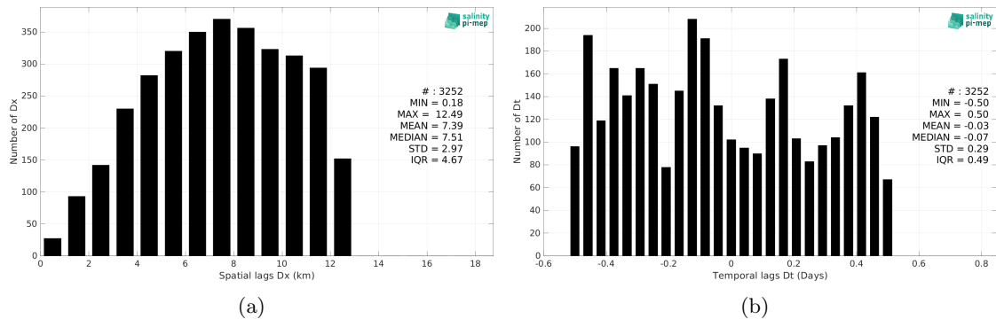
Figure 6: Histograms of the spatial (a) and temporal (b) lags between the location/time of the TSG (Lauge-Koch) measurement and the date of the corresponding SMOS SSS L3 v332 - 9 Days (CATDS-CPDC) SSS pixel.
