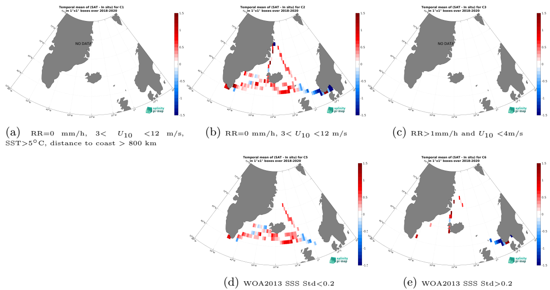
Figure 14: Temporal mean gridded over spatial boxes of size 1^\circ \times 1^\circ of \Delta SSS (SMOS SSS L3 v332 - 9 Days (CATDS-CPDC) - TSG (Lauge-Koch)) for 5 different subdatasets corresponding to:RR=0 mm/h, 3 < U_{10} < 12 m/s, SST>5°C, distance to coast > 800 km (a), RR=0 mm/h, 3 < U_{10} < 12 m/s (b), RR>1mm/h and U_{10} < 4 m/s (c), WOA2013 SSS Std<0.2 (d), WOA2013 SSS Std>0.2 (e).
