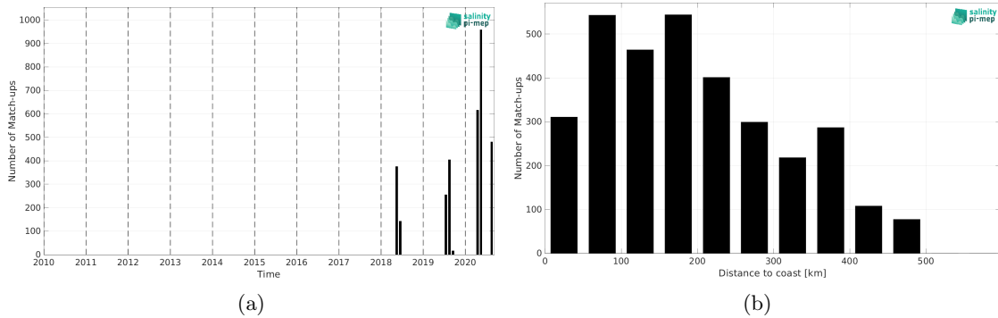
Figure 2: Number of match-ups between TSG (Lauge-Koch) and SMOS SSS L3 v332 - 9 Days (CATDS-CPDC) SSS as a function of time (a) and as function of the distance to coast (b) over the Global Ocean Pi-MEP region and for the full satellite product period.
