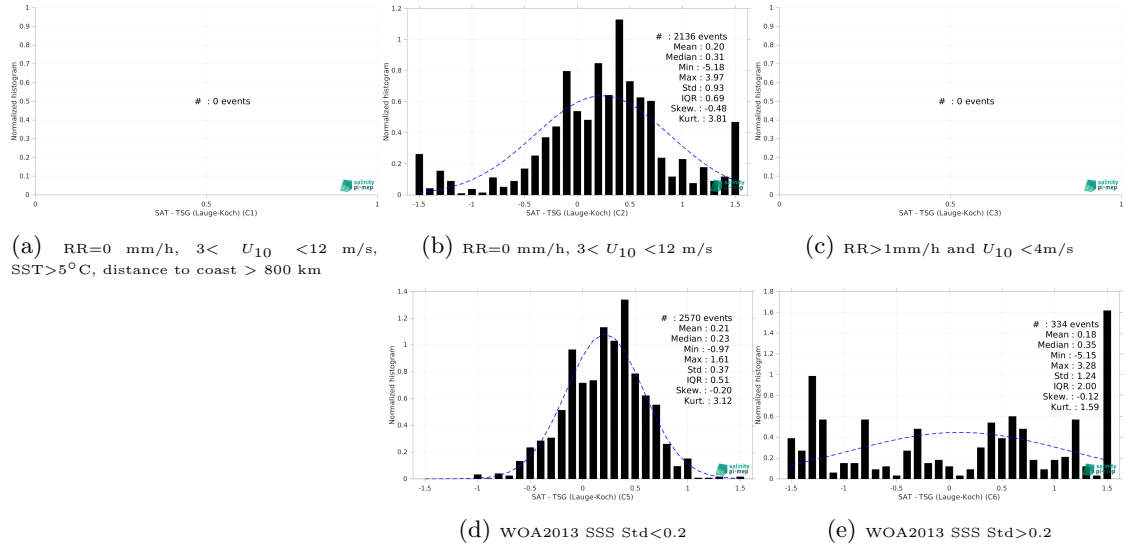
Figure 15: Normalized histogram of \Delta SSS (SMOS SSS L3 v332 - 9 Days (CATDS-CPDC) - TSG (Lauge-Koch)) for 5 different subdatasets corresponding to: RR=0 mm/h, 3 < U_{10} < 12 m/s, SST > 5°C, distance to coast > 800 km (a), RR=0 mm/h, 3 < U_{10} < 12 m/s (b), RR > 1mm/h and U_{10} < 4 m/s (c), WOA2013 SSS Std < 0.2 (d), WOA2013 SSS Std > 0.2 (e).
