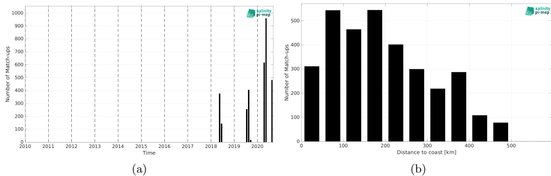
Figure 1: Number of match-ups between TSG (Lauge-Koch) and SMOS SSS L3 v332 - 9 Days (CATDS-CPDC) SSS as a function of time (a) and as function of the distance to coast (b) over the Global Ocean Pi-MEP region and for the full satellite product period.
