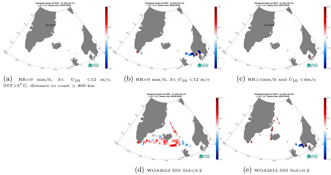
Figure 12: Temporal mean gridded over spatial boxes of size 1^{\circ}\times 1^{\circ} of \Delta\text{SSS} (SMOS SSS L3 v332 - 9 Days (CATDS-CPDC) - TSG (Lauge-Koch)) for 5 different subdatasets corresponding to:RR=0 mm/h, 3 < U_{10} < 12 m/s, SST > 5^{\circ}\text{C} , distance to coast > 800 km (a), RR=0 mm/h, 3 < U_{10} < 12 m/s (b), RR > 1 mm/h and U_{10} < 4 m/s (c), WOA2013 SSS Std < 0.2 (d), WOA2013 SSS Std > 0.2 (e).
