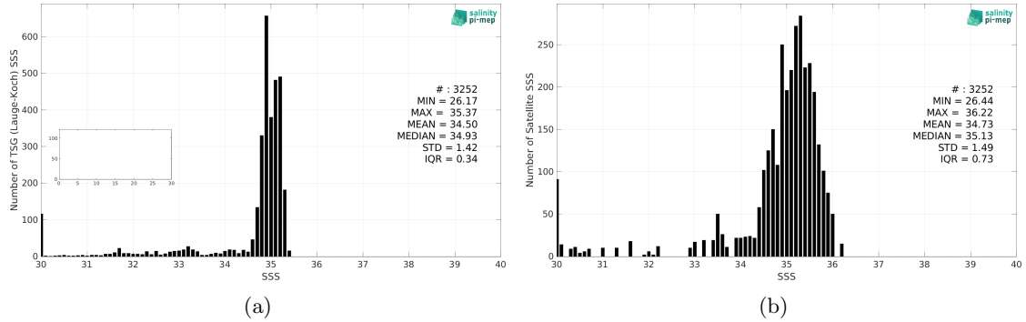
Figure 2: Histograms of SSS from TSG (Lauge-Koch) (a) and SMOS SSS L3 v332 - 9 Days (CATDS-CPDC) (b) considering all match-up pairs per bins of 0.1 over the Global Ocean Pi-MEP region and for the full satellite product period.
