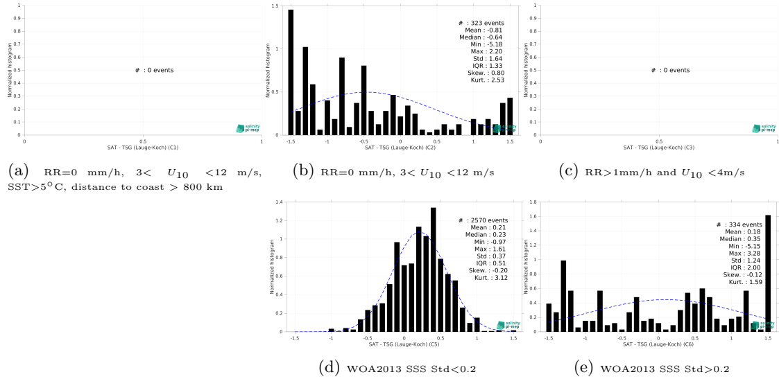
Figure 13: Normalized histogram of \Delta SSS (SMOS SSS L3 v332 - 9 Days (CATDS-CPDC) - TSG (Lauge-Koch)) for 5 different subdatasets corresponding to: RR=0 mm/h, 3 < U_{10} < 12 m/s, SST > 5°C, distance to coast > 800 km (a), RR=0 mm/h, 3 < U_{10} < 12 m/s (b), RR > 1mm/h and U_{10} < 4 m/s (c), WOA2013 SSS Std < 0.2 (d), WOA2013 SSS Std > 0.2 (e).
