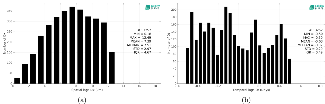
Figure 5: Histograms of the spatial (a) and temporal (b) lags between the location/time of the TSG (Lauge-Koch) measurement and the date of the corresponding SMOS SSS L3 v332 - 9 Days (CATDS-CPDC) SSS pixel.
