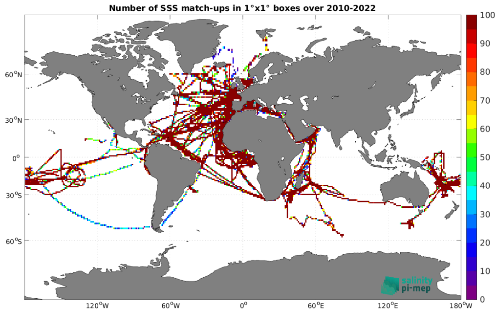
Figure 5: Number of SSS match-ups between TSG (GOSUD-Research-vessel) SSS and the SMOS SSS L3 v332 - 9 Days (CATDS-CPDC) SSS product for the Global Ocean Pi-MEP region over 1^\circ \times 1^\circ boxes and for the full satellite product period.
