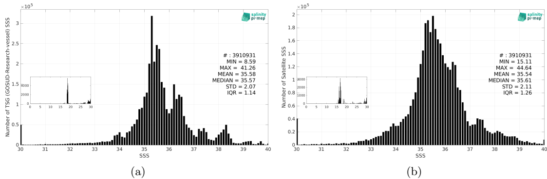
Figure 3: Histograms of SSS from TSG (GOSUD-Research-vessel) (a) and SMOS SSS L3 v332 - 9 Days (CATDS-CPDC) (b) considering all match-up pairs per bins of 0.1 over the Global Ocean Pi-MEP region and for the full satellite product period.
