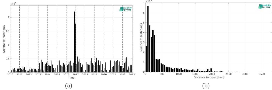
Figure 2: Number of match-ups between TSG (GOSUD-Research-vessel) and SMOS SSS L3 v332 - 9 Days (CATDS-CPDC) SSS as a function of time (a) and as function of the distance to coast (b) over the Global Ocean Pi-MEP region and for the full satellite product period.
