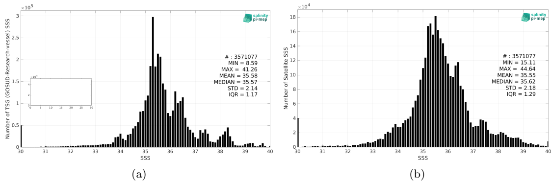
Figure 2: Histograms of SSS from TSG (GOSUD-Research-vessel) (a) and SMOS SSS L3 v332 - 9 Days (CATDS-CPDC) (b) considering all match-up pairs per bins of 0.1 over the Global Ocean Pi-MEP region and for the full satellite product period.
