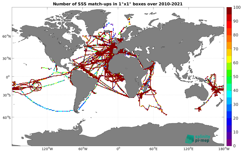
Figure 4: Number of SSS match-ups between TSG (GOSUD-Research-vessel) SSS and the SMOS SSS L3 v332 - 9 Days (CATDS-CPDC) SSS product for the Global Ocean Pi-MEP region over 1^\circ \times 1^\circ boxes and for the full satellite product period.
