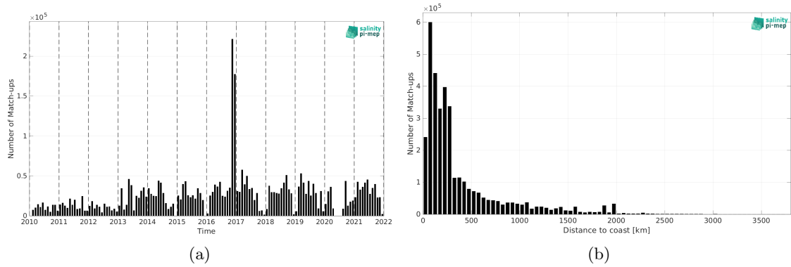
Figure 1: Number of match-ups between TSG (GOSUD-Research-vessel) and SMOS SSS L3 v332 - 9 Days (CATDS-CPDC) SSS as a function of time (a) and as function of the distance to coast (b) over the Global Ocean Pi-MEP region and for the full satellite product period.
