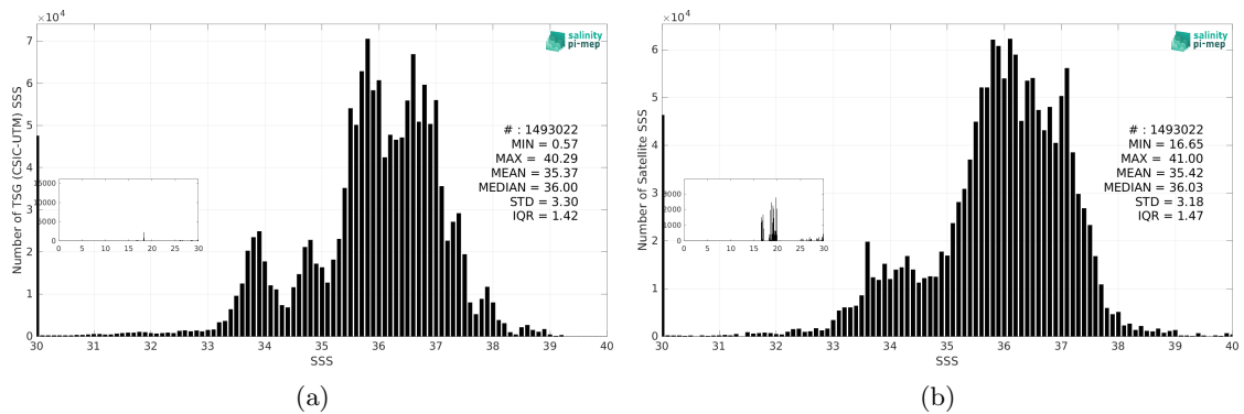
Figure 3: Histograms of SSS from TSG (CSIC-UTM) (a) and SMOS SSS L3 v332 - 9 Days (CATDS-CPDC) (b) considering all match-up pairs per bins of 0.1 over the Global Ocean Pi-MEP region and for the full satellite product period.
