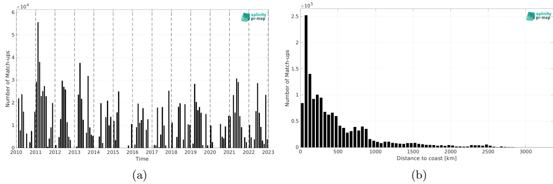
Figure 2: Number of match-ups between TSG (CSIC-UTM) and SMOS SSS L3 v332 - 9 Days (CATDS-CPDC) SSS as a function of time (a) and as function of the distance to coast (b) over the Global Ocean Pi-MEP region and for the full satellite product period.
