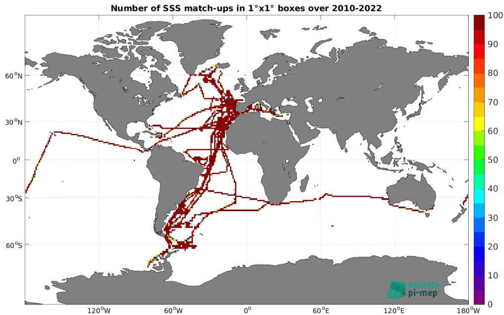
Figure 5: Number of SSS match-ups between TSG (CSIC-UTM) SSS and the SMOS SSS L3 v332 - 9 Days (CATDS-CPDC) SSS product for the Global Ocean Pi-MEP region over 1^\circ \times 1^\circ boxes and for the full satellite product period.
