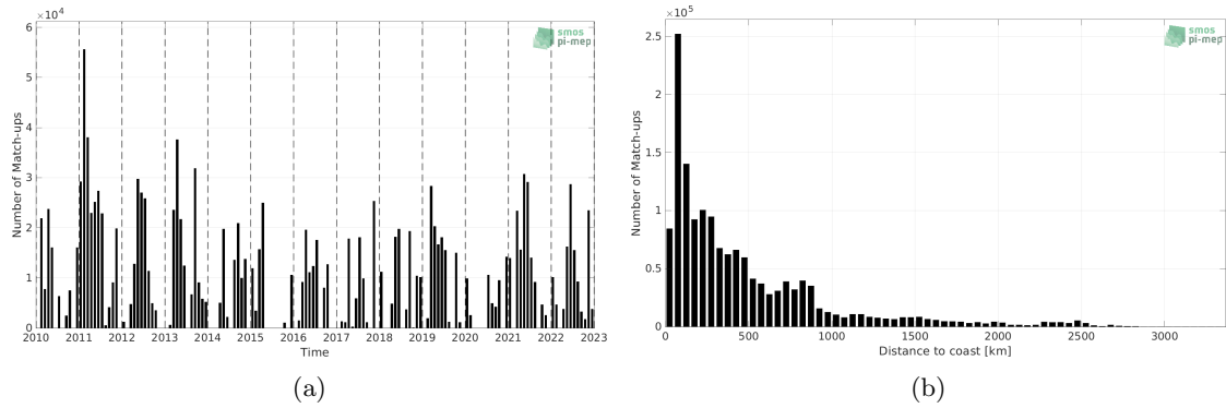
Figure 1: Number of match-ups between TSG (CSIC-UTM) and SMOS SSS L3 v332 - 9 Days (CATDS-CPDC) SSS as a function of time (a) and as function of the distance to coast (b) over the Global Ocean Pi-MEP region and for the full satellite product period.
