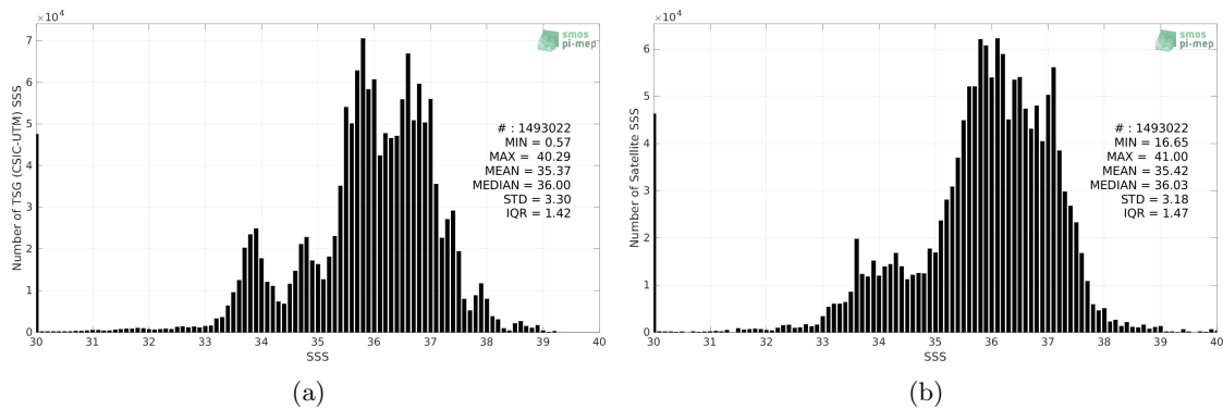
Figure 2: Histograms of SSS from TSG (CSIC-UTM) (a) and SMOS SSS L3 v332 - 9 Days (CATDS-CPDC) (b) considering all match-up pairs per bins of 0.1 over the Global Ocean Pi-MEP region and for the full satellite product period.
