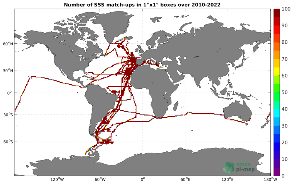
Figure 4: Number of SSS match-ups between TSG (CSIC-UTM) SSS and the SMOS SSS L3 v332 - 9 Days (CATDS-CPDC) SSS product for the Global Ocean Pi-MEP region over 1^\circ \times 1^\circ boxes and for the full satellite product period.
