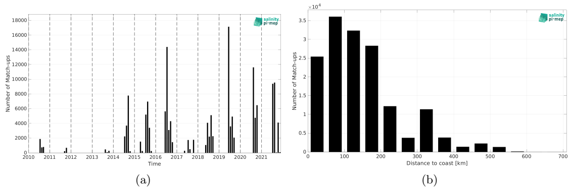
Figure 2: Number of match-ups between TSG (Amundsen) and SMOS SSS L3 v332 - 9 Days (CATDS-CPDC) SSS as a function of time (a) and as function of the distance to coast (b) over the Global Ocean Pi-MEP region and for the full satellite product period.
