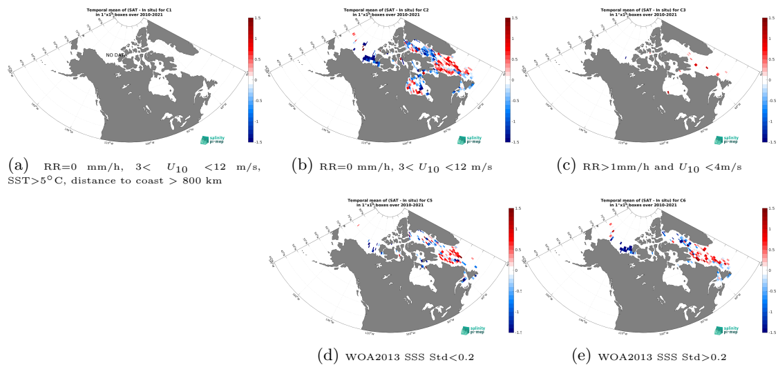
Figure 14: Temporal mean gridded over spatial boxes of size 1^\circ \times 1^\circ of \Delta SSS (SMOS SSS L3 v332 - 9 Days (CATDS-CPDC) - TSG (Amundsen)) for 5 different subdatasets corresponding to: RR=0 mm/h, 3 < U_{10} < 12 m/s, SST > 5°C, distance to coast > 800 km (a), RR=0 mm/h, 3 < U_{10} < 12 m/s (b), RR > 1mm/h and U_{10} < 4 m/s (c), WOA2013 SSS Std < 0.2 (d), WOA2013 SSS Std > 0.2 (e).
