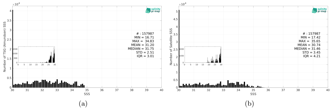
Figure 3: Histograms of SSS from TSG (Amundsen) (a) and SMOS SSS L3 v332 - 9 Days (CATDS-CPDC) (b) considering all match-up pairs per bins of 0.1 over the Global Ocean Pi-MEP region and for the full satellite product period.
