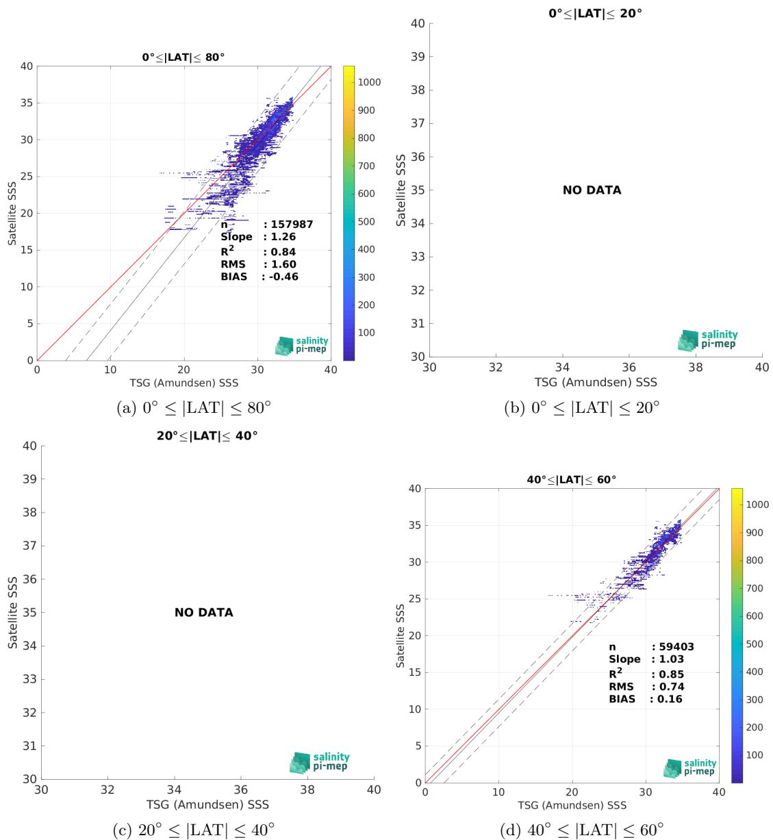
Figure 10: Contour maps of the concentration of SMOS SSS L3 v332 - 9 Days (CATDS-CPDC) SSS (y-axis) versus TSG (Amundsen) SSS (x-axis) at match-up pairs for different latitude bands. For each plot, the red line shows x=y . The black thin and dashed lines indicate a linear fit through the data cloud and the \pm 95\% confidence levels, respectively. The number match-up pairs n , the slope and R^2 coefficient of the linear fit, the root mean square (RMS) and the mean bias between satellite and in situ data are indicated for each latitude band in each plots.
