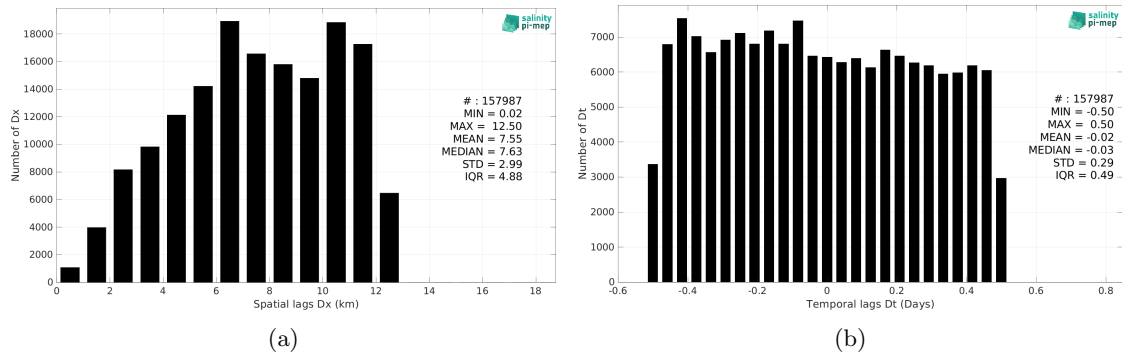
Figure 6: Histograms of the spatial (a) and temporal (b) lags between the location/time of the TSG (Amundsen) measurement and the date of the corresponding SMOS SSS L3 v332 - 9 Days (CATDS-CPDC) SSS pixel.
