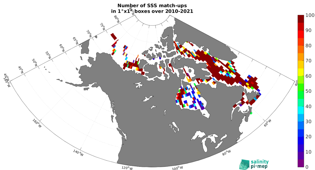
Figure 5: Number of SSS match-ups between TSG (Amundsen) SSS and the SMOS SSS L3 v332 - 9 Days (CATDS-CPDC) SSS product for the Global Ocean Pi-MEP region over 1^\circ \times 1^\circ boxes and for the full satellite product period.
