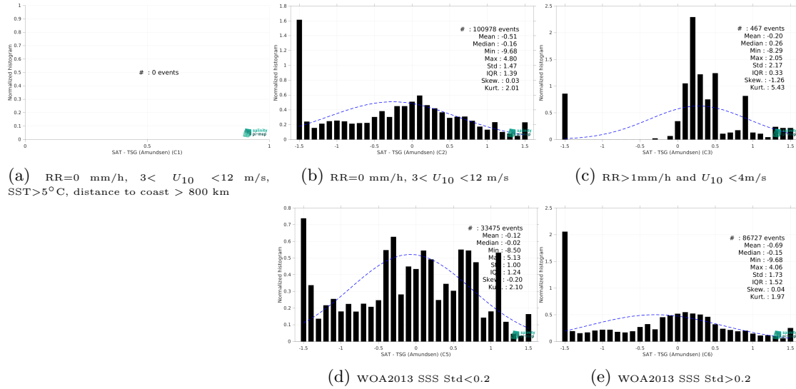
Figure 15: Normalized histogram of \Delta SSS (SMOS SSS L3 v332 - 9 Days (CATDS-CPDC) - TSG (Amundsen)) for 5 different subdatasets corresponding to: RR=0 mm/h, 3 < U_{10} < 12 m/s, SST > 5°C, distance to coast > 800 km (a), RR=0 mm/h, 3 < U_{10} < 12 m/s (b), RR > 1mm/h and U_{10} < 4 m/s (c), WOA2013 SSS Std < 0.2 (d), WOA2013 SSS Std > 0.2 (e).
