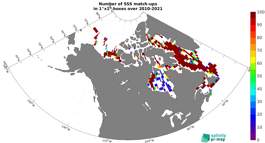
Figure 4: Number of SSS match-ups between TSG (Amundsen) SSS and the SMOS SSS L3 v332 - 9 Days (CATDS-CPDC) SSS product for the Global Ocean Pi-MEP region over 1^\circ \times 1^\circ boxes and for the full satellite product period.
