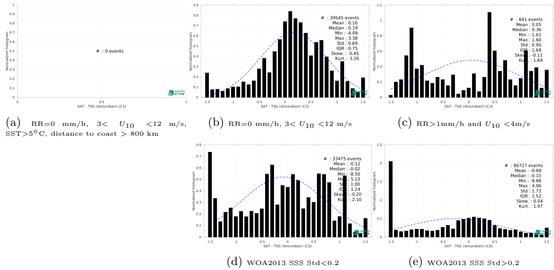
Figure 13: Normalized histogram of \Delta SSS (SMOS SSS L3 v332 - 9 Days (CATDS-CPDC) - TSG (Amundsen)) for 5 different subdatasets corresponding to: RR=0 mm/h, 3 < U_{10} < 12 m/s, SST > 5°C, distance to coast > 800 km (a), RR=0 mm/h, 3 < U_{10} < 12 m/s (b), RR > 1mm/h and U_{10} < 4 m/s (c), WOA2013 SSS Std < 0.2 (d), WOA2013 SSS Std > 0.2 (e).
