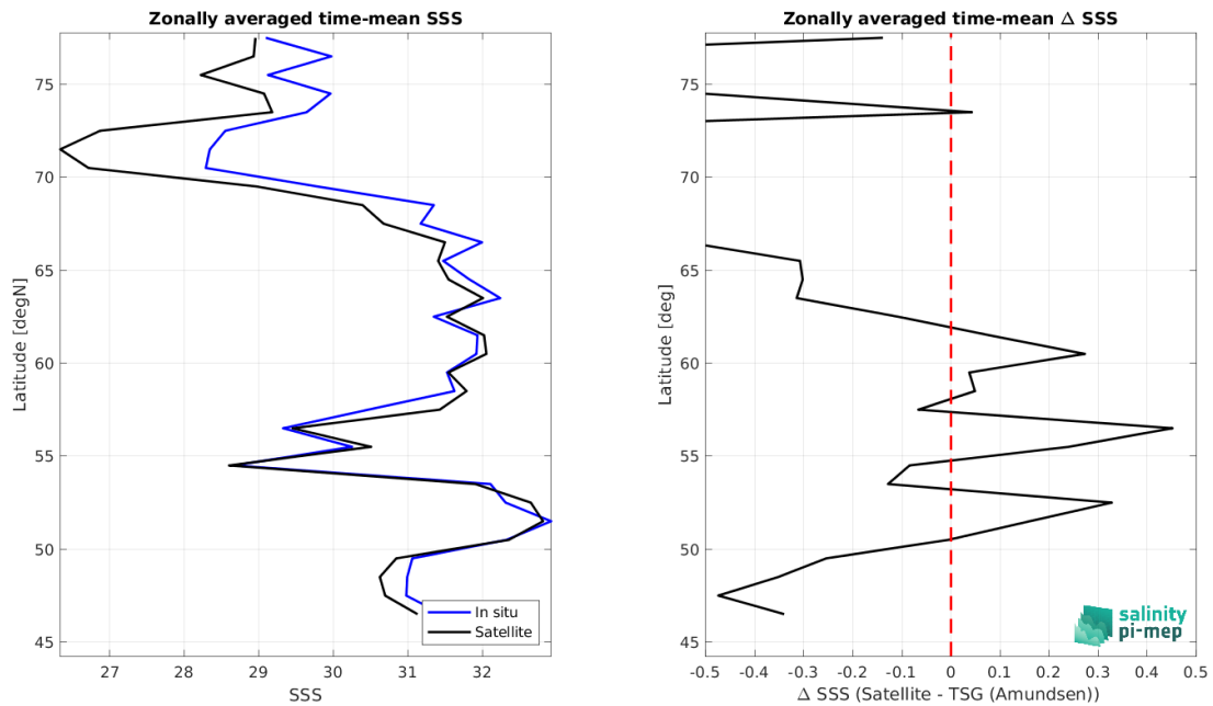
Figure 8: Left panel: Zonal mean SSS from SMOS SSS L3 v332 - 9 Days (CATDS-CPDC) satellite product (black) and from TSG (Amundsen) (blue). Right panel: Zonal mean of \Delta SSS (Satellite - TSG (Amundsen)) for all the collected Pi-MEP match-up pairs estimated over the full satellite product period.
