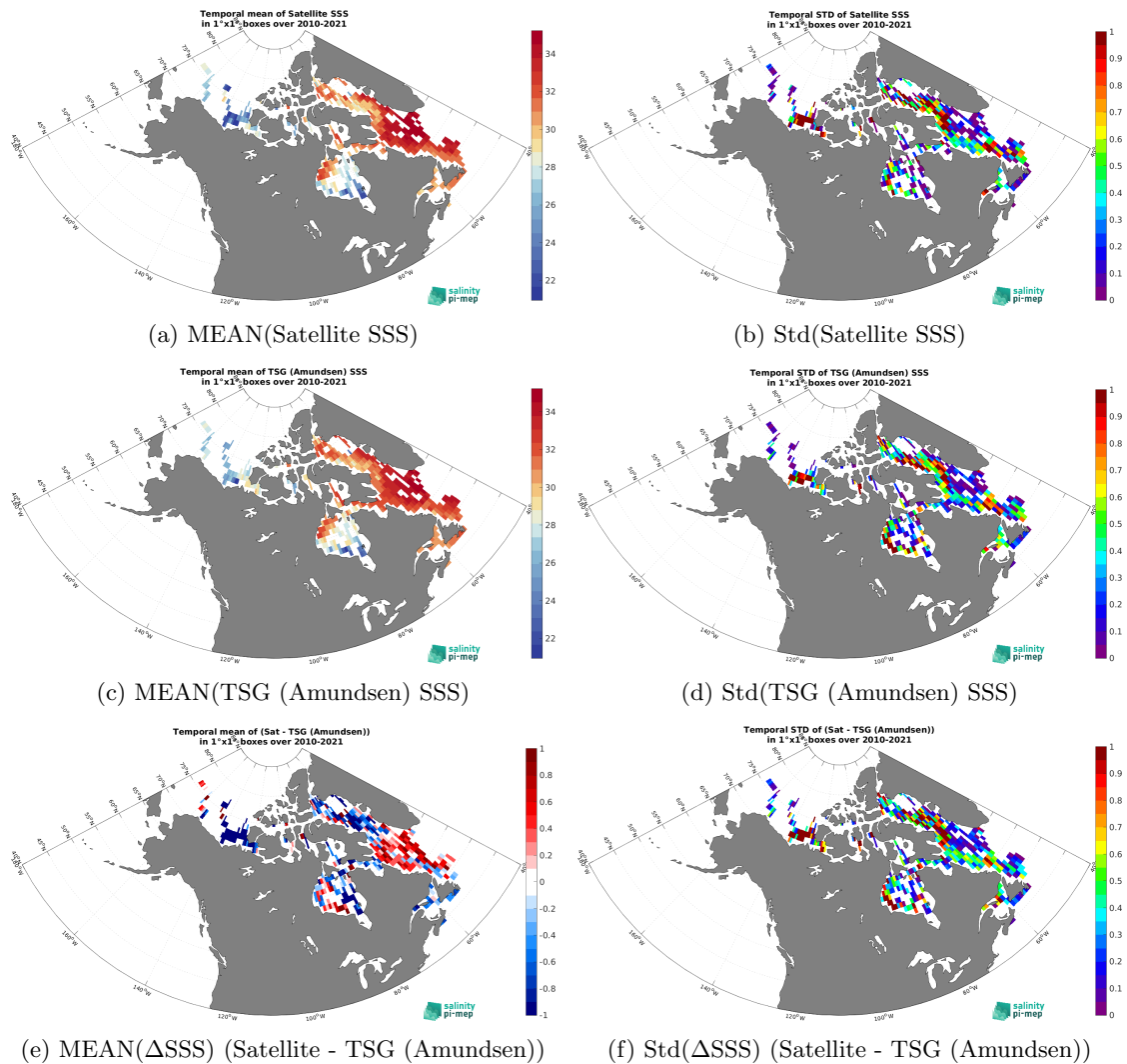
Figure 6: Temporal mean (left) and Std (right) of SSS from SMOS SSS L3 v332 - 9 Days (CATDS-CPDC) (top), TSG (Amundsen) (middle), and of \Delta SSS (Satellite - TSG (Amundsen)). Only match-up pairs are used to generate these maps.
