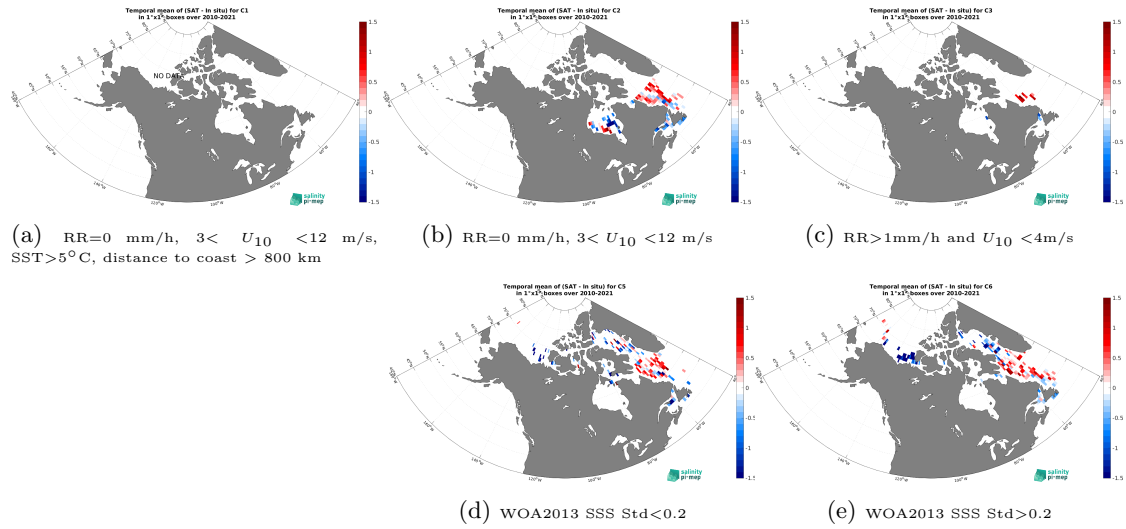
Figure 12: Temporal mean gridded over spatial boxes of size 1^{\circ}\times 1^{\circ} of \Delta\text{SSS} (SMOS SSS L3 v332 - 9 Days (CATDS-CPDC) - TSG (Amundsen)) for 5 different subdatasets corresponding to:RR=0 mm/h, 3 < U_{10} < 12 m/s, SST > 5^{\circ}\text{C} , distance to coast > 800 km (a), RR=0 mm/h, 3 < U_{10} < 12 m/s (b), RR > 1 mm/h and U_{10} < 4 m/s (c), WOA2013 SSS Std < 0.2 (d), WOA2013 SSS Std > 0.2 (e).
