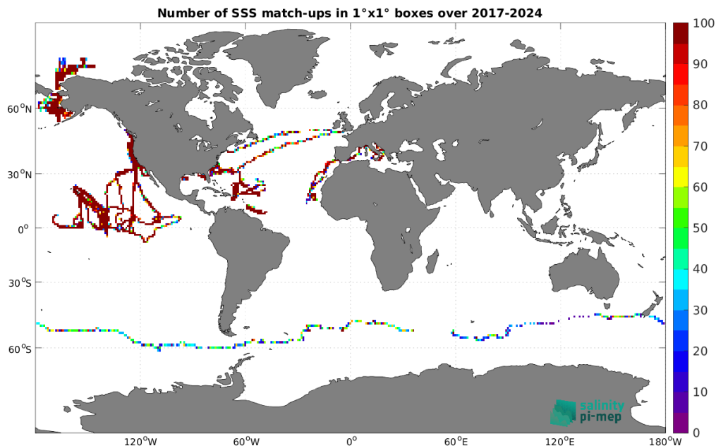
Figure 5: Number of SSS match-ups between Saildrone SSS and the SMOS SSS L3 v332 - 9 Days (CATDS-CPDC) SSS product for the Global Ocean Pi-MEP region over 1^\circ \times 1^\circ boxes and for the full satellite product period.
