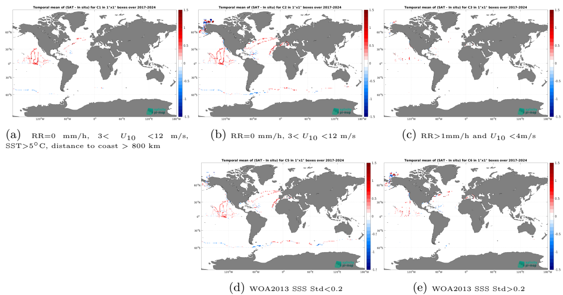
Figure 14: Temporal mean gridded over spatial boxes of size 1^\circ \times 1^\circ of \Delta SSS (SMOS SSS L3 v332 - 9 Days (CATDS-CPDC) - Saildrone) for 5 different subdatasets corresponding to:RR=0 mm/h, 3 < U_{10} < 12 m/s, SST > 5^\circ\text{C} , distance to coast > 800 km (a), RR=0 mm/h, 3 < U_{10} < 12 m/s (b), RR > 1 mm/h and U_{10} < 4 m/s (c), WOA2013 SSS Std < 0.2 (d), WOA2013 SSS Std > 0.2 (e).
