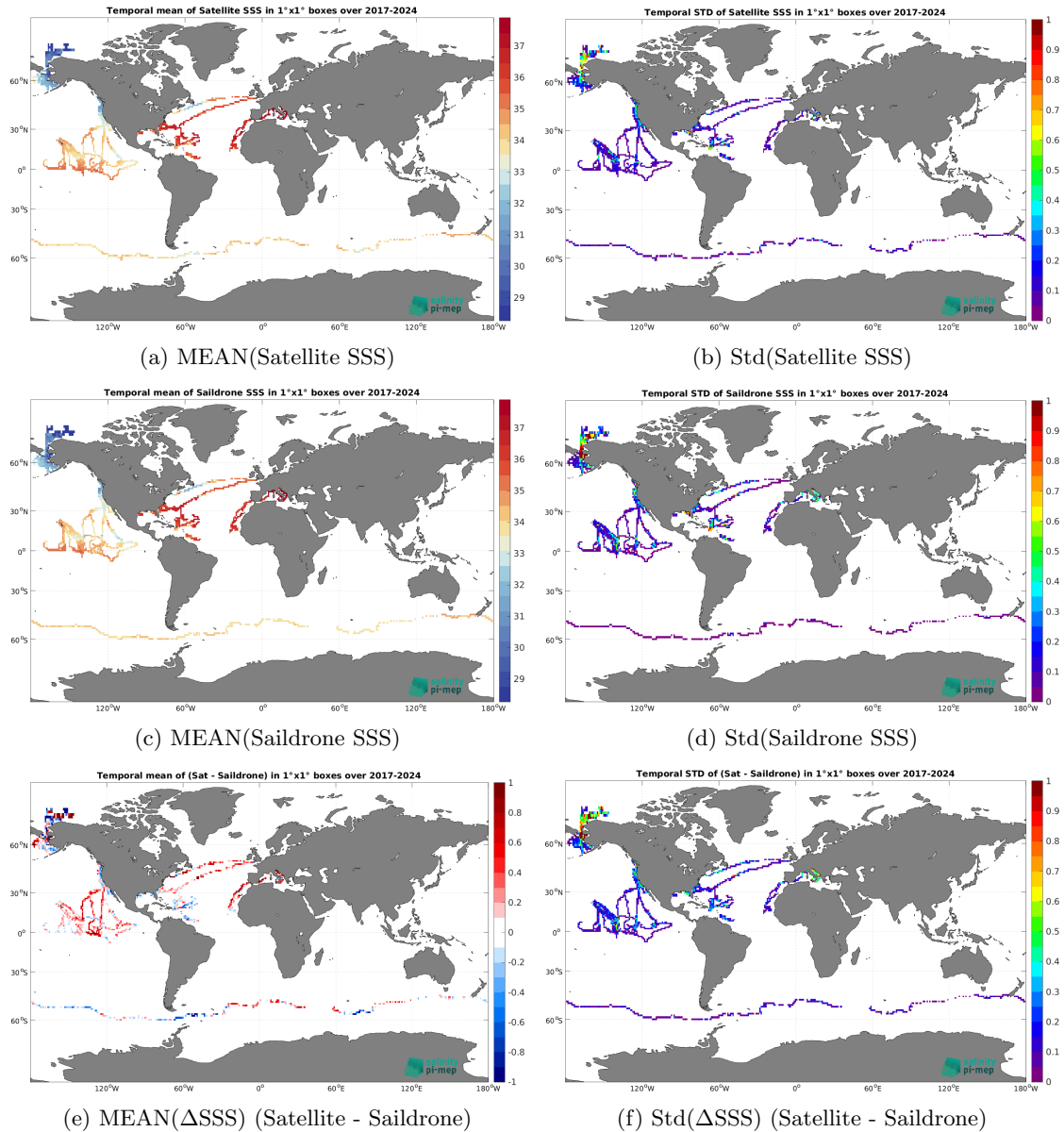
Figure 7: Temporal mean (left) and Std (right) of SSS from SMOS SSS L3 v332 - 9 Days (CATDS-CPDC) (top), Saildrone (middle), and of \Delta SSS (Satellite - Saildrone). Only match-up pairs are used to generate these maps.
