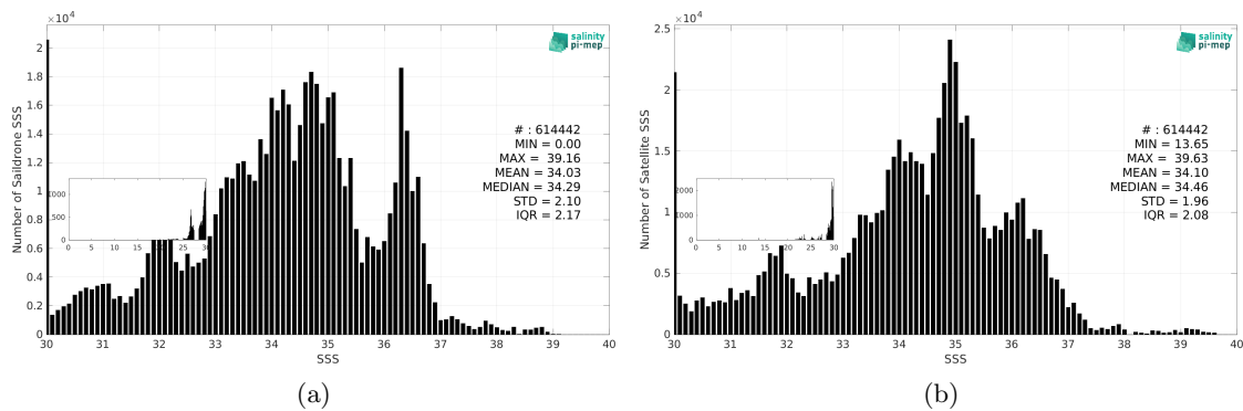
Figure 3: Histograms of SSS from Saildrone (a) and SMOS SSS L3 v332 - 9 Days (CATDS-CPDC) (b) considering all match-up pairs per bins of 0.1 over the Global Ocean Pi-MEP region and for the full satellite product period.
