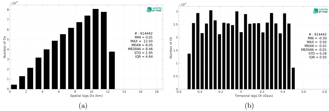
Figure 6: Histograms of the spatial (a) and temporal (b) lags between the location/time of the Sailability measurement and the date of the corresponding SMOS SSS L3 v332 - 9 Days (CATDS-CPDC) SSS pixel.
