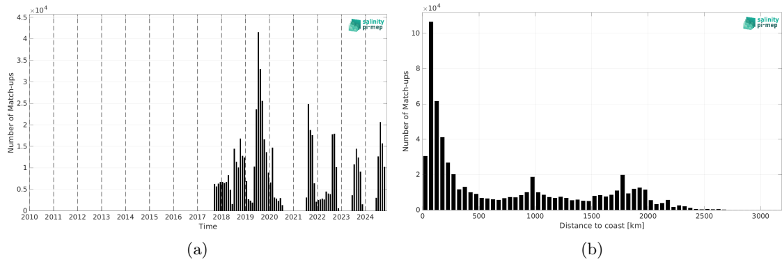
Figure 2: Number of match-ups between Saildrone and SMOS SSS L3 v332 - 9 Days (CATDS-CPDC) SSS as a function of time (a) and as function of the distance to coast (b) over the Global Ocean Pi-MEP region and for the full satellite product period.
