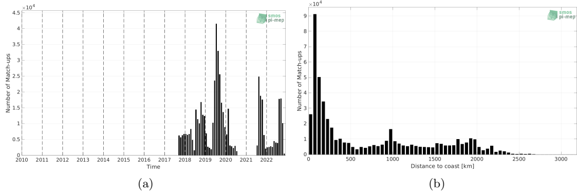
Figure 1: Number of match-ups between Saildrone and SMOS SSS L3 v332 - 9 Days (CATDS-CPDC) SSS as a function of time (a) and as function of the distance to coast (b) over the Global Ocean Pi-MEP region and for the full satellite product period.
