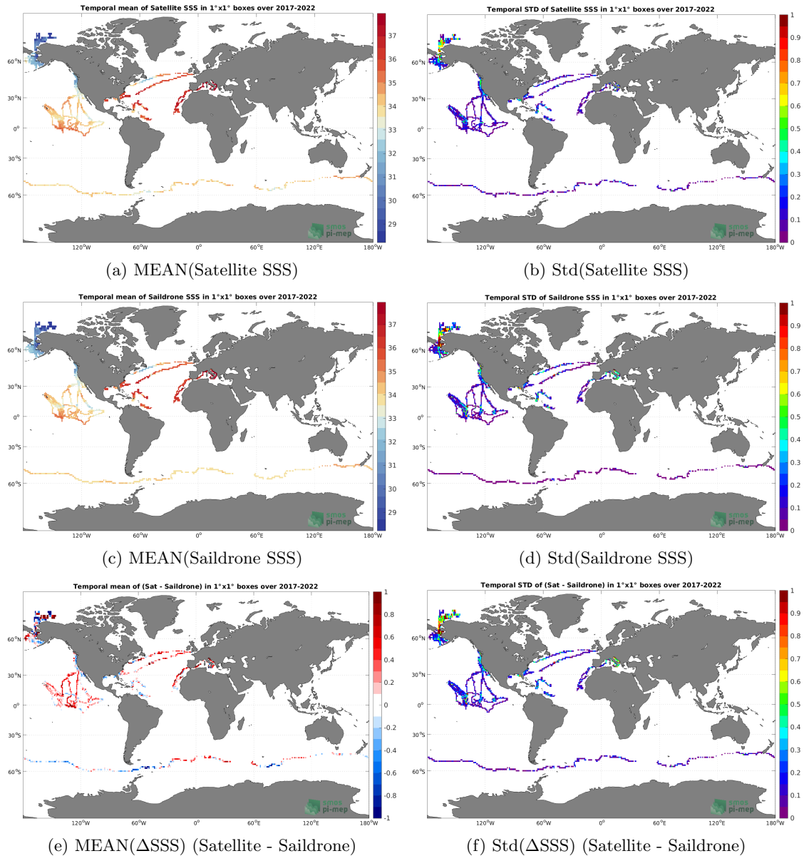
Figure 6: Temporal mean (left) and Std (right) of SSS from SMOS SSS L3 v332 - 9 Days (CATDS-CPDC) (top), Saildrone (middle), and of \Delta SSS (Satellite - Saildrone). Only match-up pairs are used to generate these maps.
