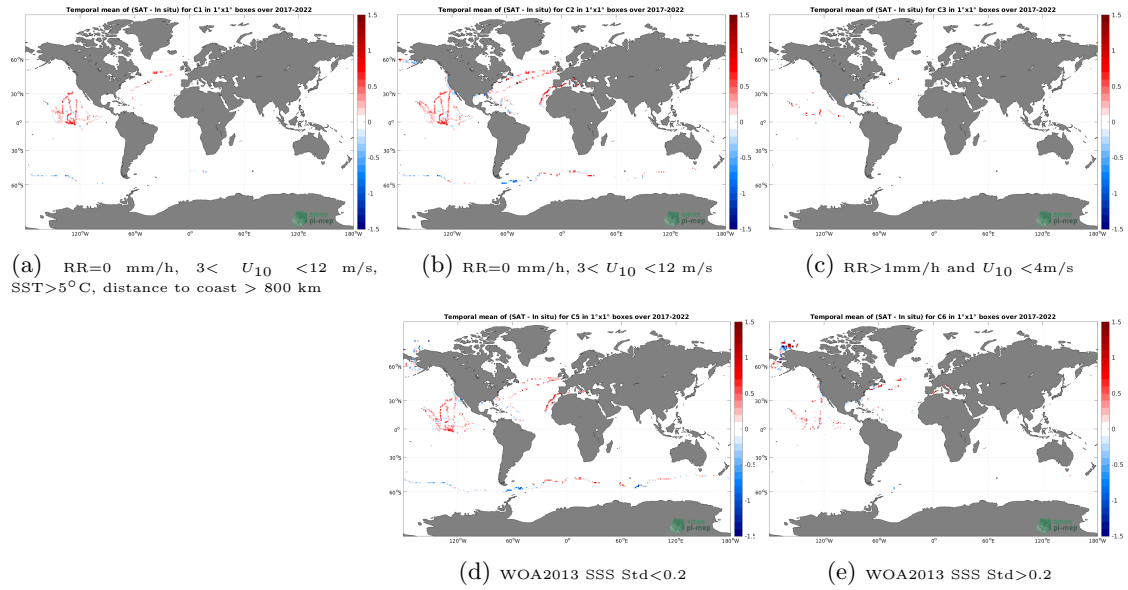
Figure 12: Temporal mean gridded over spatial boxes of size 1^\circ \times 1^\circ of \Delta SSS (SMOS SSS L3 v332 - 9 Days (CATDS-CPDC) - Sairdrone) for 5 different subdatasets corresponding to:RR=0 mm/h, 3 < U_{10} < 12 m/s, SST > 5^\circ\text{C} , distance to coast > 800 km (a), RR=0 mm/h, 3 < U_{10} < 12 m/s (b), RR > 1 mm/h and U_{10} < 4 m/s (c), WOA2013 SSS Std < 0.2 (d), WOA2013 SSS Std > 0.2 (e).
