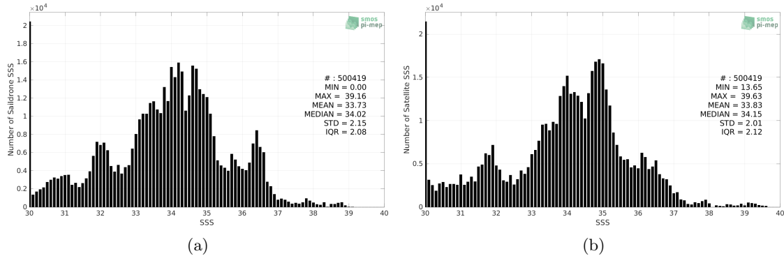
Figure 2: Histograms of SSS from Saildrone (a) and SMOS SSS L3 v332 - 9 Days (CATDS-CPDC) (b) considering all match-up pairs per bins of 0.1 over the Global Ocean Pi-MEP region and for the full satellite product period.
