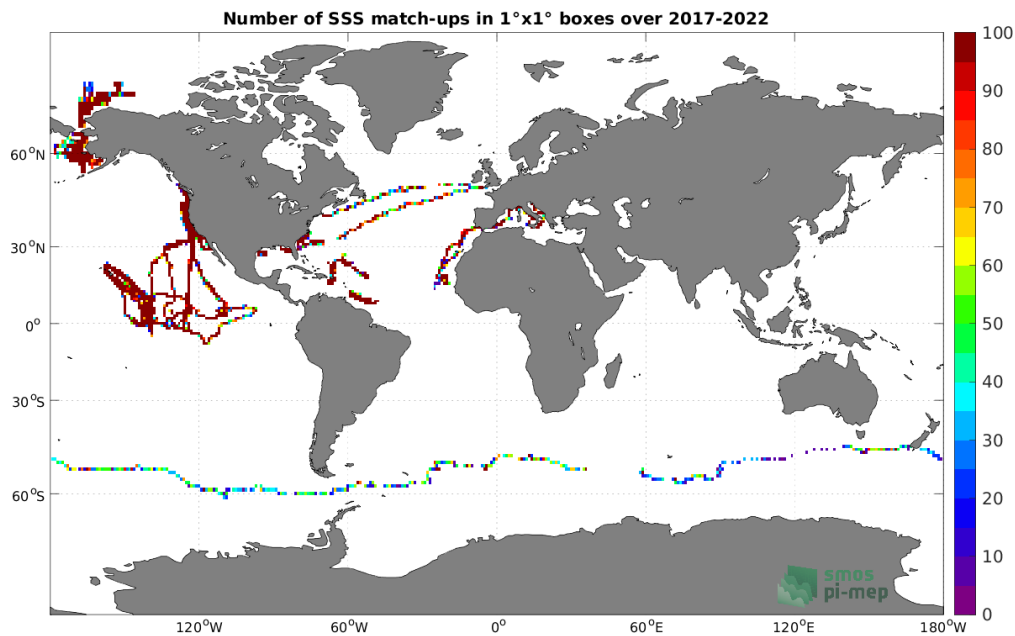
Figure 4: Number of SSS match-ups between Saildrone SSS and the SMOS SSS L3 v332 - 9 Days (CATDS-CPDC) SSS product for the Global Ocean Pi-MEP region over 1^\circ \times 1^\circ boxes and for the full satellite product period.
