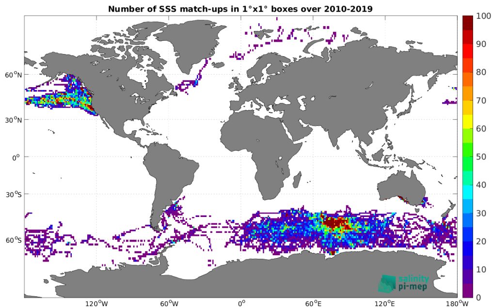
Figure 4: Number of SSS match-ups between Marine mammals SSS and the SMOS SSS L3 v332 - 9 Days (CATDS-CPDC) SSS product for the Global Ocean Pi-MEP region over 1^\circ \times 1^\circ boxes and for the full satellite product period.
