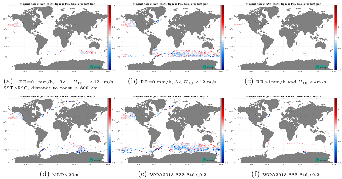
Figure 12: Temporal mean gridded over spatial boxes of size 1^\circ \times 1^\circ of \Delta SSS (SMOS SSS L3 v332 - 9 Days (CATDS-CPDC) - Marine mammals) for 6 different subdatasets corresponding to:RR=0 mm/h, 3 < U_{10} < 12 m/s, SST > 5^\circ\text{C} , distance to coast > 800 km (a), RR=0 mm/h, 3 < U_{10} < 12 m/s (b), RR > 1 mm/h and U_{10} < 4 m/s (c),MLD < 20 m (d),WOA2013 SSS Std < 0.2 (e),WOA2013 SSS Std > 0.2 (f).
