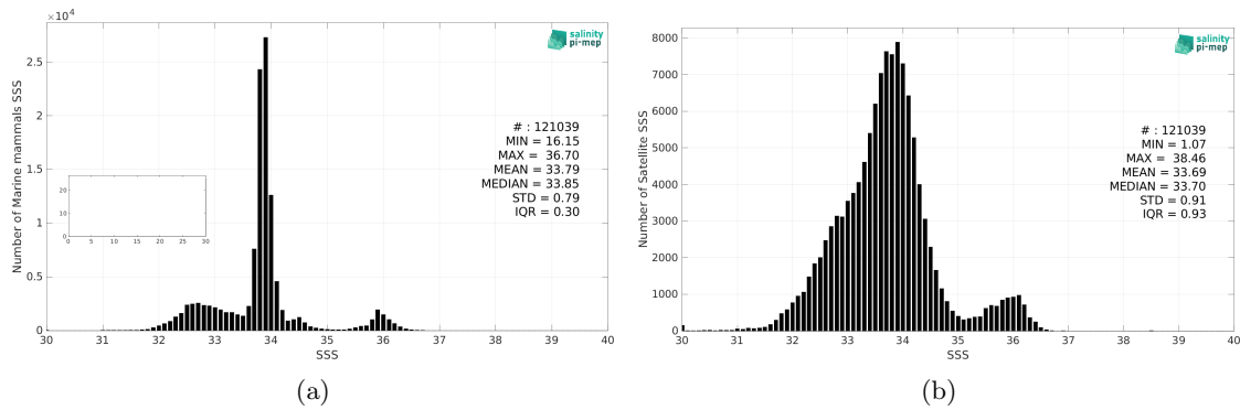
Figure 2: Histograms of SSS from Marine mammals (a) and SMOS SSS L3 v332 - 9 Days (CATDS-CPDC) (b) considering all match-up pairs per bins of 0.1 over the Global Ocean Pi-MEP region and for the full satellite product period.
