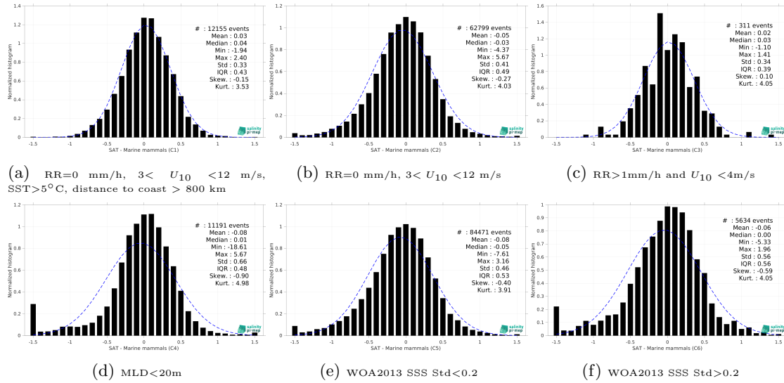
Figure 13: Normalized histogram of \Delta\text{SSS} (SMOS SSS L3 v332 - 9 Days (CATDS-CPDC) - Marine mammals) for 6 different subdatasets corresponding to: RR=0 mm/h, 3 < U_{10} < 12 m/s, SST>5°C, distance to coast > 800 km (a), RR=0 mm/h, 3 < U_{10} < 12 m/s (b), RR>1mm/h and U_{10} < 4 m/s (c), MLD<20m (d), WOA2013 SSS Std<0.2 (e), WOA2013 SSS Std>0.2 (f).
