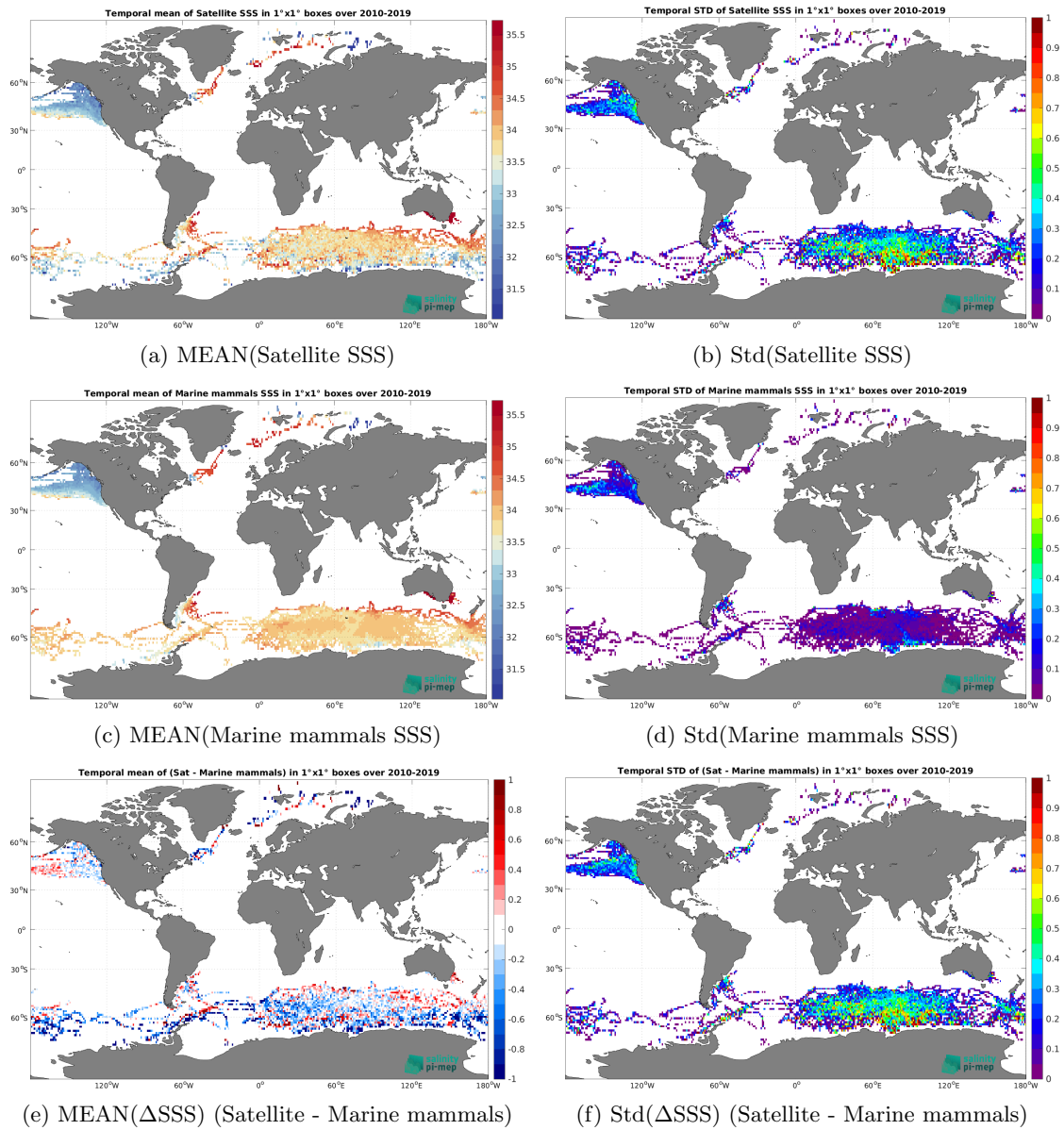
Figure 6: Temporal mean (left) and Std (right) of SSS from SMOS SSS L3 v332 - 9 Days (CATDS-CPDC) (top), Marine mammals (middle), and of \Delta SSS (Satellite - Marine mammals). Only match-up pairs are used to generate these maps.
