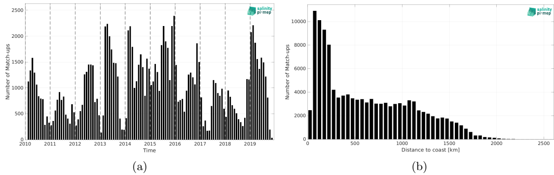
Figure 1: Number of match-ups between Marine mammals and SMOS SSS L3 v332 - 9 Days (CATDS-CPDC) SSS as a function of time (a) and as function of the distance to coast (b) over the Global Ocean Pi-MEP region and for the full satellite product period.
