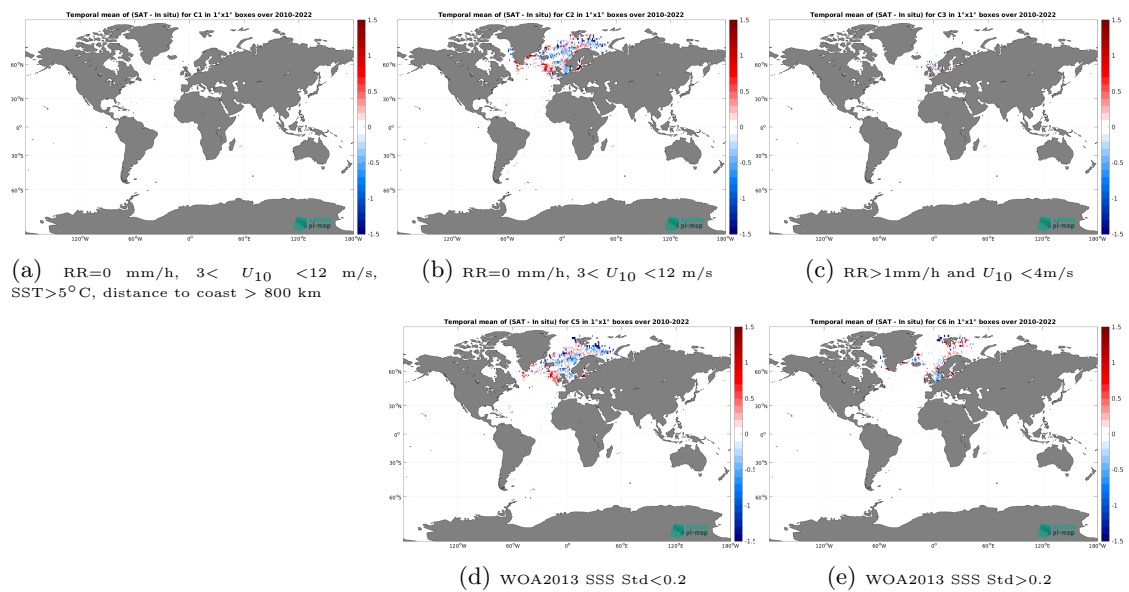
Figure 14: Temporal mean gridded over spatial boxes of size 1^\circ \times 1^\circ of \Delta SSS (SMOS SSS L3 v332 - 9 Days (CATDS-CPDC) - ICES) for 5 different subdatasets corresponding to:RR=0 mm/h, 3 < U_{10} < 12 m/s, SST > 5^\circ\text{C} , distance to coast > 800 km (a), RR=0 mm/h, 3 < U_{10} < 12 m/s (b), RR > 1 mm/h and U_{10} < 4 m/s (c), WOA2013 SSS Std < 0.2 (d), WOA2013 SSS Std > 0.2 (e).
