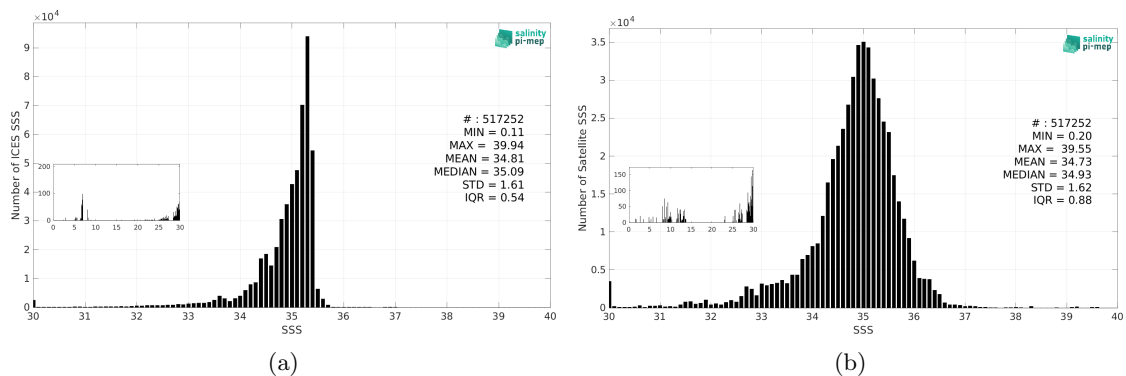
Figure 3: Histograms of SSS from ICES (a) and SMOS SSS L3 v332 - 9 Days (CATDS-CPDC) (b) considering all match-up pairs per bins of 0.1 over the Global Ocean Pi-MEP region and for the full satellite product period.
