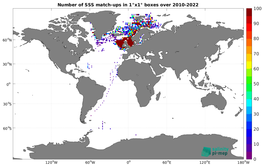
Figure 5: Number of SSS match-ups between ICES SSS and the SMOS SSS L3 v332 - 9 Days (CATDS-CPDC) SSS product for the Global Ocean Pi-MEP region over 1^\circ \times 1^\circ boxes and for the full satellite product period.
