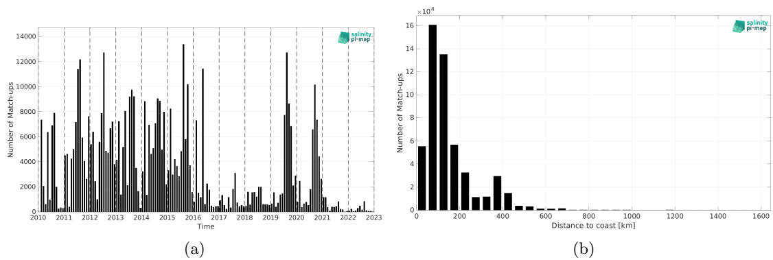
Figure 2: Number of match-ups between ICES and SMOS SSS L3 v332 - 9 Days (CATDS-CPDC) SSS as a function of time (a) and as function of the distance to coast (b) over the Global Ocean Pi-MEP region and for the full satellite product period.
