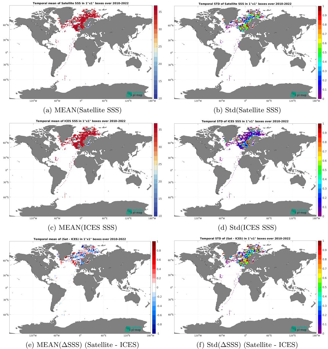
Figure 7: Temporal mean (left) and Std (right) of SSS from SMOS SSS L3 v332 - 9 Days (CATDS-CPDC) (top), ICES (middle), and of \Delta SSS (Satellite - ICES). Only match-up pairs are used to generate these maps.
