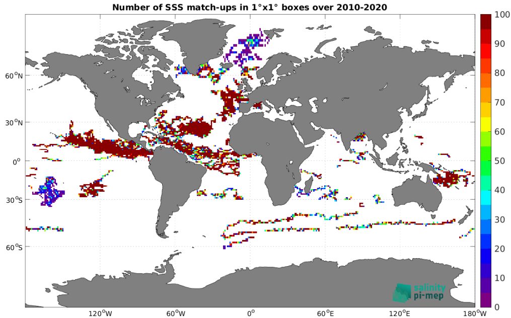
Figure 4: Number of SSS match-ups between Surface drifters SSS and the SMOS SSS L3 v332 - 9 Days (CATDS-CPDC) SSS product for the Global Ocean Pi-MEP region over 1^\circ \times 1^\circ boxes and for the full satellite product period.
