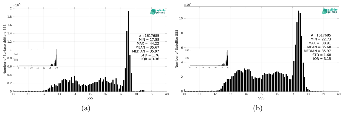
Figure 3: Histograms of SSS from Surface drifters (a) and SMOS SSS L3 v332 - 9 Days (CATDS-CPDC) (b) considering all match-up pairs per bins of 0.1 over the Global Ocean Pi-MEP region and for the full satellite product period.
