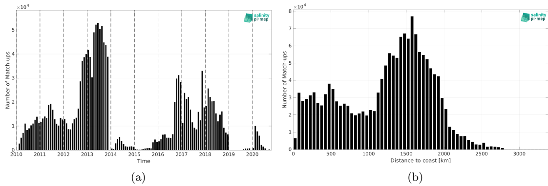
Figure 2: Number of match-ups between Surface drifters and SMOS SSS L3 v332 - 9 Days (CATDS-CPDC) SSS as a function of time (a) and as function of the distance to coast (b) over the Global Ocean Pi-MEP region and for the full satellite product period.
