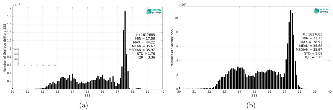
Figure 2: Histograms of SSS from Surface drifters (a) and SMOS SSS L3 v332 - 9 Days (CATDS-CPDC) (b) considering all match-up pairs per bins of 0.1 over the Global Ocean Pi-MEP region and for the full satellite product period.
