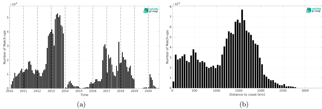
Figure 1: Number of match-ups between Surface drifters and SMOS SSS L3 v332 - 9 Days (CATDS-CPDC) SSS as a function of time (a) and as function of the distance to coast (b) over the Global Ocean Pi-MEP region and for the full satellite product period.
