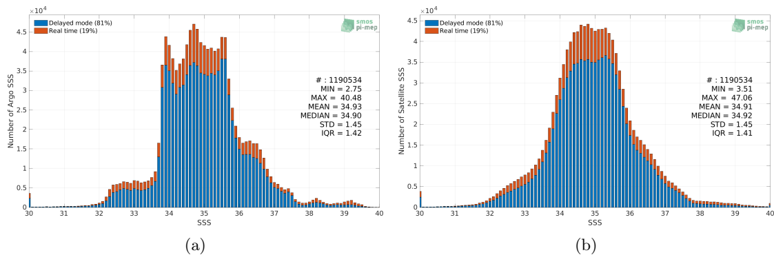
Figure 2: Histograms of SSS from Argo (a) and SMOS SSS L3 v332 - 9 Days (CATDS-CPDC) (b) considering all match-up pairs per bins of 0.1 over the Global Ocean Pi-MEP region and for the full satellite product period.
