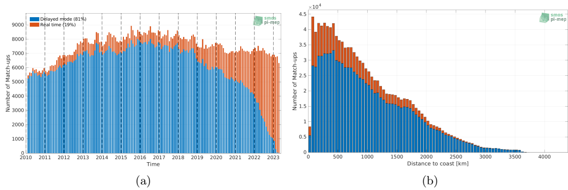
Figure 1: Number of match-ups between Argo and SMOS SSS L3 v332 - 9 Days (CATDS-CPDC) SSS as a function of time (a) and as function of the distance to coast (b) over the Global Ocean Pi-MEP region and for the full satellite product period.
