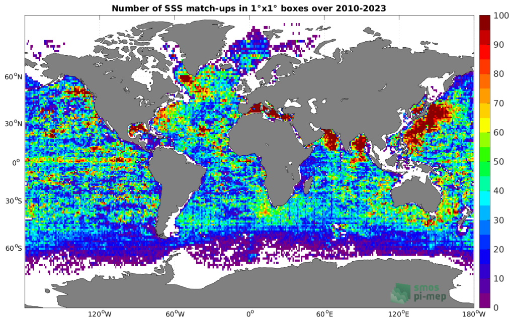
Figure 4: Number of SSS match-ups between Argo SSS and the SMOS SSS L3 v332 - 9 Days (CATDS-CPDC) SSS product for the Global Ocean Pi-MEP region over 1^\circ \times 1^\circ boxes and for the full satellite product period.
