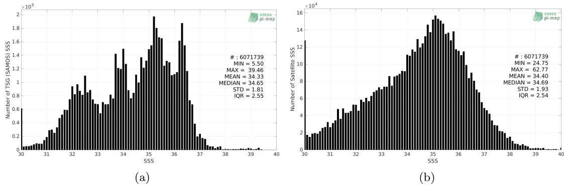
Figure 2: Histograms of SSS from TSG (SAMOS) (a) and SMOS SSS L2Q v331 - 0.25 Deg (CATDS-CPDC) (b) considering all match-up pairs per bins of 0.1 over the Global Ocean Pi-MEP region and for the full satellite product period.
