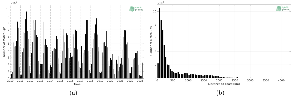
Figure 1: Number of match-ups between TSG (SAMOS) and SMOS SSS L2Q v331 - 0.25 Deg (CATDS-CPDC) SSS as a function of time (a) and as function of the distance to coast (b) over the Global Ocean Pi-MEP region and for the full satellite product period.
