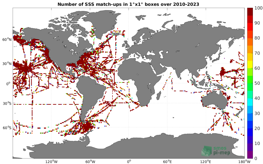
Figure 4: Number of SSS match-ups between TSG (SAMOS) SSS and the SMOS SSS L2Q v331 - 0.25 Deg (CATDS-CPDC) SSS product for the Global Ocean Pi-MEP region over 1^\circ \times 1^\circ boxes and for the full satellite product period.
