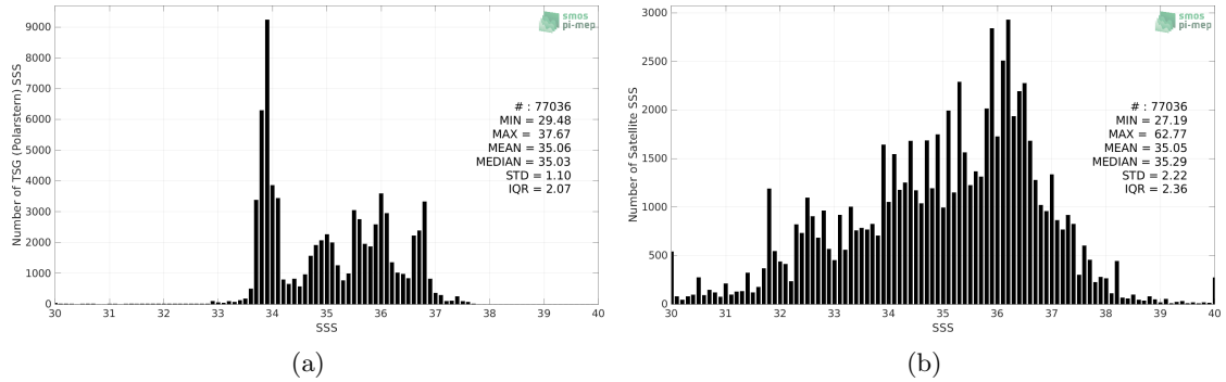
Figure 2: Histograms of SSS from TSG (Polarstern) (a) and SMOS SSS L2Q v331 - 0.25 Deg (CATDS-CPDC) (b) considering all match-up pairs per bins of 0.1 over the Global Ocean Pi-MEP region and for the full satellite product period.
