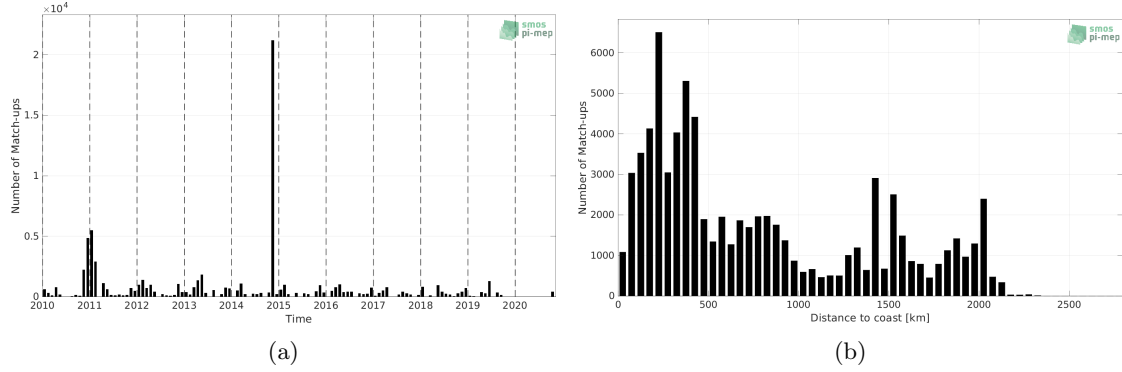
Figure 1: Number of match-ups between TSG (Polarstern) and SMOS SSS L2Q v331 - 0.25 Deg (CATDS-CPDC) SSS as a function of time (a) and as function of the distance to coast (b) over the Global Ocean Pi-MEP region and for the full satellite product period.
