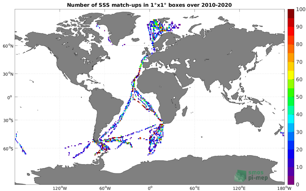
Figure 4: Number of SSS match-ups between TSG (Polarstern) SSS and the SMOS SSS L2Q v331 - 0.25 Deg (CATDS-CPDC) SSS product for the Global Ocean Pi-MEP region over 1^\circ \times 1^\circ boxes and for the full satellite product period.
