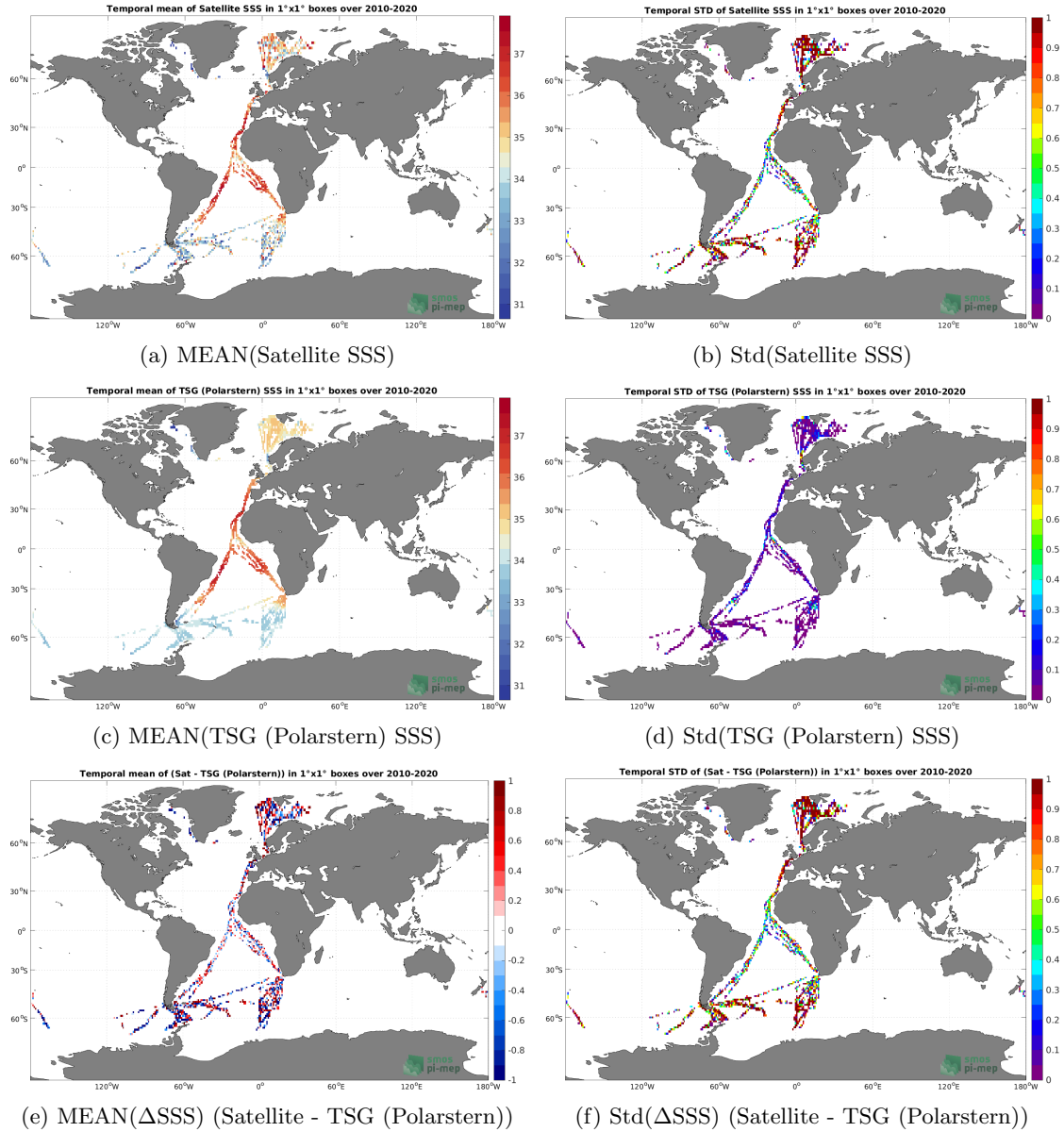
Figure 6: Temporal mean (left) and Std (right) of SSS from SMOS SSS L2Q v331 - 0.25 Deg (CATDS-CPDC) (top), TSG (Polarstern) (middle), and of \Delta SSS (Satellite - TSG (Polarstern)). Only match-up pairs are used to generate these maps.
