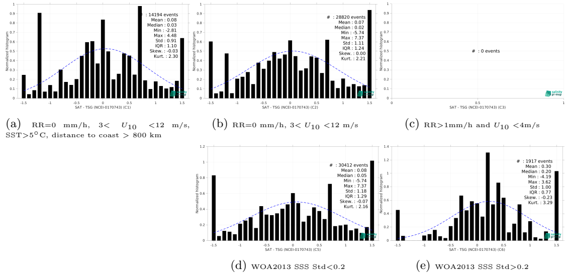
Figure 13: Normalized histogram of \Delta SSS (SMOS SSS L2Q v331 - 0.25 Deg (CATDS-CPDC) - TSG (NCEI-0170743)) for 5 different subdatasets corresponding to: RR=0 mm/h, 3 < U_{10} < 12 m/s, SST > 5°C, distance to coast > 800 km (a), RR=0 mm/h, 3 < U_{10} < 12 m/s (b), RR > 1mm/h and U_{10} < 4 m/s (c), WOA2013 SSS Std < 0.2 (d), WOA2013 SSS Std > 0.2 (e).
