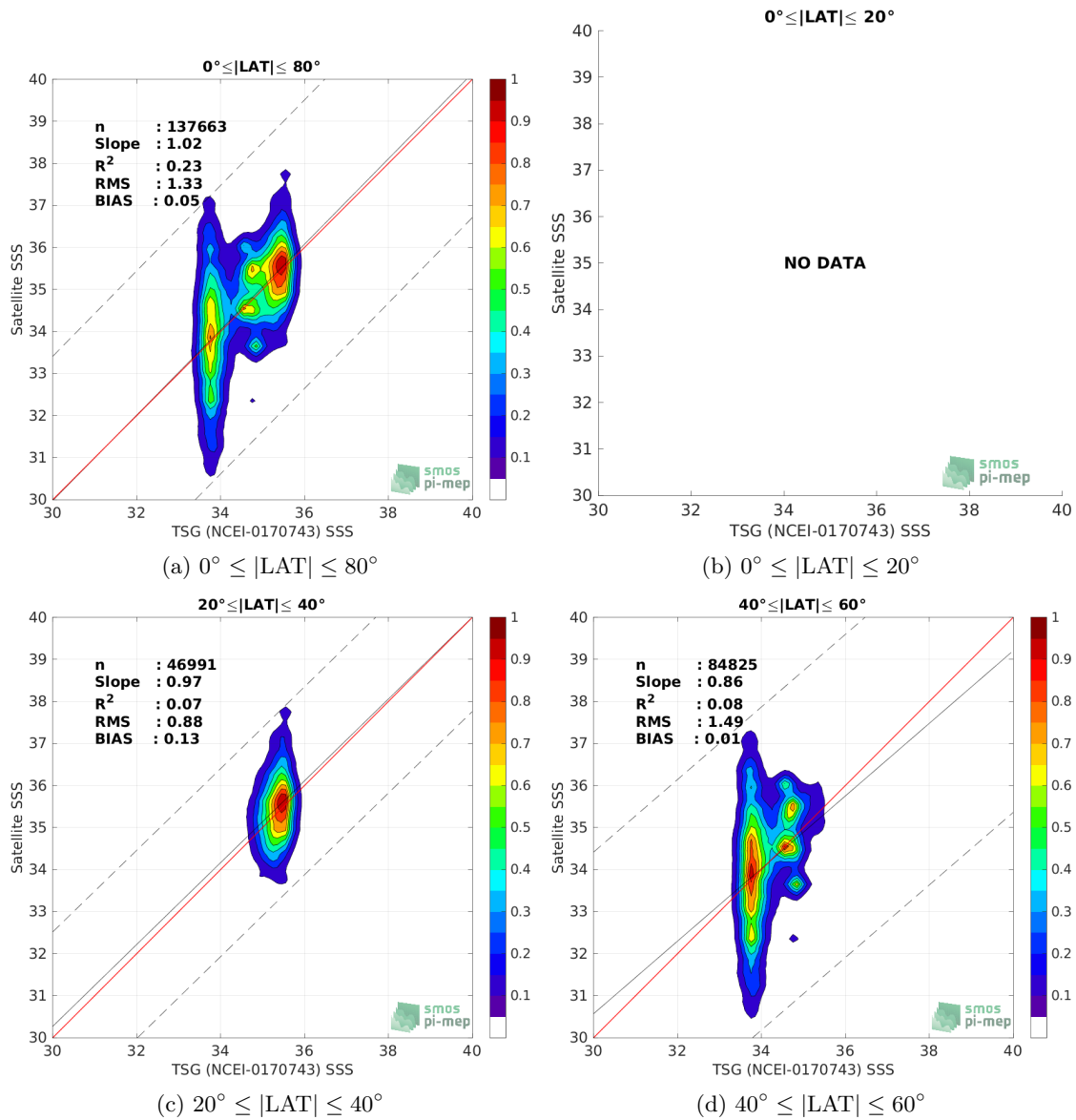
Figure 9: Contour maps of the concentration of SMOS SSS L2Q v331 - 0.25 Deg (CATDS-CPDC) SSS (y-axis) versus TSG (NCEI-0170743) SSS (x-axis) at match-up pairs for different latitude bands. For each plot, the red line shows x=y . The black thin and dashed lines indicate a linear fit through the data cloud and the \pm 95\% confidence levels, respectively. The number match-up pairs n , the slope and R^2 coefficient of the linear fit, the root mean square (RMS) and the mean bias between satellite and in situ data are indicated for each latitude band in each plots.
