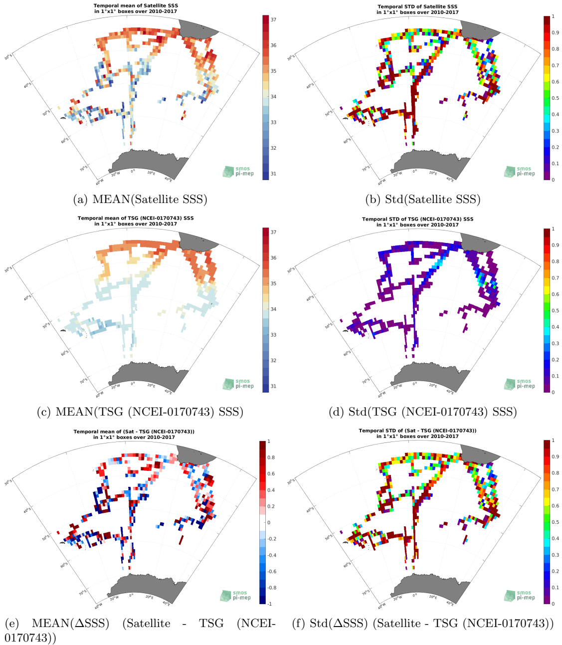
Figure 6: Temporal mean (left) and Std (right) of SSS from SMOS SSS L2Q v331 - 0.25 Deg (CATDS-CPDC) (top), TSG (NCEI-0170743) (middle), and of \Delta SSS (Satellite - TSG (NCEI-0170743)). Only match-up pairs are used to generate these maps.
