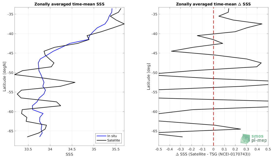
Figure 8: Left panel: Zonal mean SSS from SMOS SSS L2Q v331 - 0.25 Deg (CATDS-CPDC) satellite product (black) and from TSG (NCEI-0170743) (blue). Right panel: Zonal mean of \Delta SSS (Satellite - TSG (NCEI-0170743)) for all the collected Pi-MEP match-up pairs estimated over the full satellite product period.
