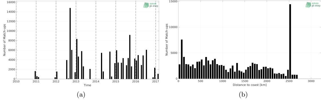
Figure 1: Number of match-ups between TSG (NCEI-0170743) and SMOS SSS L2Q v331 - 0.25 Deg (CATDS-CPDC) SSS as a function of time (a) and as function of the distance to coast (b) over the Global Ocean Pi-MEP region and for the full satellite product period.
