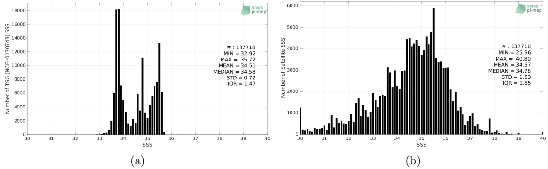
Figure 2: Histograms of SSS from TSG (NCEI-0170743) (a) and SMOS SSS L2Q v331 - 0.25 Deg (CATDS-CPDC) (b) considering all match-up pairs per bins of 0.1 over the Global Ocean Pi-MEP region and for the full satellite product period.
