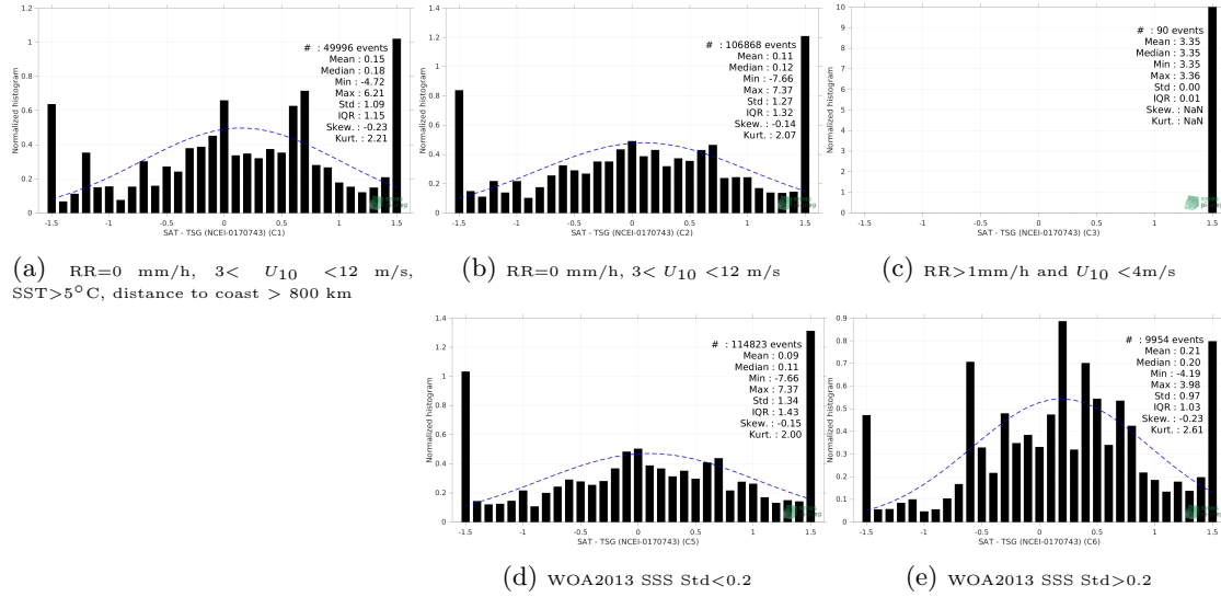
Figure 13: Normalized histogram of \Delta SSS (SMOS SSS L2Q v331 - 0.25 Deg (CATDS-CPDC) - TSG (NCEI-0170743)) for 5 different subdatasets corresponding to: RR=0 mm/h, 3 < U_{10} < 12 m/s, SST>5°C, distance to coast > 800 km (a), RR=0 mm/h, 3 < U_{10} < 12 m/s (b), RR>1mm/h and U_{10} < 4 m/s (c), WOA2013 SSS Std<0.2 (d), WOA2013 SSS Std>0.2 (e).
