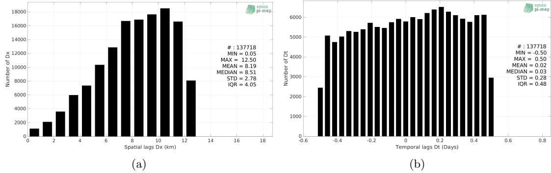
Figure 5: Histograms of the spatial (a) and temporal (b) lags between the location/time of the TSG (NCEI-0170743) measurement and the date of the corresponding SMOS SSS L2Q v331 - 0.25 Deg (CATDS-CPDC) SSS pixel.
