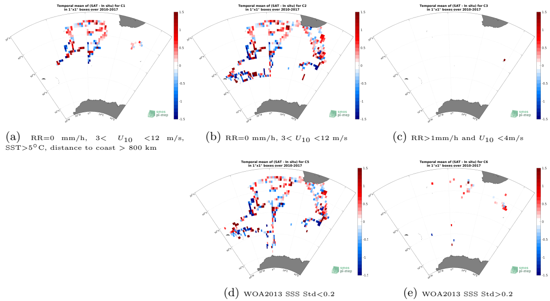
Figure 12: Temporal mean gridded over spatial boxes of size 1^\circ \times 1^\circ of \Delta SSS (SMOS SSS L2Q v331 - 0.25 Deg (CATDS-CPDC) - TSG (NCEI-0170743)) for 5 different subdatasets corresponding to:RR=0 mm/h, 3 < U_{10} < 12 m/s, SST >5^\circ C, distance to coast > 800 km (a), RR=0 mm/h, 3 < U_{10} < 12 m/s (b), RR >1 mm/h and U_{10} < 4 m/s (c), WOA2013 SSS Std <0.2 (d), WOA2013 SSS Std >0.2 (e).
