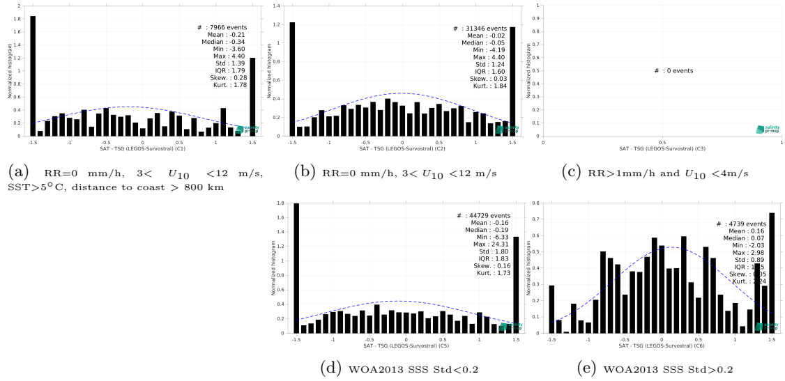
Figure 13: Normalized histogram of \Delta SSS (SMOS SSS L2Q v331 - 0.25 Deg (CATDS-CPDC) - TSG (LEGOS-Survostral)) for 5 different subdatasets corresponding to: RR=0 mm/h, 3 < U_{10} < 12 m/s, SST > 5°C, distance to coast > 800 km (a), RR=0 mm/h, 3 < U_{10} < 12 m/s (b), RR > 1mm/h and U_{10} < 4 m/s (c), WOA2013 SSS Std < 0.2 (d), WOA2013 SSS Std > 0.2 (e).
