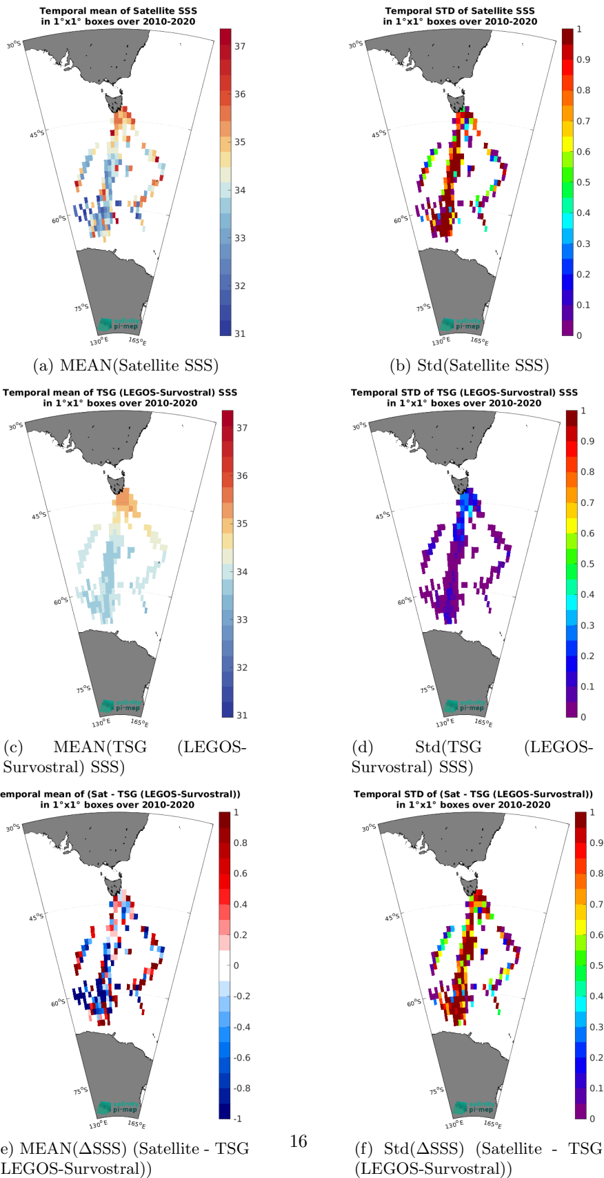
Figure 6: Temporal mean (left) and Std (right) of SSS from SMOS SSS L2Q v331 - 0.25 Deg (CATDS-CPDC) (top), TSG (LEGOS-Survostral) (middle), and of \Delta SSS (Satellite - TSG (LEGOS-Survostral)). Only match-up pairs are used to generate these maps.
