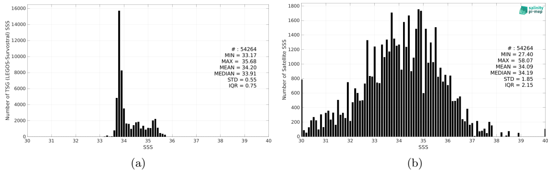
Figure 2: Histograms of SSS from TSG (LEGOS-Survostral) (a) and SMOS SSS L2Q v331 - 0.25 Deg (CATDS-CPDC) (b) considering all match-up pairs per bins of 0.1 over the Global Ocean Pi-MEP region and for the full satellite product period.
