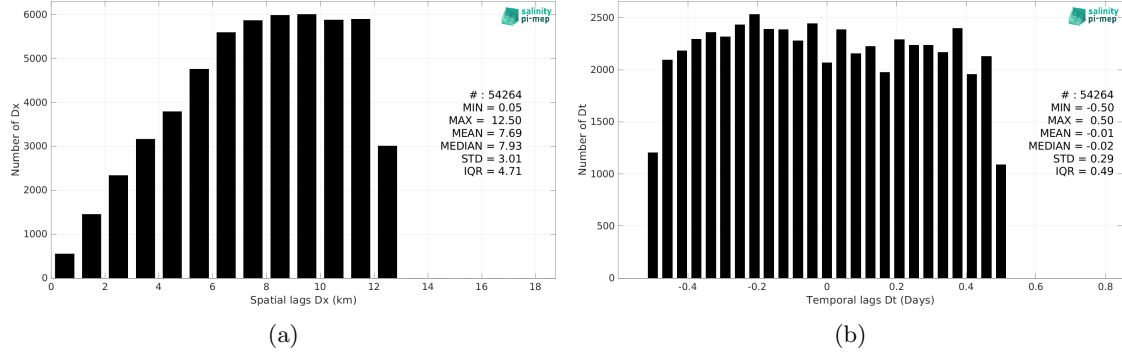
Figure 5: Histograms of the spatial (a) and temporal (b) lags between the location/time of the TSG (LEGOS-Survostral) measurement and the date of the corresponding SMOS SSS L2Q v331 - 0.25 Deg (CATDS-CPDC) SSS pixel.
