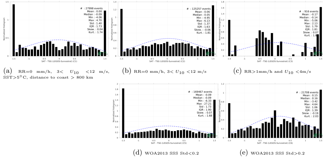
Figure 13: Normalized histogram of \Delta SSS (SMOS SSS L2Q v331 - 0.25 Deg (CATDS-CPDC) - TSG (LEGOS-Survostral)) for 5 different subdatasets corresponding to: RR=0 mm/h, 3 < U_{10} < 12 m/s, SST>5°C, distance to coast > 800 km (a), RR=0 mm/h, 3 < U_{10} < 12 m/s (b), RR>1mm/h and U_{10} < 4 m/s (c), WOA2013 SSS Std<0.2 (d), WOA2013 SSS Std>0.2 (e).
