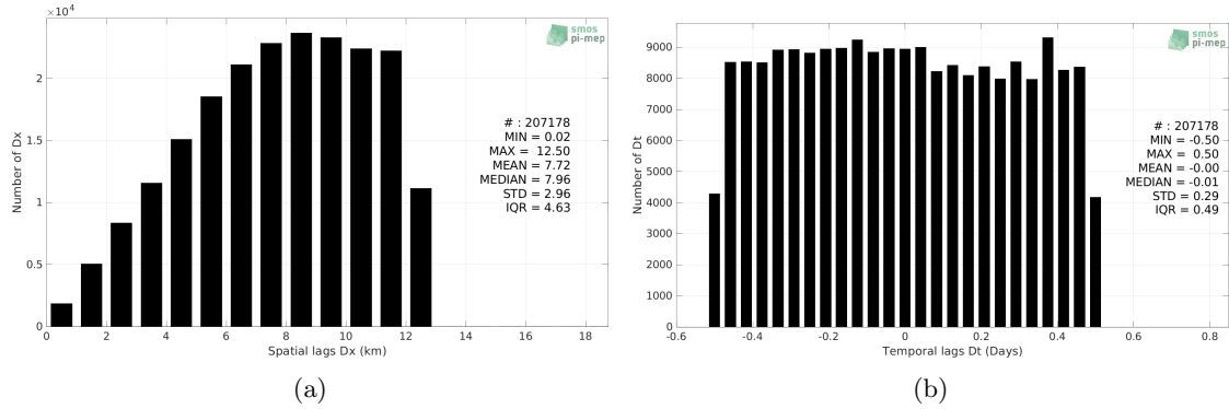
Figure 5: Histograms of the spatial (a) and temporal (b) lags between the location/time of the TSG (LEGOS-Survostral) measurement and the date of the corresponding SMOS SSS L2Q v331 - 0.25 Deg (CATDS-CPDC) SSS pixel.
