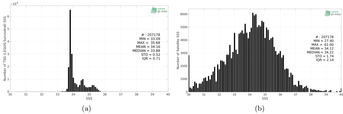
Figure 2: Histograms of SSS from TSG (LEGOS-Survostral) (a) and SMOS SSS L2Q v331 - 0.25 Deg (CATDS-CPDC) (b) considering all match-up pairs per bins of 0.1 over the Global Ocean Pi-MEP region and for the full satellite product period.
