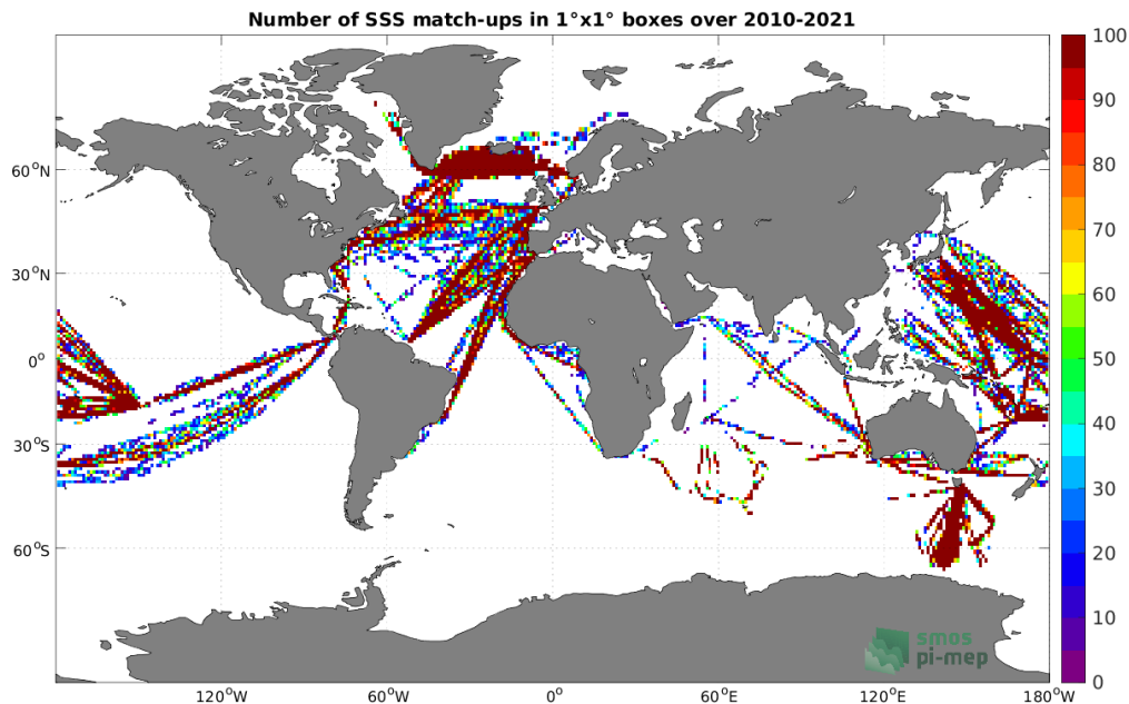
Figure 4: Number of SSS match-ups between TSG (LEGOS-DM) SSS and the SMOS SSS L2Q v331 - 0.25 Deg (CATDS-CPDC) SSS product for the Global Ocean Pi-MEP region over 1^\circ \times 1^\circ boxes and for the full satellite product period.
