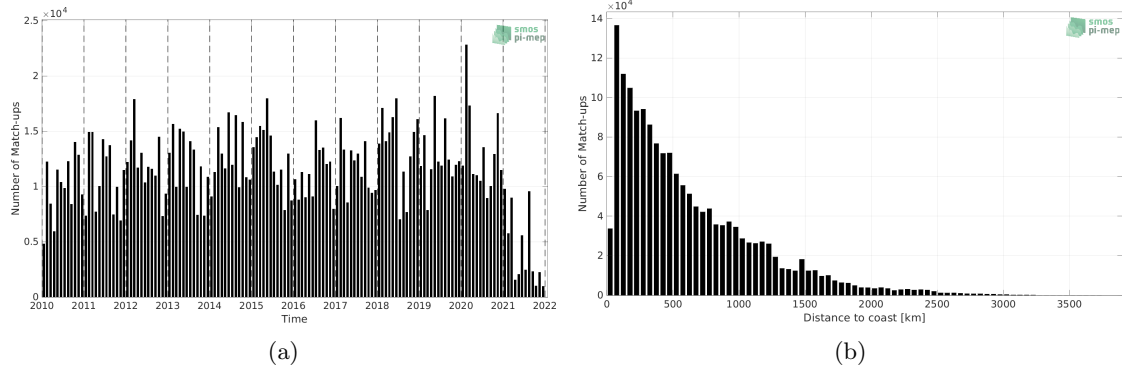
Figure 1: Number of match-ups between TSG (LEGOS-DM) and SMOS SSS L2Q v331 - 0.25 Deg (CATDS-CPDC) SSS as a function of time (a) and as function of the distance to coast (b) over the Global Ocean Pi-MEP region and for the full satellite product period.
