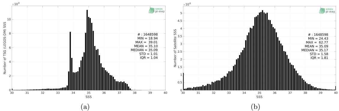
Figure 2: Histograms of SSS from TSG (LEGOS-DM) (a) and SMOS SSS L2Q v331 - 0.25 Deg (CATDS-CPDC) (b) considering all match-up pairs per bins of 0.1 over the Global Ocean Pi-MEP region and for the full satellite product period.
