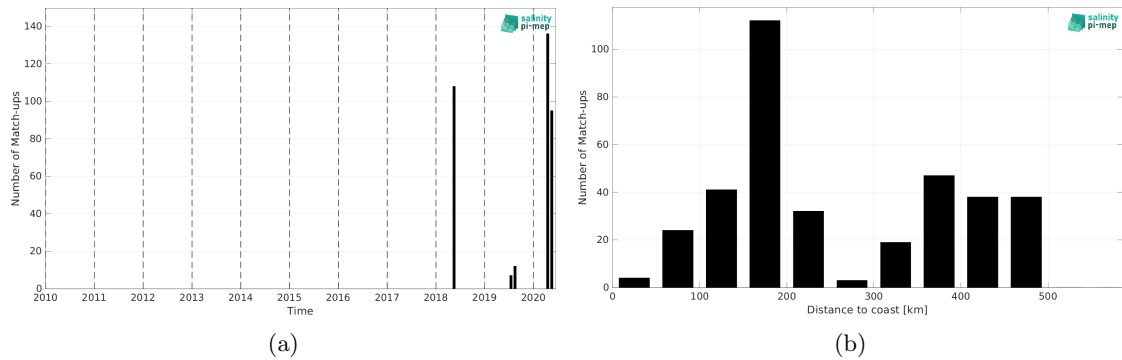
Figure 1: Number of match-ups between TSG (Lauge-Koch) and SMOS SSS L2Q v331 - 0.25 Deg (CATDS-CPDC) SSS as a function of time (a) and as function of the distance to coast (b) over the Global Ocean Pi-MEP region and for the full satellite product period.
