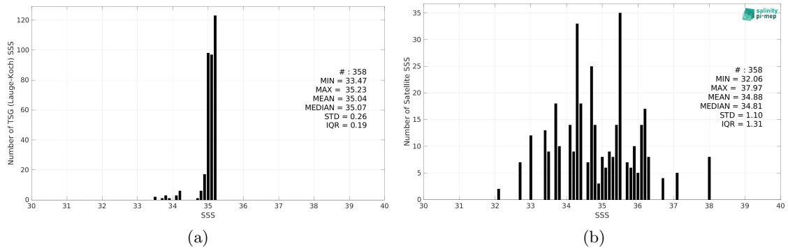
Figure 2: Histograms of SSS from TSG (Lauge-Koch) (a) and SMOS SSS L2Q v331 - 0.25 Deg (CATDS-CPDC) (b) considering all match-up pairs per bins of 0.1 over the Global Ocean Pi-MEP region and for the full satellite product period.
