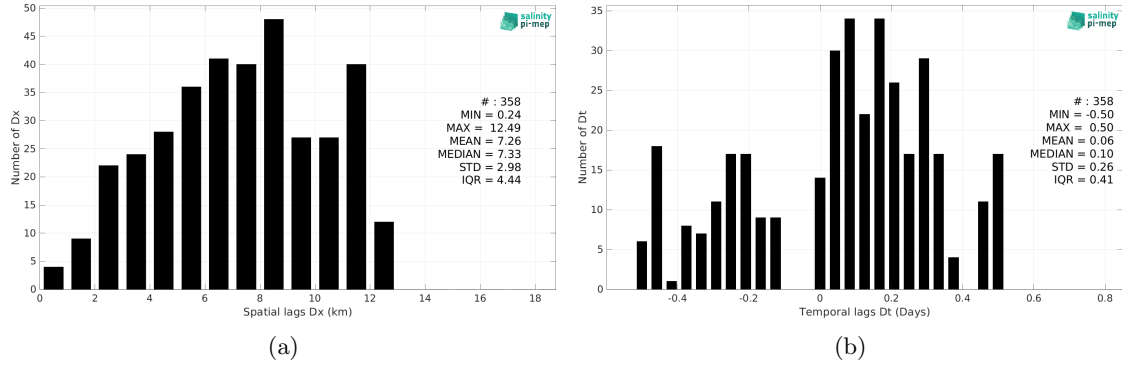
Figure 5: Histograms of the spatial (a) and temporal (b) lags between the location/time of the TSG (Lauge-Koch) measurement and the date of the corresponding SMOS SSS L2Q v331 - 0.25 Deg (CATDS-CPDC) SSS pixel.
