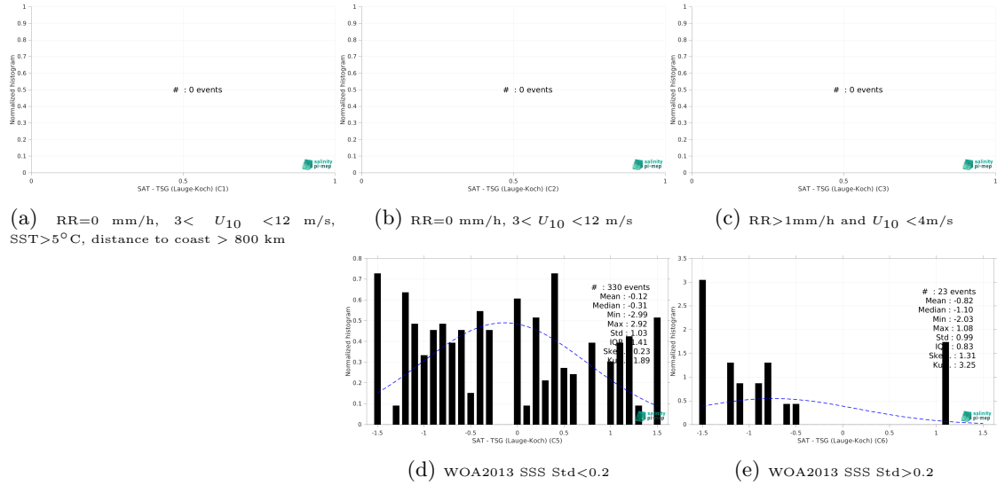
Figure 13: Normalized histogram of \Delta SSS (SMOS SSS L2Q v331 - 0.25 Deg (CATDS-CPDC) - TSG (Lauge-Koch)) for 5 different subdatasets corresponding to: RR=0 mm/h, 3 < U_{10} < 12 m/s, SST>5°C, distance to coast > 800 km (a), RR=0 mm/h, 3 < U_{10} < 12 m/s (b), RR>1mm/h and U_{10} < 4 m/s (c), WOA2013 SSS Std<0.2 (d), WOA2013 SSS Std>0.2 (e).
