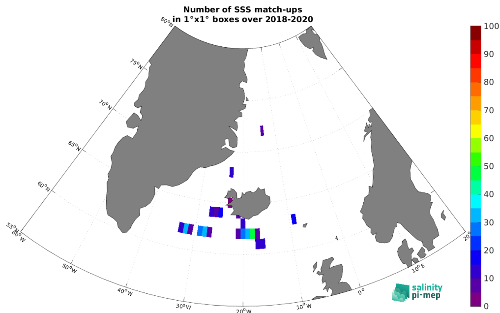
Figure 4: Number of SSS match-ups between TSG (Lauge-Koch) SSS and the SMOS SSS L2Q v331 - 0.25 Deg (CATDS-CPDC) SSS product for the Global Ocean Pi-MEP region over 1^\circ \times 1^\circ boxes and for the full satellite product period.
