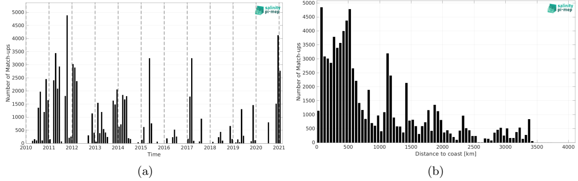
Figure 1: Number of match-ups between TSG (GOSUD-Sailing-ship) and SMOS SSS L2Q v331 - 0.25 Deg (CATDS-CPDC) SSS as a function of time (a) and as function of the distance to coast (b) over the Global Ocean Pi-MEP region and for the full satellite product period.
