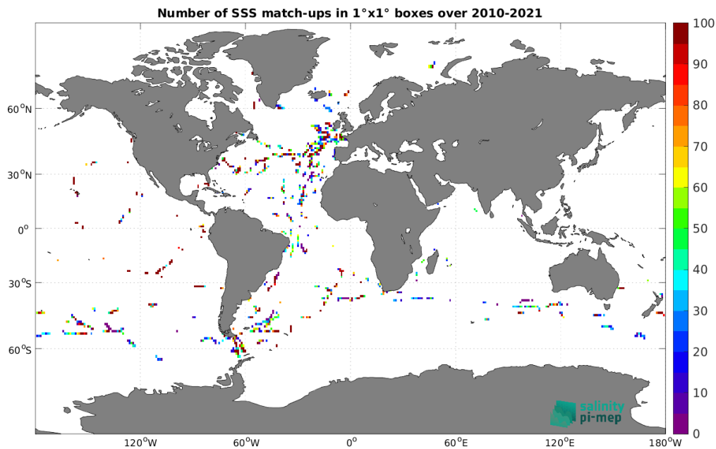
Figure 4: Number of SSS match-ups between TSG (GOSUD-Sailing-ship) SSS and the SMOS SSS L2Q v331 - 0.25 Deg (CATDS-CPDC) SSS product for the Global Ocean Pi-MEP region over 1^\circ \times 1^\circ boxes and for the full satellite product period.
