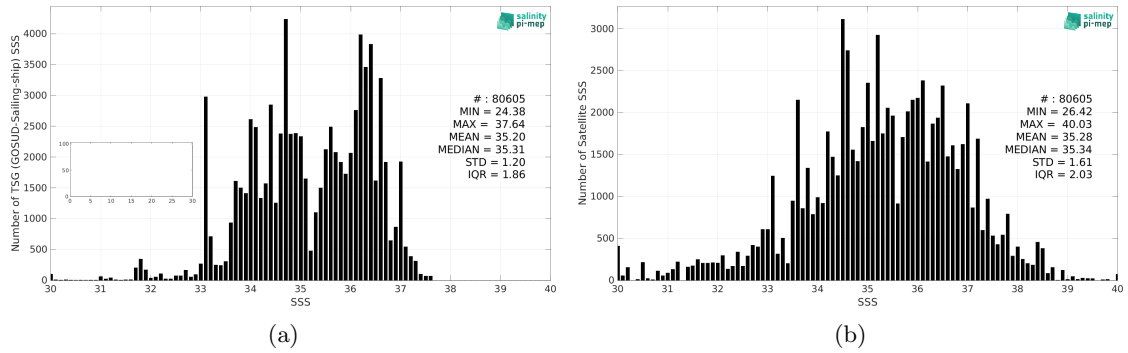
Figure 2: Histograms of SSS from TSG (GOSUD-Sailing-ship) (a) and SMOS SSS L2Q v331 - 0.25 Deg (CATDS-CPDC) (b) considering all match-up pairs per bins of 0.1 over the Global Ocean Pi-MEP region and for the full satellite product period.
