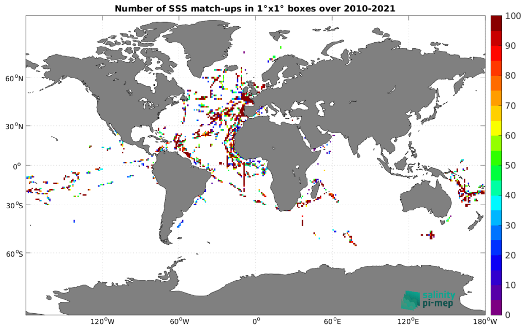
Figure 4: Number of SSS match-ups between TSG (GOSUD-Research-vessel) SSS and the SMOS SSS L2Q v331 - 0.25 Deg (CATDS-CPDC) SSS product for the Global Ocean Pi-MEP region over 1^\circ \times 1^\circ boxes and for the full satellite product period.
