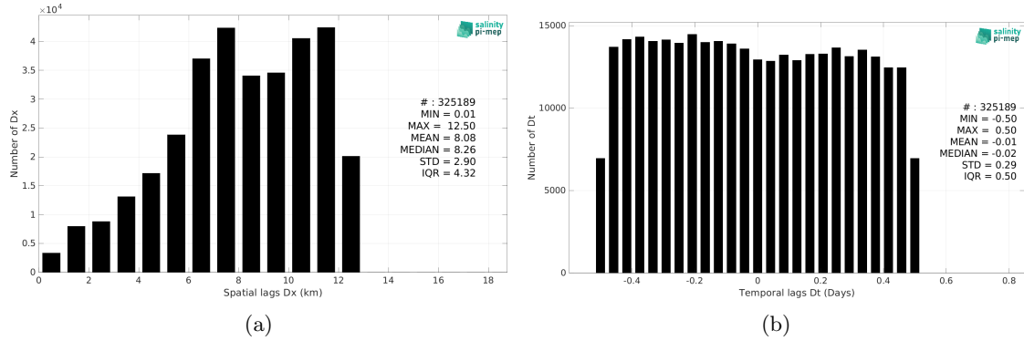
Figure 5: Histograms of the spatial (a) and temporal (b) lags between the location/time of the TSG (GOSUD-Research-vessel) measurement and the date of the corresponding SMOS SSS L2Q v331 - 0.25 Deg (CATDS-CPDC) SSS pixel.
