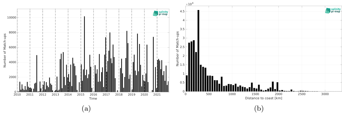
Figure 1: Number of match-ups between TSG (GOSUD-Research-vessel) and SMOS SSS L2Q v331 - 0.25 Deg (CATDS-CPDC) SSS as a function of time (a) and as function of the distance to coast (b) over the Global Ocean Pi-MEP region and for the full satellite product period.
