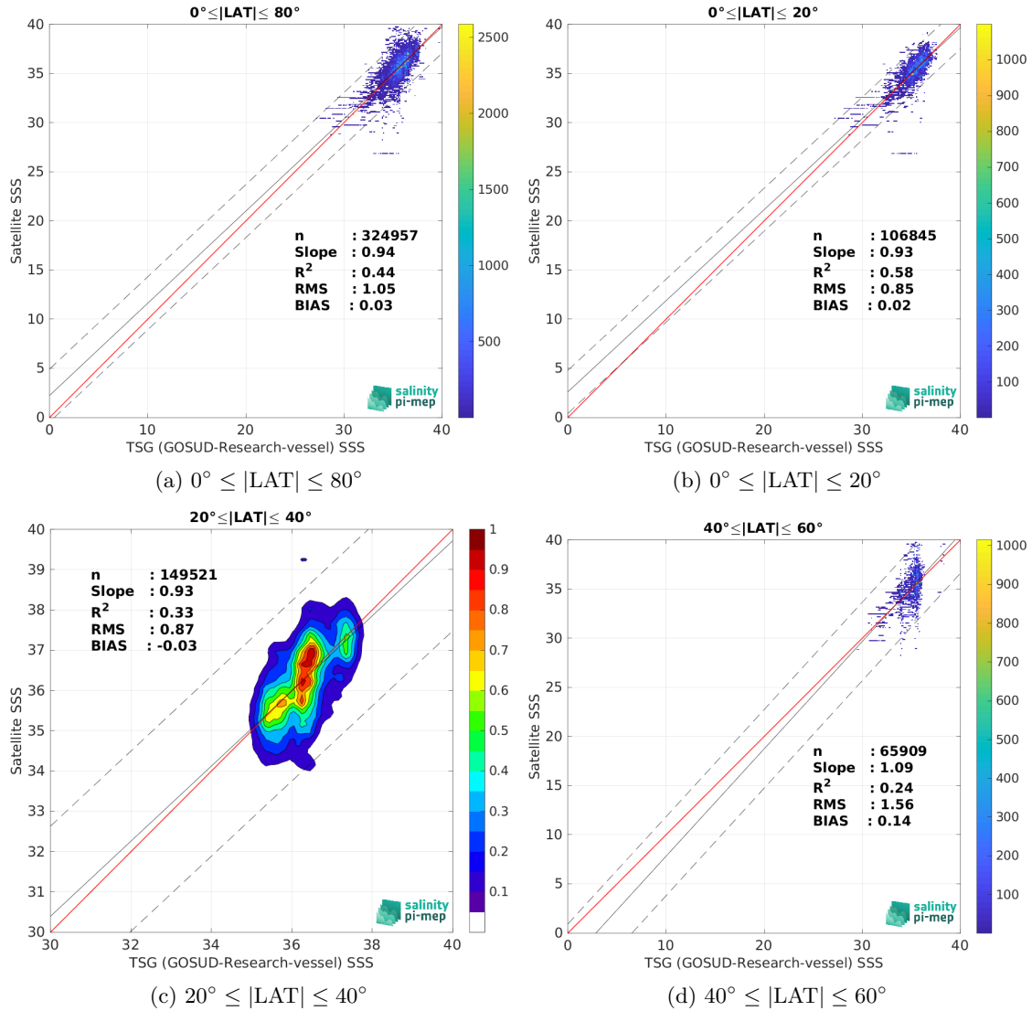
Figure 9: Contour maps of the concentration of SMOS SSS L2Q v331 - 0.25 Deg (CATDS-CPDC) SSS (y-axis) versus TSG (GOSUD-Research-vessel) SSS (x-axis) at match-up pairs for different latitude bands. For each plot, the red line shows x=y . The black thin and dashed lines indicate a linear fit through the data cloud and the \pm 95\% confidence levels, respectively. The number match-up pairs n , the slope and R^2 coefficient of the linear fit, the root mean square (RMS) and the mean bias between satellite and in situ data are indicated for each latitude band in each plots.
