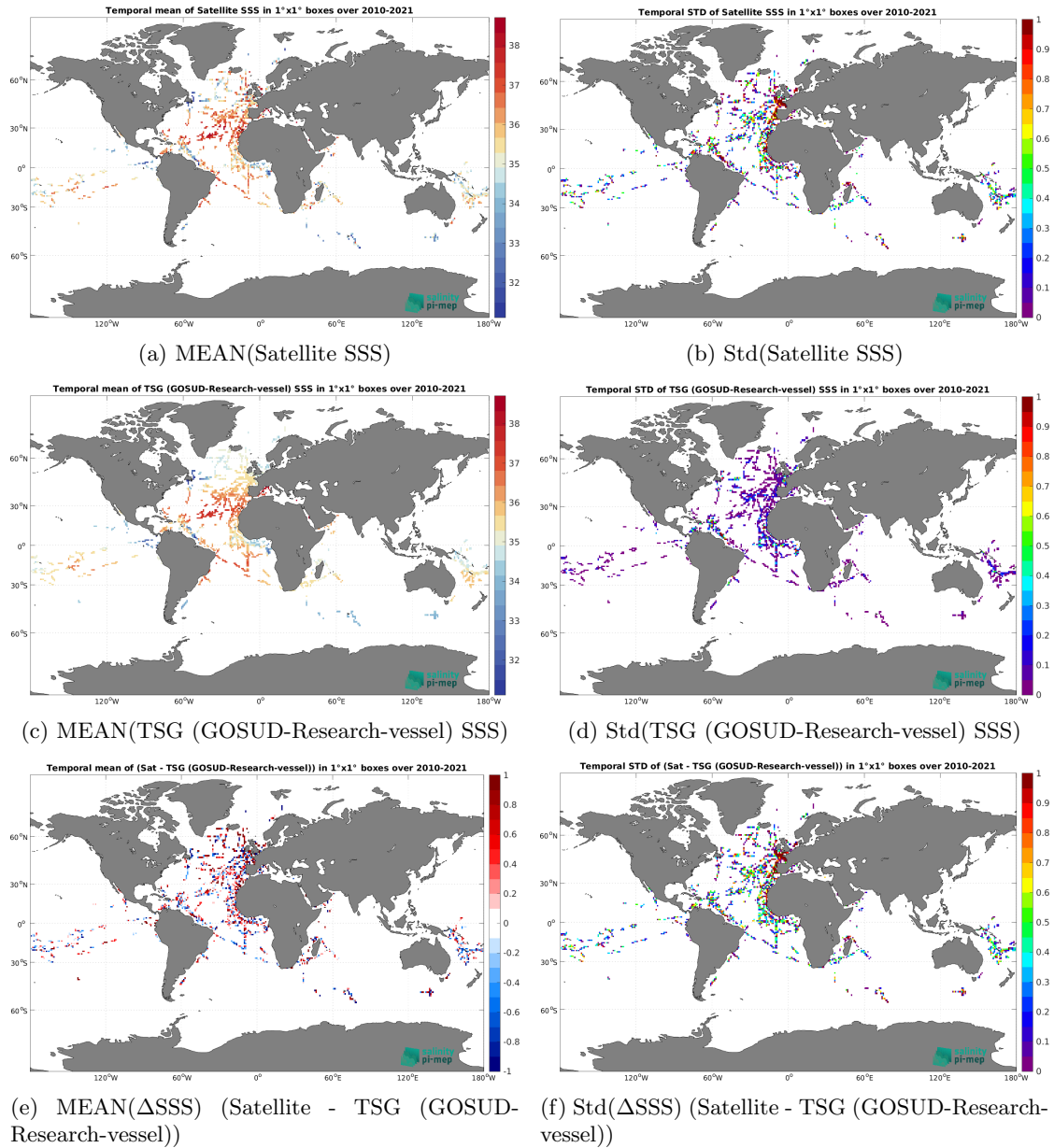
Figure 6: Temporal mean (left) and Std (right) of SSS from SMOS SSS L2Q v331 - 0.25 Deg (CATDS-CPDC) (top), TSG (GOSUD-Research-vessel) (middle), and of \Delta SSS (Satellite - TSG (GOSUD-Research-vessel)). Only match-up pairs are used to generate these maps.
