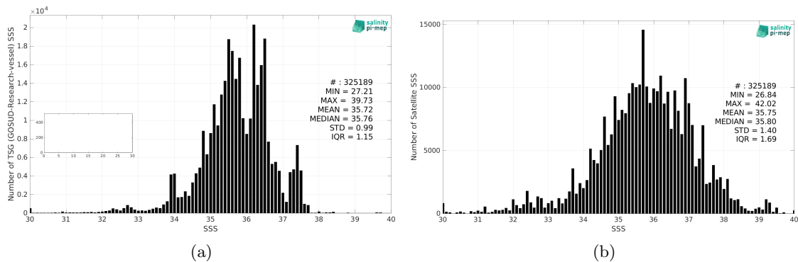
Figure 2: Histograms of SSS from TSG (GOSUD-Research-vessel) (a) and SMOS SSS L2Q v331 - 0.25 Deg (CATDS-CPDC) (b) considering all match-up pairs per bins of 0.1 over the Global Ocean Pi-MEP region and for the full satellite product period.
