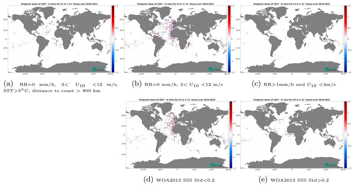
Figure 12: Temporal mean gridded over spatial boxes of size 1^\circ \times 1^\circ of \Delta SSS (SMOS SSS L2Q v331 - 0.25 Deg (CATDS-CPDC) - TSG (GOSUD-Research-vessel)) for 5 different subdatasets corresponding to:RR=0 mm/h, 3 < U_{10} < 12 m/s, SST > 5^\circ\text{C} , distance to coast > 800 km (a), RR=0 mm/h, 3 < U_{10} < 12 m/s (b), RR > 1 mm/h and U_{10} < 4 m/s (c), WOA2013 SSS Std < 0.2 (d), WOA2013 SSS Std > 0.2 (e).
