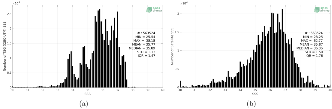
Figure 2: Histograms of SSS from TSG (CSIC-UTM) (a) and SMOS SSS L2Q v331 - 0.25 Deg (CATDS-CPDC) (b) considering all match-up pairs per bins of 0.1 over the Global Ocean Pi-MEP region and for the full satellite product period.
