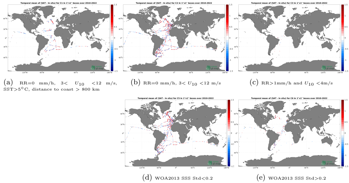
Figure 12: Temporal mean gridded over spatial boxes of size 1^\circ \times 1^\circ of \Delta SSS (SMOS SSS L2Q v331 - 0.25 Deg (CATDS-CPDC) - TSG (CSIC-UTM)) for 5 different subdatasets corresponding to:RR=0 mm/h, 3 < U_{10} < 12 m/s, SST > 5^\circ\text{C} , distance to coast > 800 km (a), RR=0 mm/h, 3 < U_{10} < 12 m/s (b), RR > 1 mm/h and U_{10} < 4 m/s (c), WOA2013 SSS Std < 0.2 (d), WOA2013 SSS Std > 0.2 (e).
