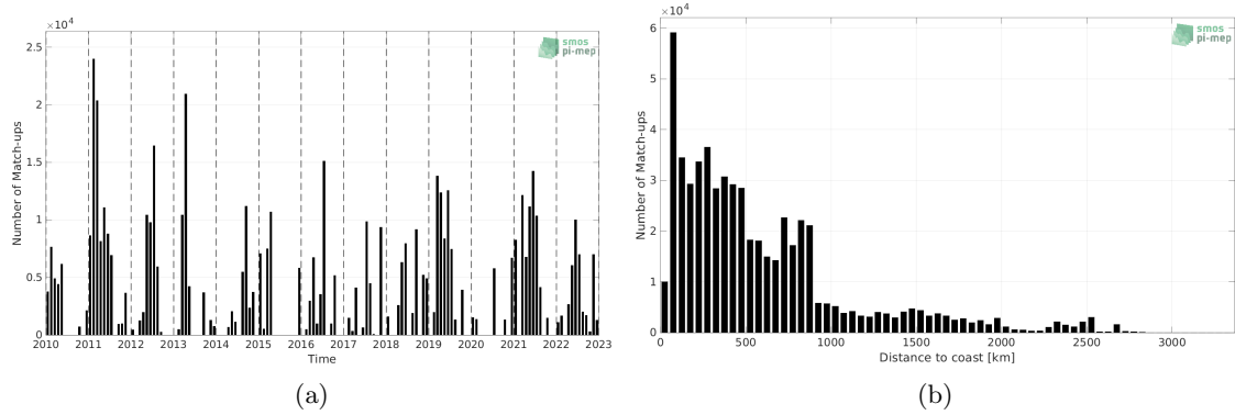
Figure 1: Number of match-ups between TSG (CSIC-UTM) and SMOS SSS L2Q v331 - 0.25 Deg (CATDS-CPDC) SSS as a function of time (a) and as function of the distance to coast (b) over the Global Ocean Pi-MEP region and for the full satellite product period.
