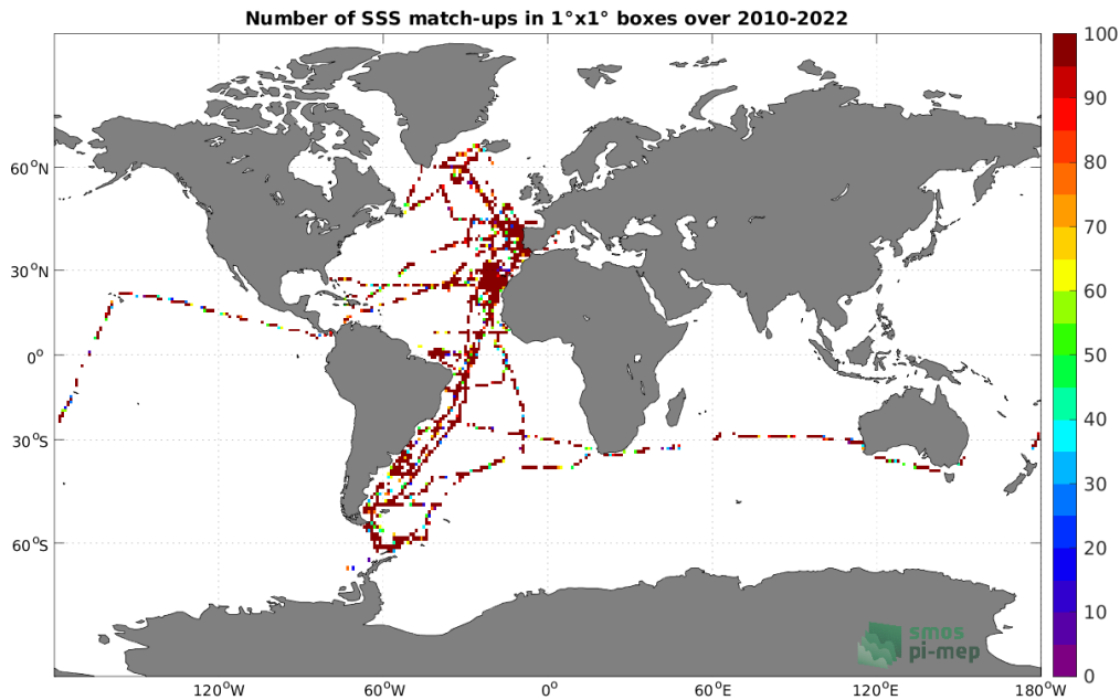
Figure 4: Number of SSS match-ups between TSG (CSIC-UTM) SSS and the SMOS SSS L2Q v331 - 0.25 Deg (CATDS-CPDC) SSS product for the Global Ocean Pi-MEP region over 1^\circ \times 1^\circ boxes and for the full satellite product period.
