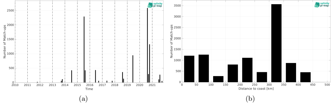
Figure 1: Number of match-ups between TSG (Amundsen) and SMOS SSS L2Q v331 - 0.25 Deg (CATDS-CPDC) SSS as a function of time (a) and as function of the distance to coast (b) over the Global Ocean Pi-MEP region and for the full satellite product period.
