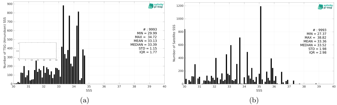
Figure 2: Histograms of SSS from TSG (Amundsen) (a) and SMOS SSS L2Q v331 - 0.25 Deg (CATDS-CPDC) (b) considering all match-up pairs per bins of 0.1 over the Global Ocean Pi-MEP region and for the full satellite product period.
