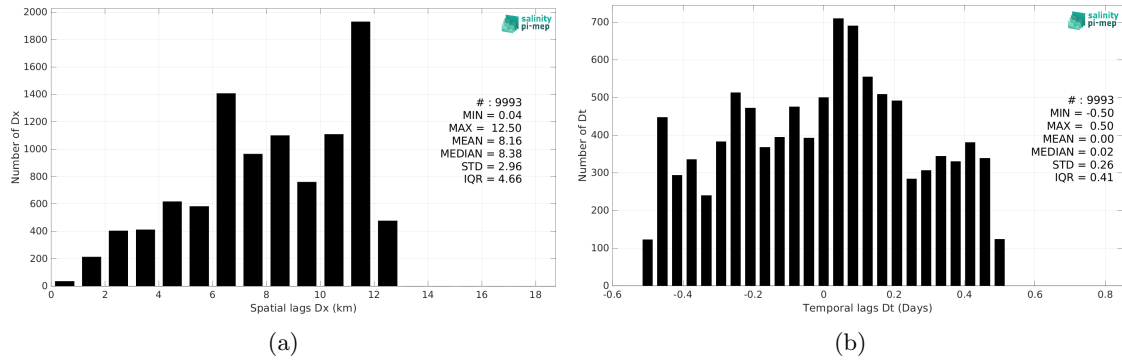
Figure 5: Histograms of the spatial (a) and temporal (b) lags between the location/time of the TSG (Amundsen) measurement and the date of the corresponding SMOS SSS L2Q v331 - 0.25 Deg (CATDS-CPDC) SSS pixel.
