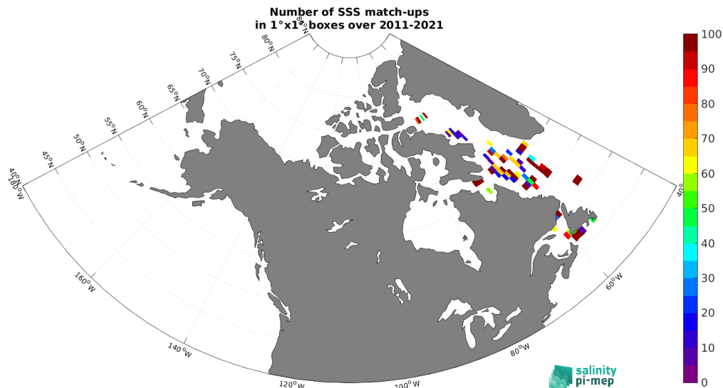
Figure 4: Number of SSS match-ups between TSG (Amundsen) SSS and the SMOS SSS L2Q v331 - 0.25 Deg (CATDS-CPDC) SSS product for the Global Ocean Pi-MEP region over 1^\circ \times 1^\circ boxes and for the full satellite product period.
