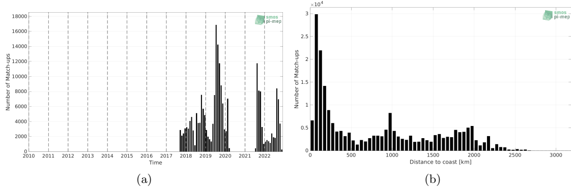
Figure 1: Number of match-ups between Saildrone and SMOS SSS L2Q v331 - 0.25 Deg (CATDS-CPDC) SSS as a function of time (a) and as function of the distance to coast (b) over the Global Ocean Pi-MEP region and for the full satellite product period.
