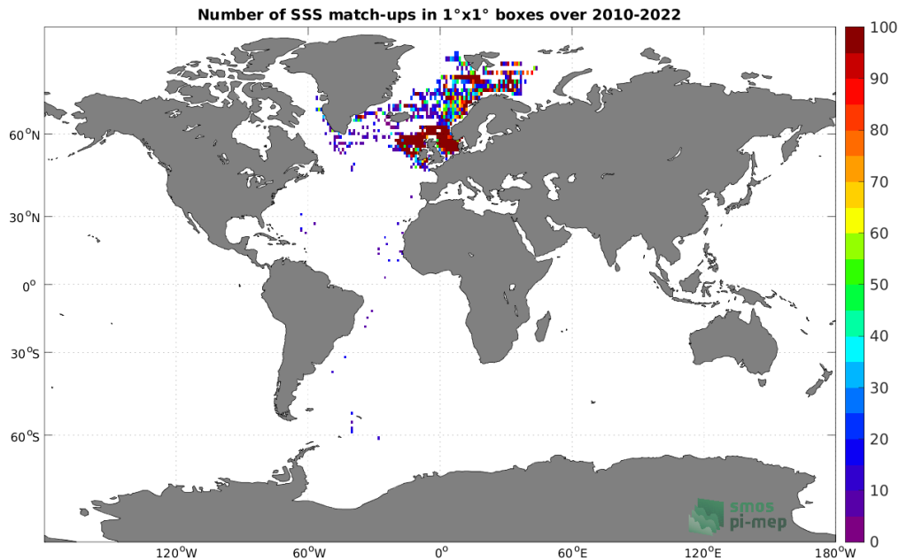
Figure 4: Number of SSS match-ups between ICES SSS and the SMOS SSS L2Q v331 - 0.25 Deg (CATDS-CPDC) SSS product for the Global Ocean Pi-MEP region over 1^\circ \times 1^\circ boxes and for the full satellite product period.
