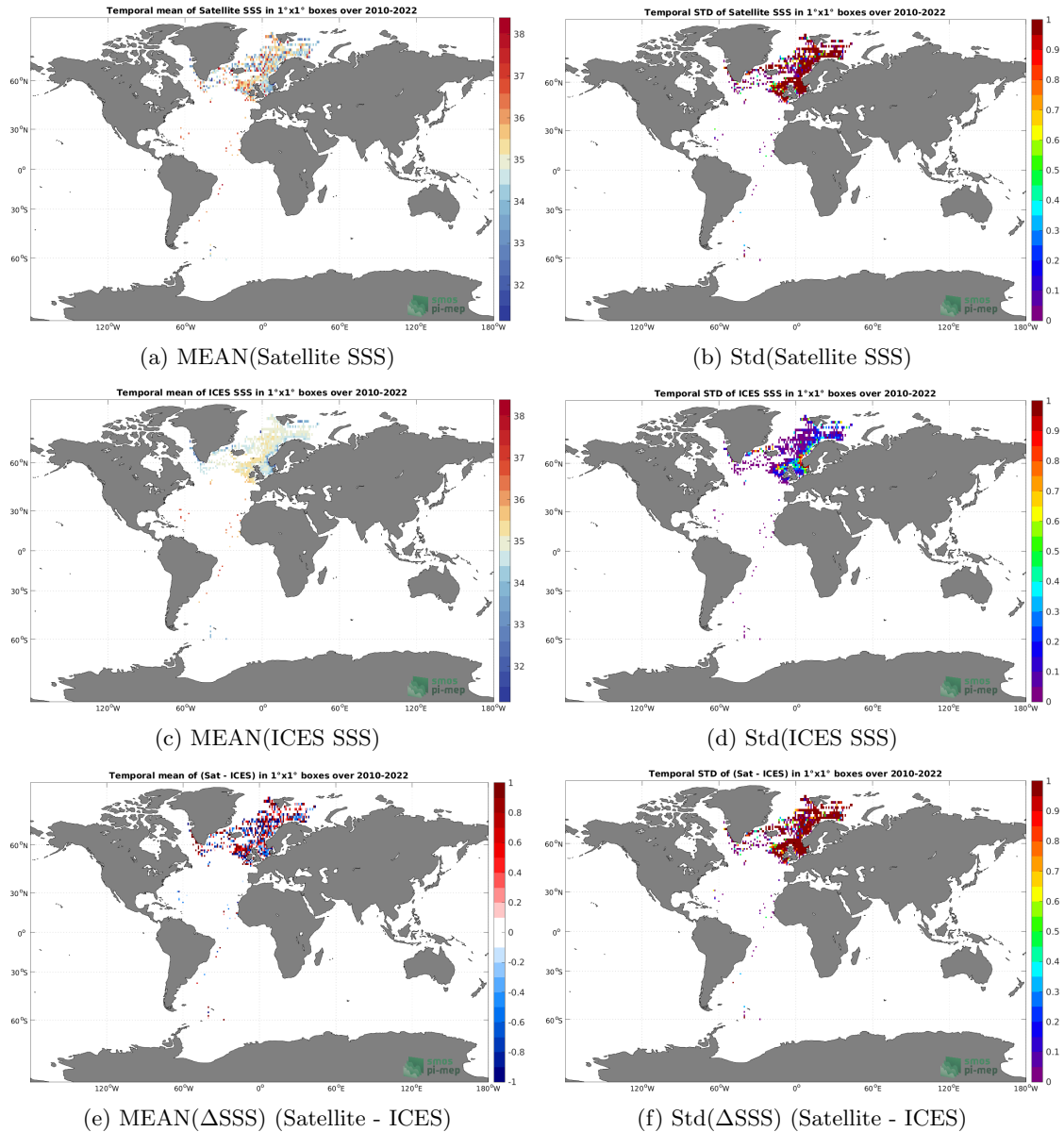
Figure 6: Temporal mean (left) and Std (right) of SSS from SMOS SSS L2Q v331 - 0.25 Deg (CATDS-CPDC) (top), ICES (middle), and of \Delta SSS (Satellite - ICES). Only match-up pairs are used to generate these maps.
