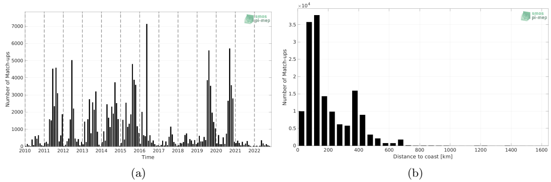
Figure 1: Number of match-ups between ICES and SMOS SSS L2Q v331 - 0.25 Deg (CATDS-CPDC) SSS as a function of time (a) and as function of the distance to coast (b) over the Global Ocean Pi-MEP region and for the full satellite product period.
