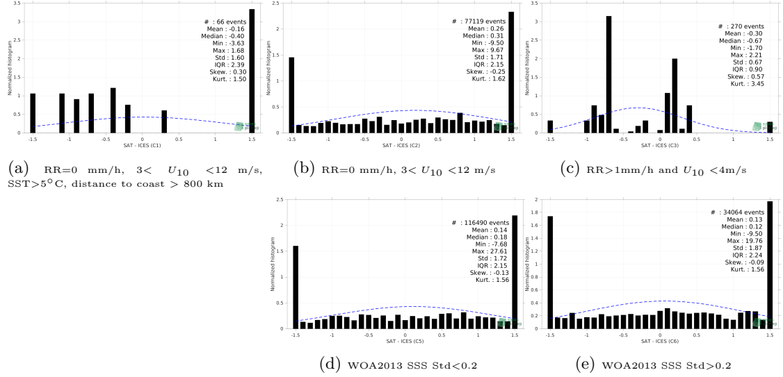
Figure 13: Normalized histogram of \Delta SSS (SMOS SSS L2Q v331 - 0.25 Deg (CATDS-CPDC) - ICES) for 5 different subdatasets corresponding to: RR=0 mm/h, 3 < U_{10} < 12 m/s, SST>5°C, distance to coast > 800 km (a), RR=0 mm/h, 3 < U_{10} < 12 m/s (b), RR>1mm/h and U_{10} < 4 m/s (c), WOA2013 SSS Std<0.2 (d), WOA2013 SSS Std>0.2 (e).
