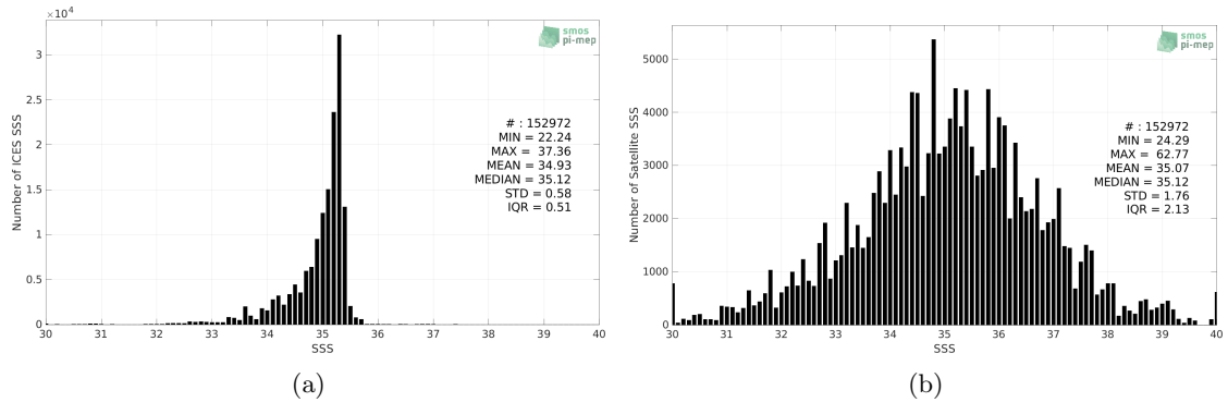
Figure 2: Histograms of SSS from ICES (a) and SMOS SSS L2Q v331 - 0.25 Deg (CATDS-CPDC) (b) considering all match-up pairs per bins of 0.1 over the Global Ocean Pi-MEP region and for the full satellite product period.
