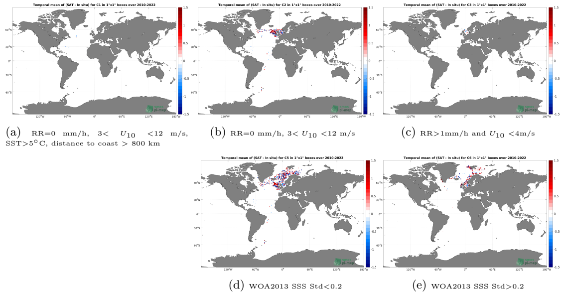
Figure 12: Temporal mean gridded over spatial boxes of size 1^\circ \times 1^\circ of \Delta SSS (SMOS SSS L2Q v331 - 0.25 Deg (CATDS-CPDC) - ICES) for 5 different subdatasets corresponding to:RR=0 mm/h, 3 < U_{10} < 12 m/s, SST >5^\circ\text{C} , distance to coast > 800 km (a), RR=0 mm/h, 3 < U_{10} < 12 m/s (b), RR >1 mm/h and U_{10} < 4 m/s (c), WOA2013 SSS Std <0.2 (d), WOA2013 SSS Std >0.2 (e).
