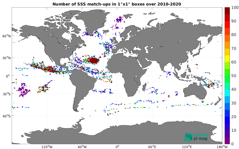
Figure 3: Number of SSS match-ups between Surface drifters SSS and the SMOS SSS L2Q v331 - 0.25 Deg (CATDS-CPDC) SSS product for the Global Ocean Pi-MEP region over 1°×1° boxes and for the full satellite product period.
