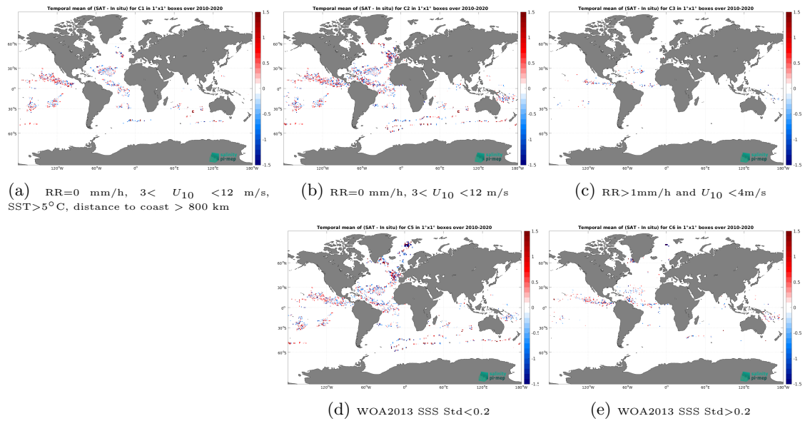
Figure 11: Temporal mean gridded over spatial boxes of size 1^\circ \times 1^\circ of \Delta\text{SSS} (SMOS SSS L2Q v331 - 0.25 Deg (CATDS-CPDC) - Surface drifters) for 5 different subdatasets corresponding to:RR=0 mm/h, 3 < U_{10} < 12 m/s, SST >5^\circ\text{C} , distance to coast > 800 km (a), RR=0 mm/h, 3 < U_{10} < 12 m/s (b), RR >1 mm/h and U_{10} < 4 m/s (c), WOA2013 SSS Std <0.2 (d), WOA2013 SSS Std >0.2 (e).
