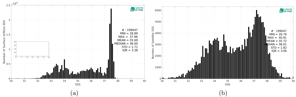
Figure 2: Histograms of SSS from Surface drifters (a) and SMOS SSS L2Q v331 - 0.25 Deg (CATDS-CPDC) (b) considering all match-up pairs per bins of 0.1 over the Global Ocean Pi-MEP region and for the full satellite product period.
