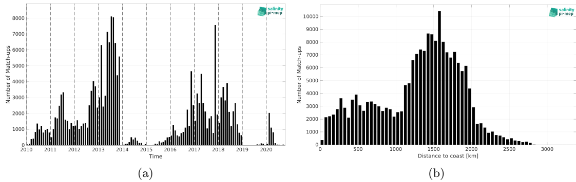
Figure 1: Number of match-ups between Surface drifters and SMOS SSS L2Q v331 - 0.25 Deg (CATDS-CPDC) SSS as a function of time (a) and as function of the distance to coast (b) over the Global Ocean Pi-MEP region and for the full satellite product period.
