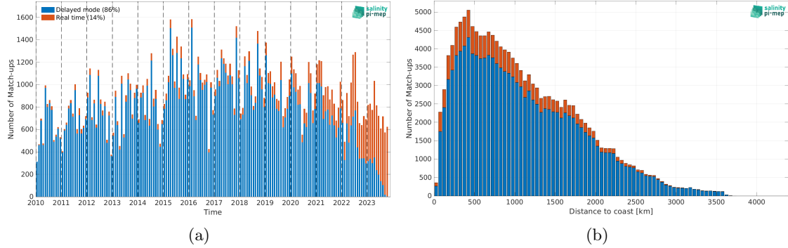
Figure 1: Number of match-ups between Argo and SMOS SSS L2Q v331 - 0.25 Deg (CATDS-CPDC) SSS as a function of time (a) and as function of the distance to coast (b) over the Global Ocean Pi-MEP region and for the full satellite product period.
