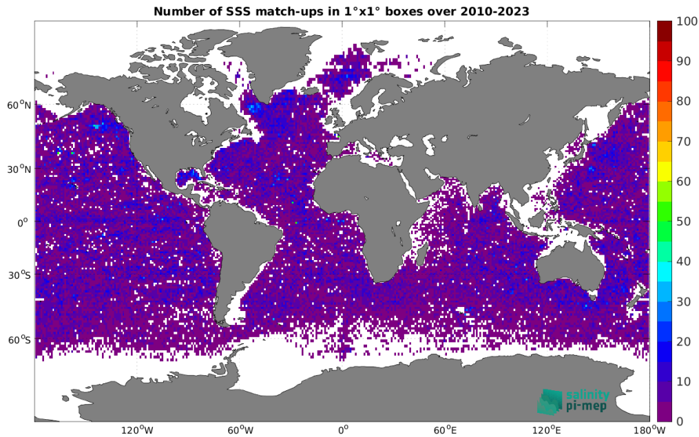
Figure 4: Number of SSS match-ups between Argo SSS and the SMOS SSS L2Q v331 - 0.25 Deg (CATDS-CPDC) SSS product for the Global Ocean Pi-MEP region over 1^\circ \times 1^\circ boxes and for the full satellite product period.
