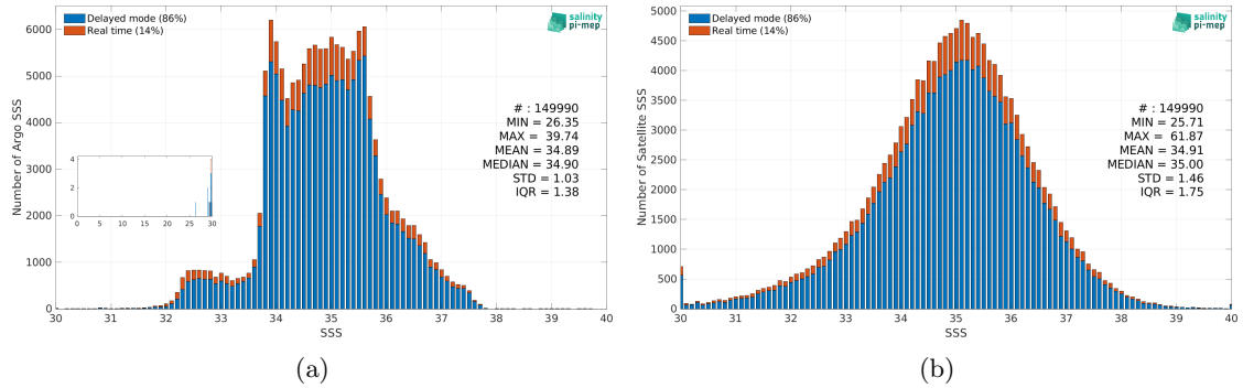
Figure 2: Histograms of SSS from Argo (a) and SMOS SSS L2Q v331 - 0.25 Deg (CATDS-CPDC) (b) considering all match-up pairs per bins of 0.1 over the Global Ocean Pi-MEP region and for the full satellite product period.
