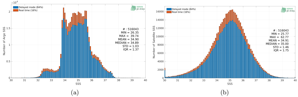
Figure 2: Histograms of SSS from Argo (a) and SMOS SSS L2Q v331 - 0.25 Deg (CATDS-CPDC) (b) considering all match-up pairs per bins of 0.1 over the Global Ocean Pi-MEP region and for the full satellite product period.
