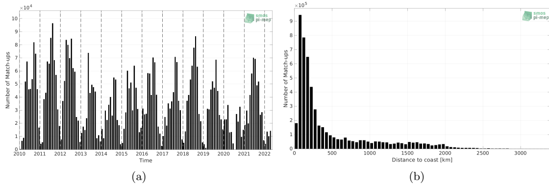
Figure 1: Number of match-ups between TSG (SAMOS) and SMOS SSS L2Q v330 - 0.25 Deg (CATDS-CPDC) SSS as a function of time (a) and as function of the distance to coast (b) over the Global Ocean Pi-MEP region and for the full satellite product period.
