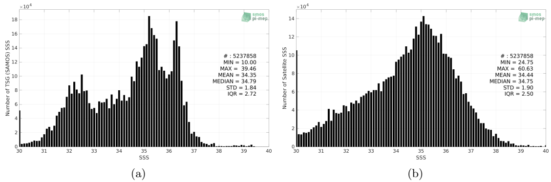
Figure 2: Histograms of SSS from TSG (SAMOS) (a) and SMOS SSS L2Q v330 - 0.25 Deg (CATDS-CPDC) (b) considering all match-up pairs per bins of 0.1 over the Global Ocean Pi-MEP region and for the full satellite product period.
