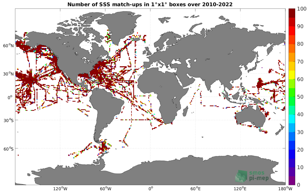
Figure 4: Number of SSS match-ups between TSG (SAMOS) SSS and the SMOS SSS L2Q v330 - 0.25 Deg (CATDS-CPDC) SSS product for the Global Ocean Pi-MEP region over 1^\circ \times 1^\circ boxes and for the full satellite product period.
