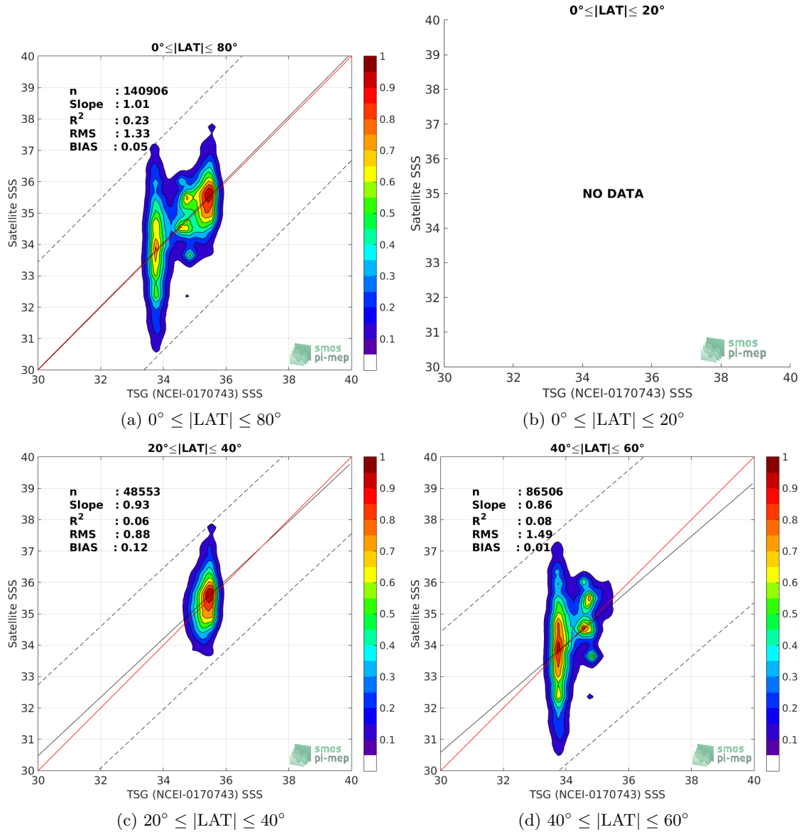
Figure 9: Contour maps of the concentration of SMOS SSS L2Q v330 - 0.25 Deg (CATDS-CPDC) SSS (y-axis) versus TSG (NCEI-0170743) SSS (x-axis) at match-up pairs for different latitude bands. For each plot, the red line shows x=y . The black thin and dashed lines indicate a linear fit through the data cloud and the \pm 95\% confidence levels, respectively. The number match-up pairs n , the slope and R^2 coefficient of the linear fit, the root mean square (RMS) and the mean bias between satellite and in situ data are indicated for each latitude band in each plots.
