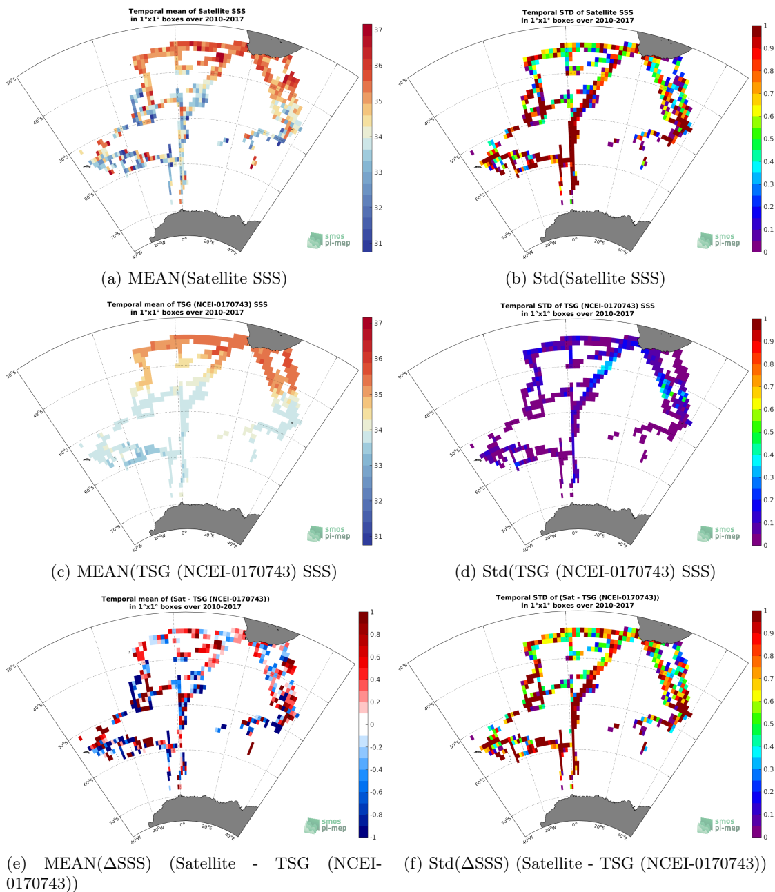
Figure 6: Temporal mean (left) and Std (right) of SSS from SMOS SSS L2Q v330 - 0.25 Deg (CATDS-CPDC) (top), TSG (NCEI-0170743) (middle), and of \Delta SSS (Satellite - TSG (NCEI-0170743)). Only match-up pairs are used to generate these maps.
