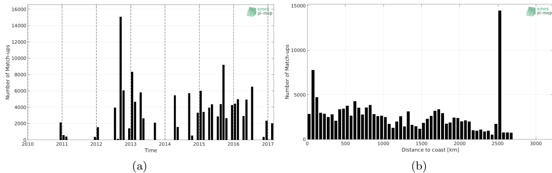
Figure 1: Number of match-ups between TSG (NCEI-0170743) and SMOS SSS L2Q v330 - 0.25 Deg (CATDS-CPDC) SSS as a function of time (a) and as function of the distance to coast (b) over the Global Ocean Pi-MEP region and for the full satellite product period.
