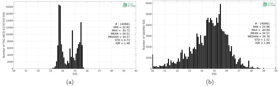
Figure 2: Histograms of SSS from TSG (NCEI-0170743) (a) and SMOS SSS L2Q v330 - 0.25 Deg (CATDS-CPDC) (b) considering all match-up pairs per bins of 0.1 over the Global Ocean Pi-MEP region and for the full satellite product period.
