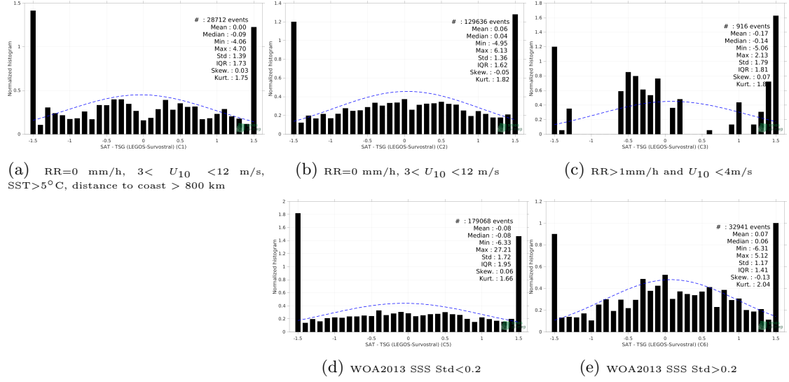
Figure 13: Normalized histogram of \Delta SSS (SMOS SSS L2Q v330 - 0.25 Deg (CATDS-CPDC) - TSG (LEGOS-Survostral)) for 5 different subdatasets corresponding to: RR=0 mm/h, 3 < U_{10} < 12 m/s, SST>5°C, distance to coast > 800 km (a), RR=0 mm/h, 3 < U_{10} < 12 m/s (b), RR>1mm/h and U_{10} < 4 m/s (c), WOA2013 SSS Std<0.2 (d), WOA2013 SSS Std>0.2 (e).
