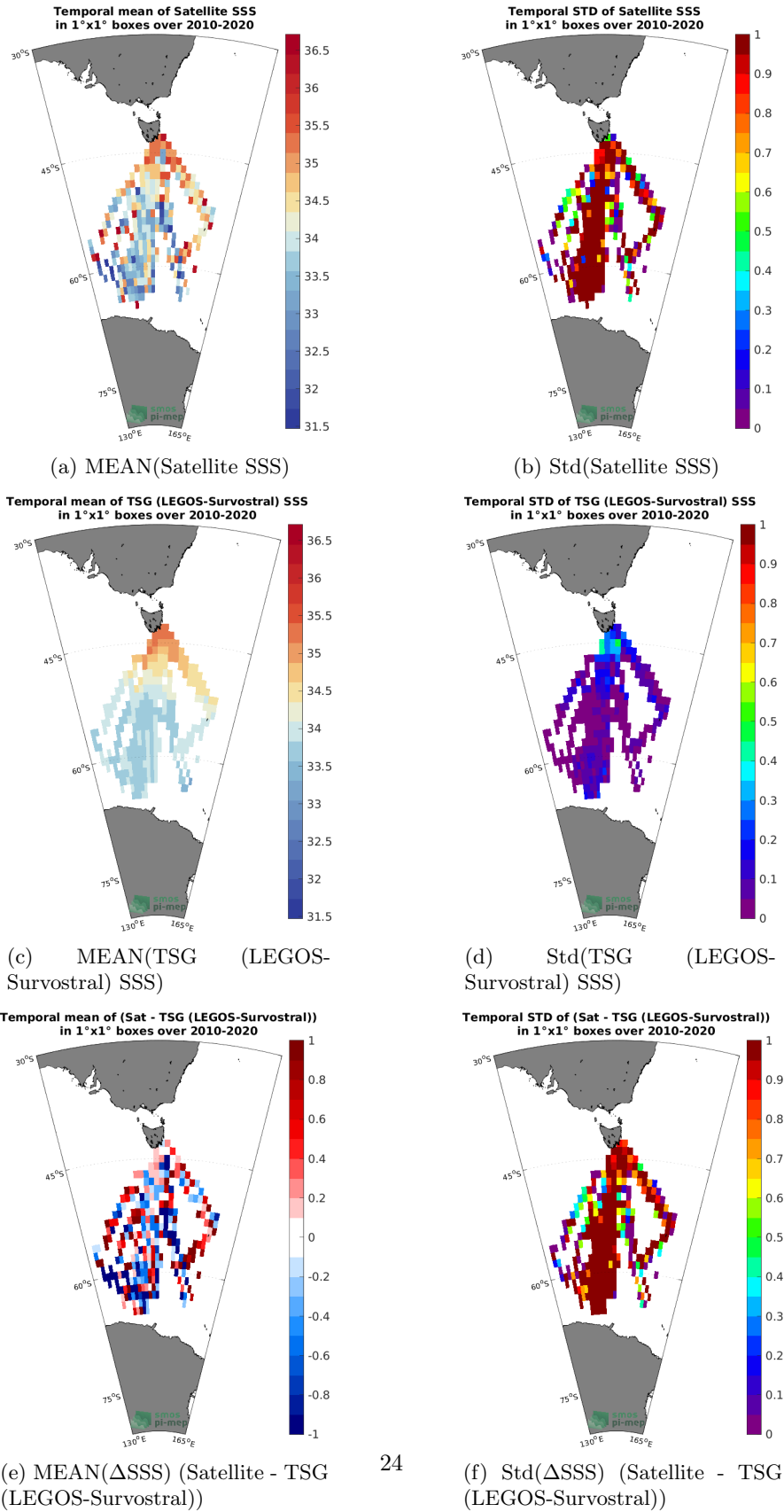
Figure 6: Temporal mean (left) and Std (right) of SSS from SMOS SSS L2Q v330 - 0.25 Deg (CATDS-CPDC) (top), TSG (LEGOS-Survostral) (middle), and of \Delta SSS (Satellite - TSG (LEGOS-Survostral)). Only match-up pairs are used to generate these maps.
