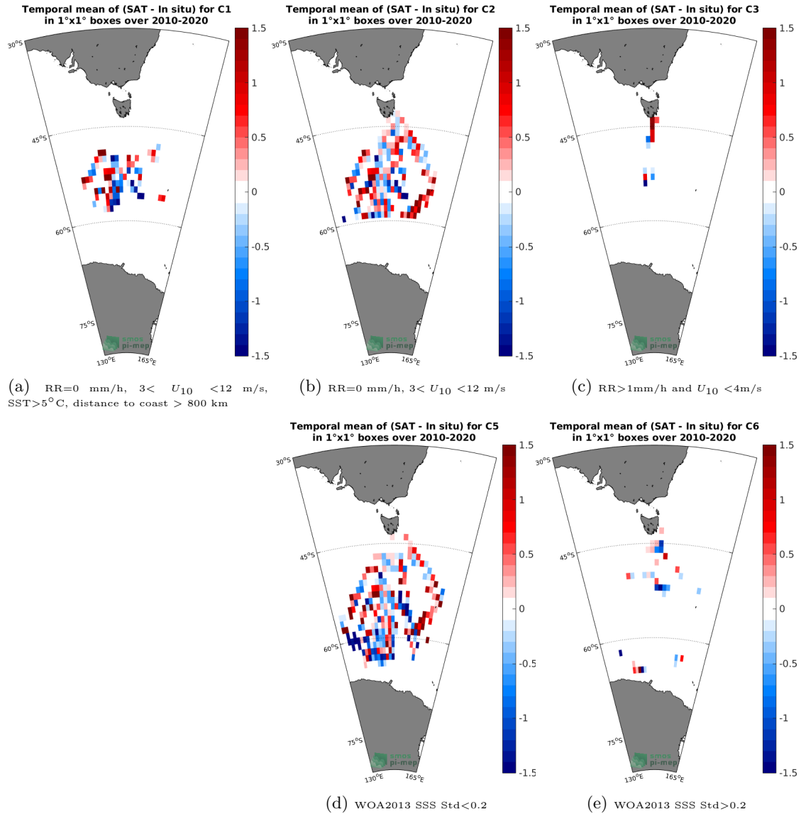
Figure 12: Temporal mean gridded over spatial boxes of size 1^\circ \times 1^\circ of \Delta SSS (SMOS SSS L2Q v330 - 0.25 Deg (CATDS-CPDC) - TSG (LEGOS-Survostral)) for 5 different subdatasets corresponding to:RR=0 mm/h, 3 < U_{10} < 12 m/s, SST>5°C, distance to coast > 800 km (a), RR=0 mm/h, 3 < U_{10} < 12 m/s (b), RR>1mm/h and U_{10} < 4 m/s (c), WOA2013 SSS Std<0.2 (d), WOA2013 SSS Std>0.2 (e).
