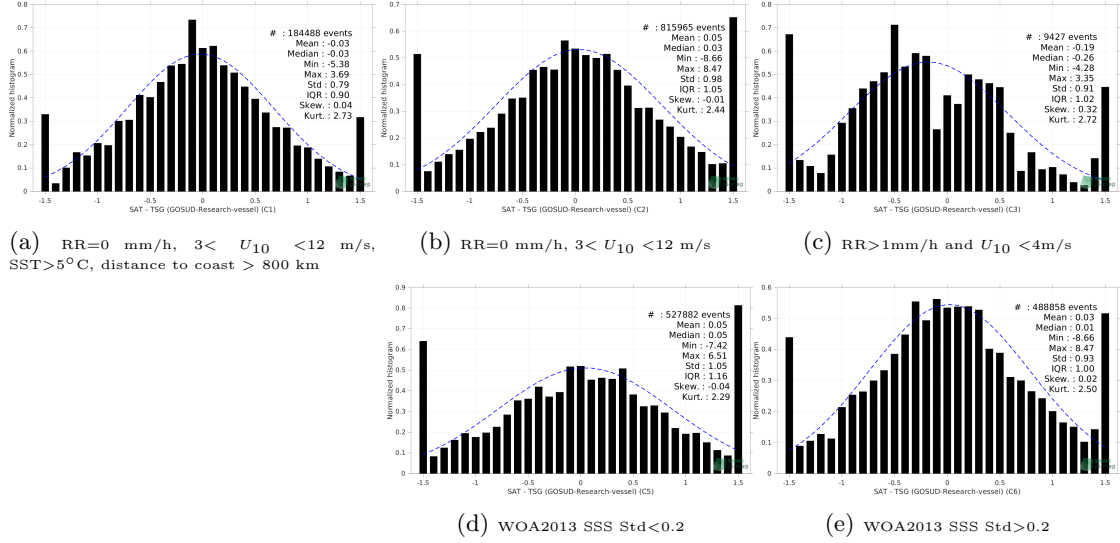
Figure 13: Normalized histogram of \Delta\text{SSS} (SMOS SSS L2Q v330 - 0.25 Deg (CATDS-CPDC) - TSG (GOSUD-Research-vessel)) for 5 different subdatasets corresponding to: RR=0 mm/h, 3 < U_{10} < 12 m/s, SST > 5^\circ\text{C} , distance to coast > 800 km (a), RR=0 mm/h, 3 < U_{10} < 12 m/s (b), RR > 1 mm/h and U_{10} < 4 m/s (c), WOA2013 SSS Std < 0.2 (d), WOA2013 SSS Std > 0.2 (e).
