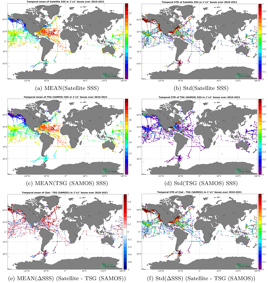
Figure 6: Temporal mean (left) and Std (right) of SSS from SMOS SSS L2Q v321 - 0.25 Deg (CATDS-CPDC) (top), TSG (SAMOS) (middle), and of \Delta SSS (Satellite - TSG (SAMOS)). Only match-up pairs are used to generate these maps.
