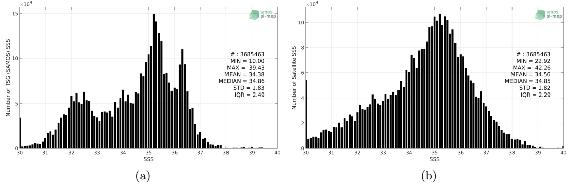
Figure 2: Histograms of SSS from TSG (SAMOS) (a) and SMOS SSS L2Q v321 - 0.25 Deg (CATDS-CPDC) (b) considering all match-up pairs per bins of 0.1 over the Global Ocean Pi-MEP region and for the full satellite product period.
