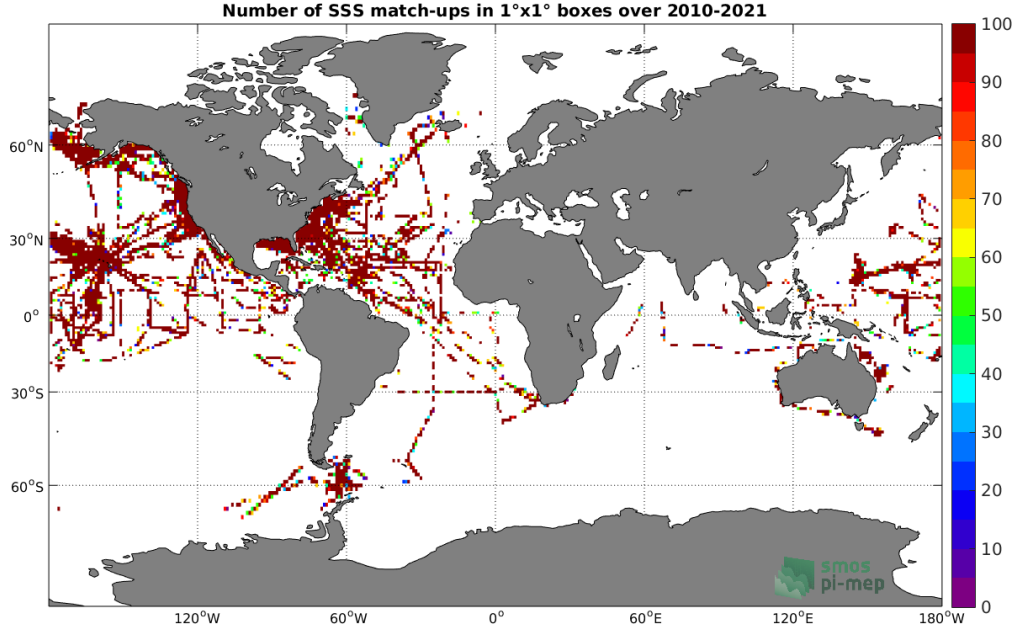
Figure 4: Number of SSS match-ups between TSG (SAMOS) SSS and the SMOS SSS L2Q v321 - 0.25 Deg (CATDS-CPDC) SSS product for the Global Ocean Pi-MEP region over 1^\circ \times 1^\circ boxes and for the full satellite product period.
