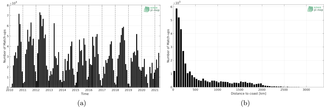
Figure 1: Number of match-ups between TSG (SAMOS) and SMOS SSS L2Q v321 - 0.25 Deg (CATDS-CPDC) SSS as a function of time (a) and as function of the distance to coast (b) over the Global Ocean Pi-MEP region and for the full satellite product period.
