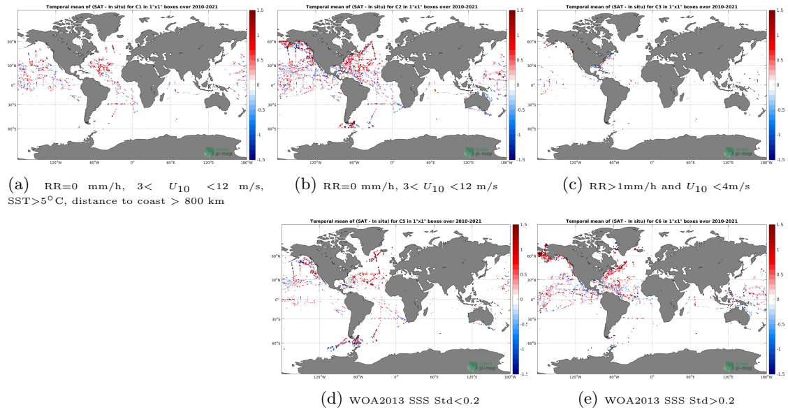
Figure 12: Temporal mean gridded over spatial boxes of size 1^\circ \times 1^\circ of \Delta SSS (SMOS SSS L2Q v321 - 0.25 Deg (CATDS-CPDC) - TSG (SAMOS)) for 5 different subdatasets corresponding to: RR=0 mm/h, 3 < U_{10} < 12 m/s, SST > 5^\circ C , distance to coast > 800 km (a), RR=0 mm/h, 3 < U_{10} < 12 m/s (b), RR > 1 mm/h and U_{10} < 4 m/s (c), WOA2013 SSS Std < 0.2 (d), WOA2013 SSS Std > 0.2 (e).
