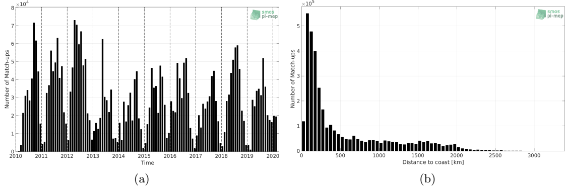
Figure 1: Number of match-ups between TSG-SAMOS and SMOS L2Q v321 - 0.25 Deg (CATDS-CPDC) SSS as a function of time (a) and as function of the distance to coast (b) over the Global Ocean Pi-MEP region and for the full satellite product period.
