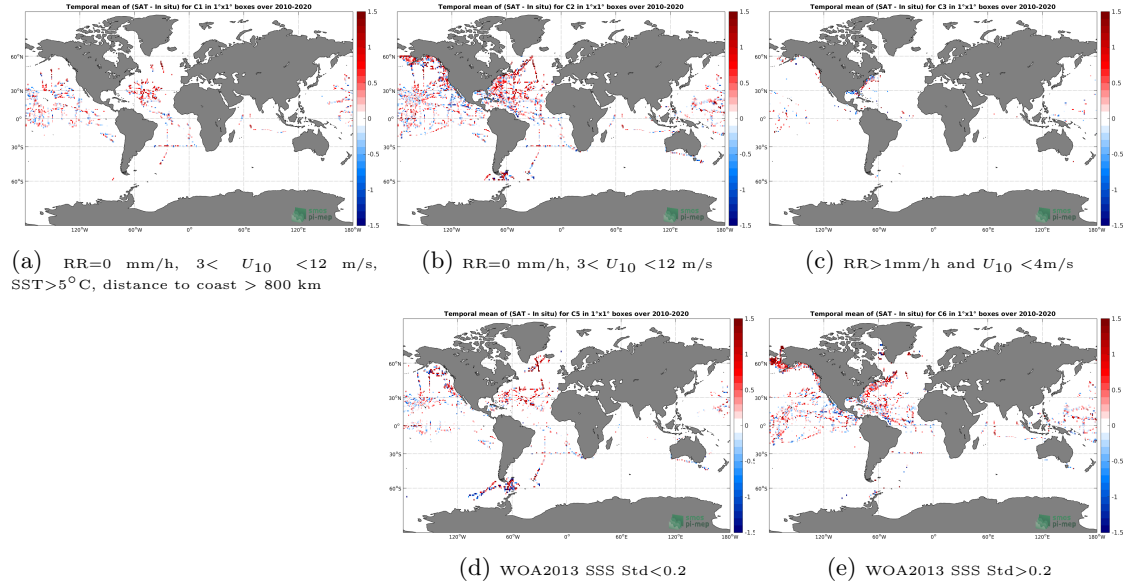
Figure 12: Temporal mean gridded over spatial boxes of size 1^\circ \times 1^\circ of \Delta SSS (SMOS L2Q v321 - 0.25 Deg (CATDS-CPDC) - TSG-SAMOS) for 5 different subdatasets corresponding to:RR=0 mm/h, 3 < U_{10} < 12 m/s, SST >5^\circ C, distance to coast > 800 km (a), RR=0 mm/h, 3 < U_{10} < 12 m/s (b), RR >1 mm/h and U_{10} < 4 m/s (c), WOA2013 SSS Std <0.2 (d), WOA2013 SSS Std >0.2 (e).
