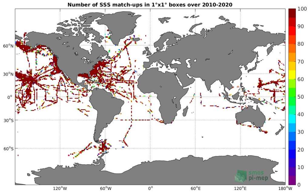
Figure 4: Number of SSS match-ups between TSG-SAMOS SSS and the SMOS L2Q v321 - 0.25 Deg (CATDS-CPDC) SSS product for the Global Ocean Pi-MEP region over 1°x1° boxes and for the full satellite product period.
