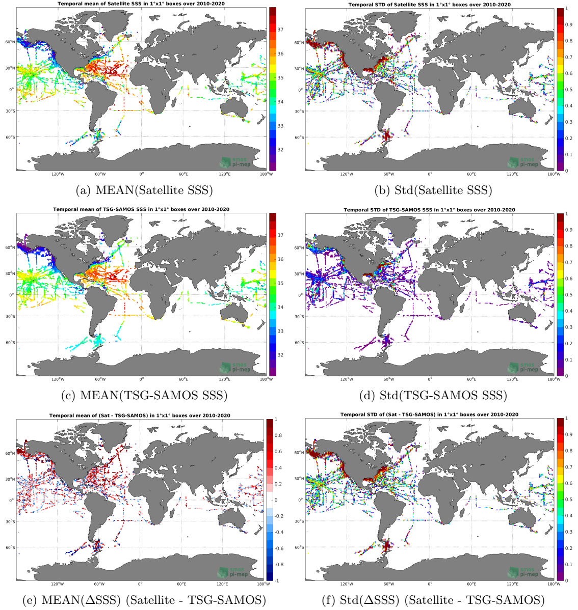
Figure 6: Temporal mean (left) and Std (right) of SSS from SMOS L2Q v321 - 0.25 Deg (CATDS-CPDC) (top), TSG-SAMOS (middle), and of \Delta SSS (Satellite - TSG-SAMOS). Only match-up pairs are used to generate these maps.
