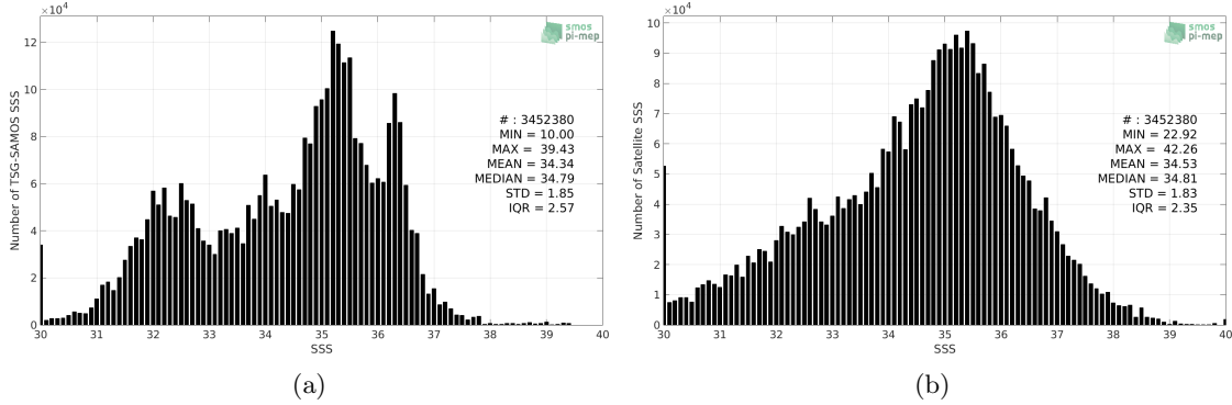
Figure 2: Histograms of SSS from TSG-SAMOS (a) and SMOS L2Q v321 - 0.25 Deg (CATDS-CPDC) (b) considering all match-up pairs per bins of 0.1 over the Global Ocean Pi-MEP region and for the full satellite product period.
