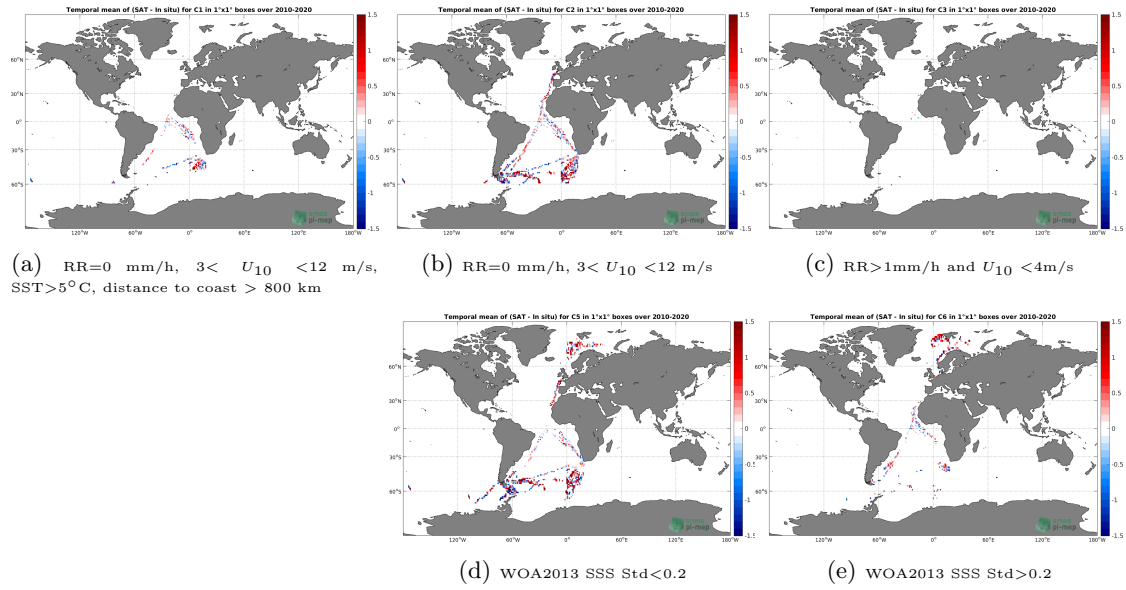
Figure 12: Temporal mean gridded over spatial boxes of size 1^\circ \times 1^\circ of \Delta SSS (SMOS SSS L2Q v321 - 0.25 Deg (CATDS-CPDC) - TSG (Polarstern)) for 5 different subdatasets corresponding to: RR=0 mm/h, 3 < U_{10} < 12 m/s, SST > 5^\circ\text{C} , distance to coast > 800 km (a), RR=0 mm/h, 3 < U_{10} < 12 m/s (b), RR > 1 mm/h and U_{10} < 4 m/s (c), WOA2013 SSS Std < 0.2 (d), WOA2013 SSS Std > 0.2 (e).
