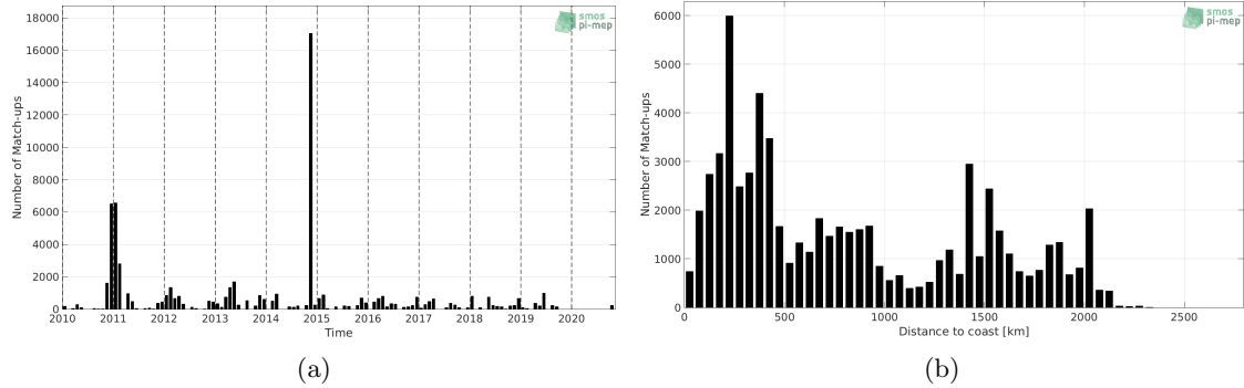
Figure 1: Number of match-ups between TSG (Polarstern) and SMOS SSS L2Q v321 - 0.25 Deg (CATDS-CPDC) SSS as a function of time (a) and as function of the distance to coast (b) over the Global Ocean Pi-MEP region and for the full satellite product period.
