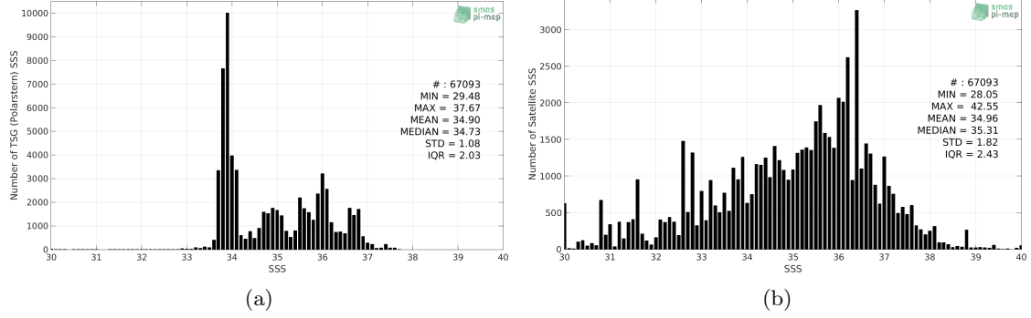
Figure 2: Histograms of SSS from TSG (Polarstern) (a) and SMOS SSS L2Q v321 - 0.25 Deg (CATDS-CPDC) (b) considering all match-up pairs per bins of 0.1 over the Global Ocean Pi-MEP region and for the full satellite product period.
