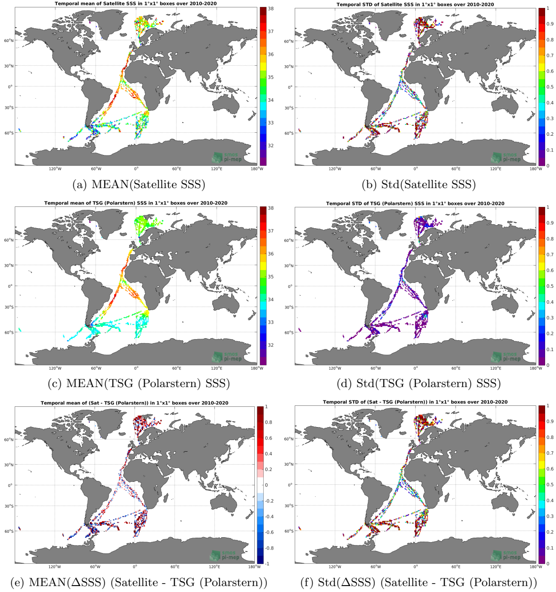
Figure 6: Temporal mean (left) and Std (right) of SSS from SMOS SSS L2Q v321 - 0.25 Deg (CATDS-CPDC) (top), TSG (Polarstern) (middle), and of \Delta SSS (Satellite - TSG (Polarstern)). Only match-up pairs are used to generate these maps.
