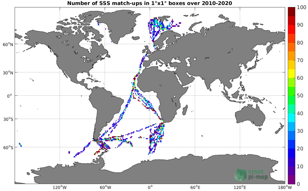
Figure 4: Number of SSS match-ups between TSG (Polarstern) SSS and the SMOS SSS L2Q v321 - 0.25 Deg (CATDS-CPDC) SSS product for the Global Ocean Pi-MEP region over 1^\circ \times 1^\circ boxes and for the full satellite product period.
