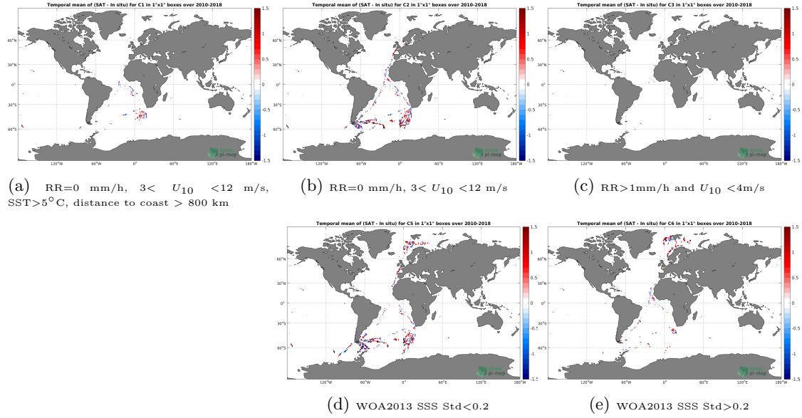
Figure 12: Temporal mean gridded over spatial boxes of size 1^\circ \times 1^\circ of \Delta SSS (SMOS-L3-CATDS-CPDC-V321-L2Q - TSG-POLARSTERN) for 5 different subdatasets corresponding to: RR=0 mm/h, 3 < U_{10} < 12 m/s, SST >5^\circ C, distance to coast > 800 km (a), RR=0 mm/h, 3 < U_{10} < 12 m/s (b), RR >1 mm/h and U_{10} < 4 m/s (c), WOA2013 SSS Std <0.2 (d), WOA2013 SSS Std >0.2 (e).
