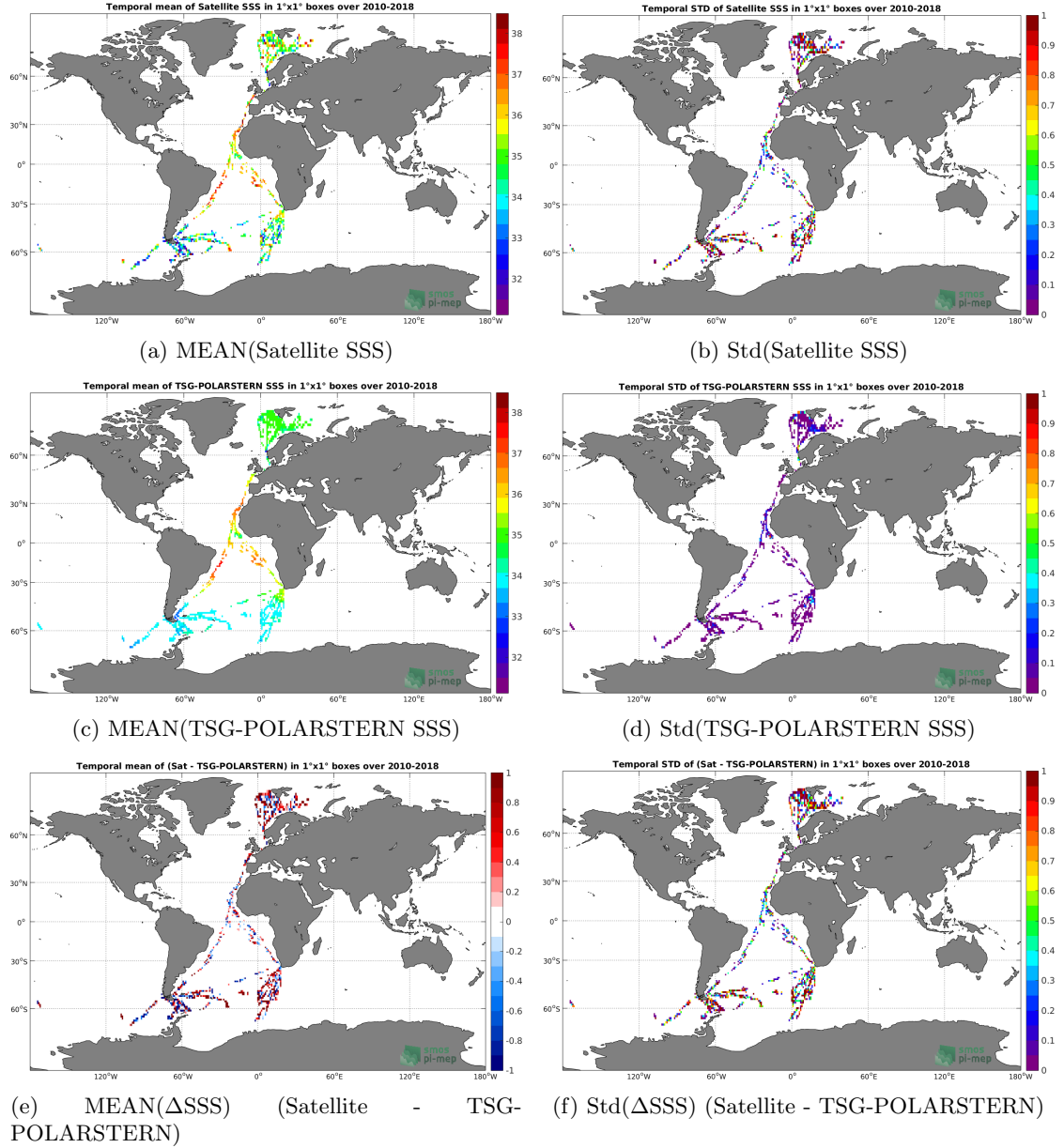
Figure 6: Temporal mean (left) and Std (right) of SSS from SMOS-L3-CATDS-CPDC-V321-L2Q (top), TSG-POLARSTERN (middle), and of \Delta SSS (Satellite - TSG-POLARSTERN). Only match-up pairs are used to generate these maps.
