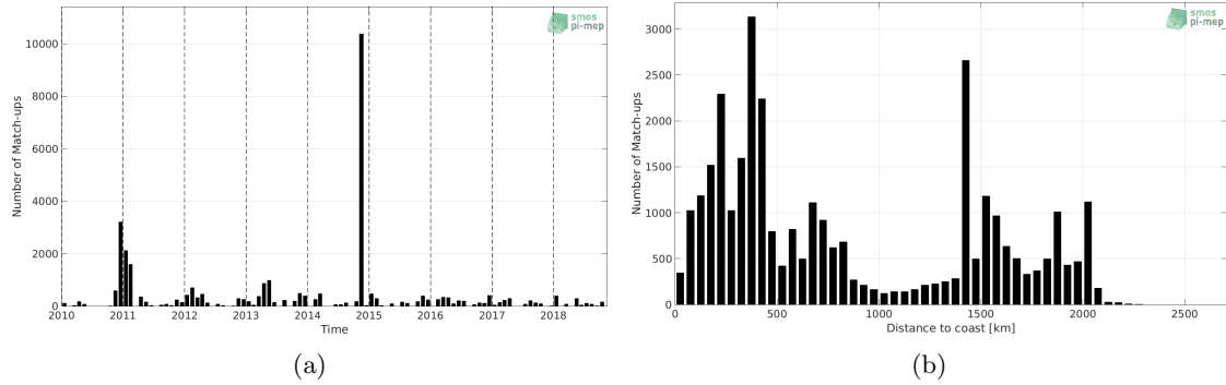
Figure 1: Number of match-ups between TSG-POLARSTERN and SMOS-L3-CATDS-CPDC-V321-L2Q SSS as a function of time (a) and as function of the distance to coast (b) over the Global Ocean Pi-MEP region and for the full satellite product period.
