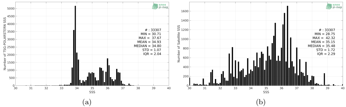
Figure 2: Histograms of SSS from TSG-POLARSTERN (a) and SMOS-L3-CATDS-CPDC-V321-L2Q (b) considering all match-up pairs per bins of 0.1 over the Global Ocean Pi-MEP region and for the full satellite product period.
