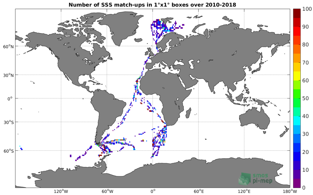
Figure 4: Number of SSS match-ups between TSG-POLARSTERN SSS and the SMOS-L3-CATDS-CPDC-V321-L2Q SSS product for the Global Ocean Pi-MEP region over 1^\circ \times 1^\circ boxes and for the full satellite product period.
