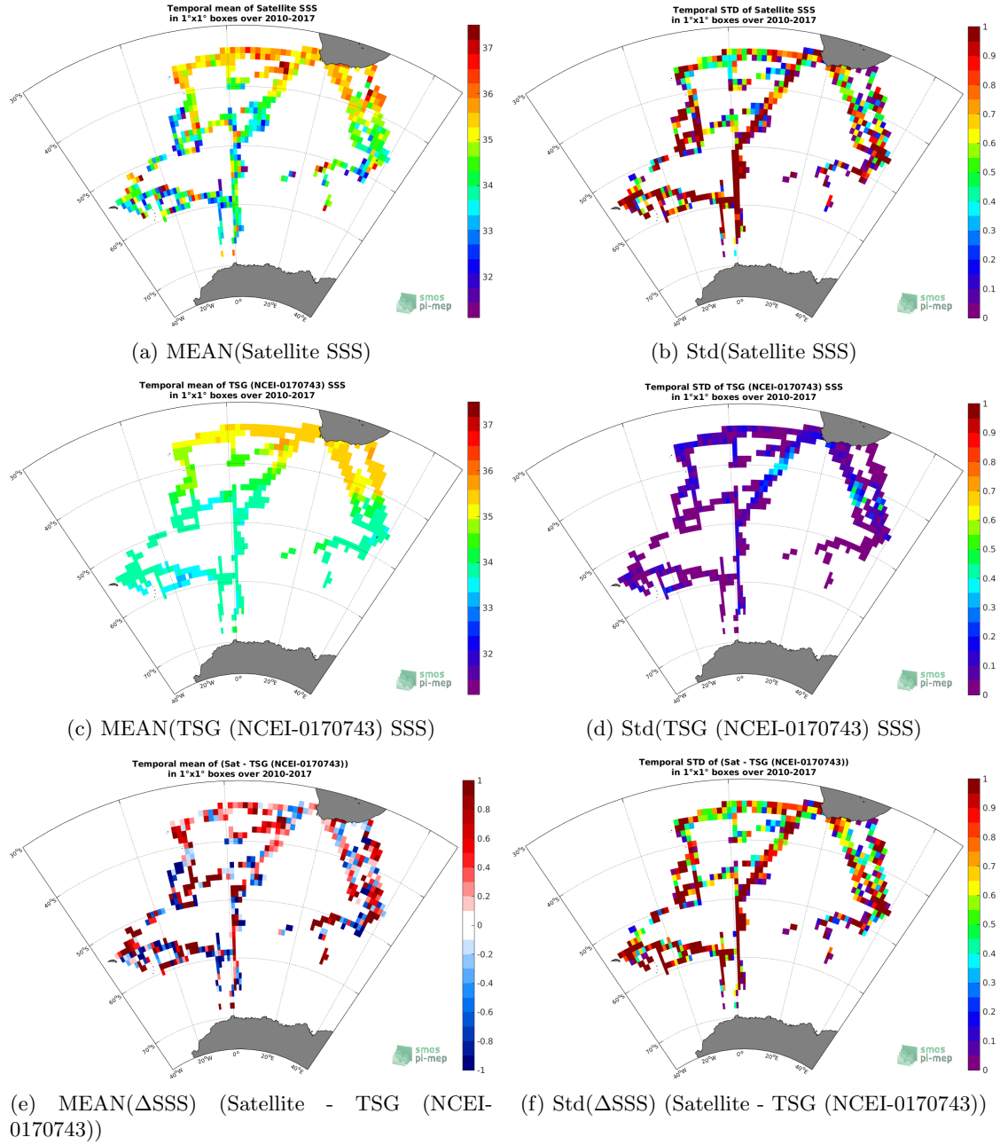
Figure 6: Temporal mean (left) and Std (right) of SSS from SMOS SSS L2Q v321 - 0.25 Deg (CATDS-CPDC) (top), TSG (NCEI-0170743) (middle), and of ΔSSS (Satellite - TSG (NCEI-0170743)). Only match-up pairs are used to generate these maps.
