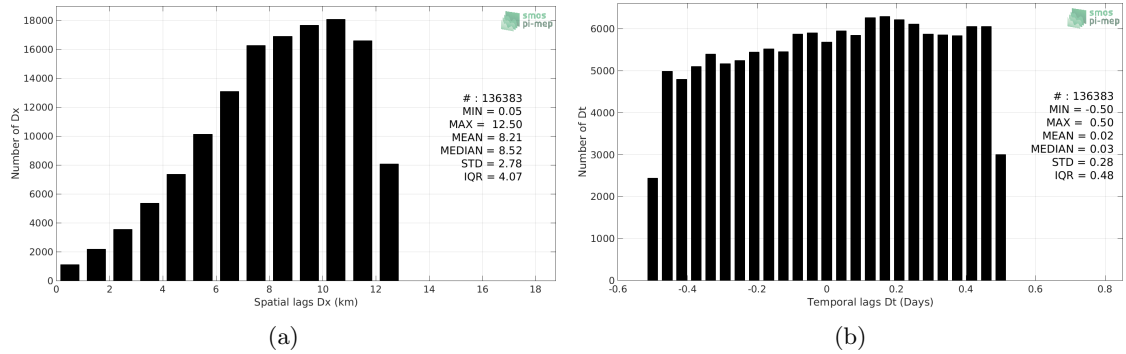
Figure 5: Histograms of the spatial (a) and temporal (b) lags between the location/time of the TSG (NCEI-0170743) measurement and the date of the corresponding SMOS SSS L2Q v321 - 0.25 Deg (CATDS-CPDC) SSS pixel.
