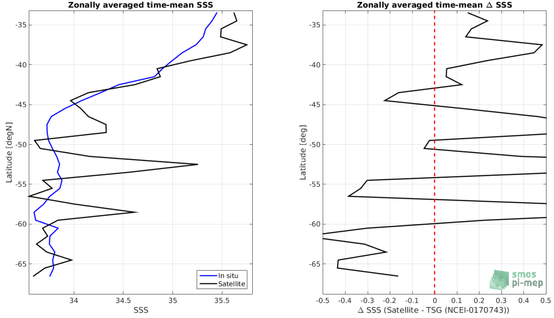
Figure 8: Left panel: Zonal mean SSS from SMOS SSS L2Q v321 - 0.25 Deg (CATDS-CPDC) satellite product (black) and from TSG (NCEI-0170743) (blue). Right panel: Zonal mean of \Delta SSS (Satellite - TSG (NCEI-0170743)) for all the collected Pi-MEP match-up pairs estimated over the full satellite product period.
