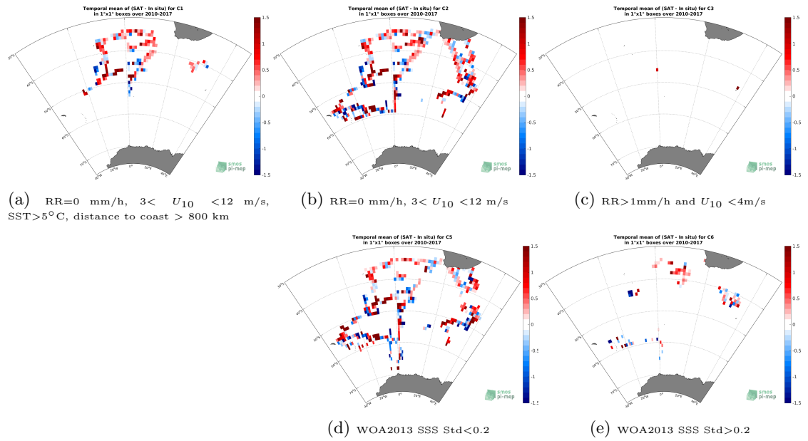
Figure 12: Temporal mean gridded over spatial boxes of size 1^\circ \times 1^\circ of \Delta SSS (SMOS SSS L2Q v321 - 0.25 Deg (CATDS-CPDC) - TSG (NCEI-0170743)) for 5 different subdatasets corresponding to:RR=0 mm/h, 3 < U_{10} < 12 m/s, SST >5^\circ C, distance to coast > 800 km (a), RR=0 mm/h, 3 < U_{10} < 12 m/s (b), RR >1 mm/h and U_{10} < 4 m/s (c), WOA2013 SSS Std <0.2 (d), WOA2013 SSS Std >0.2 (e).
