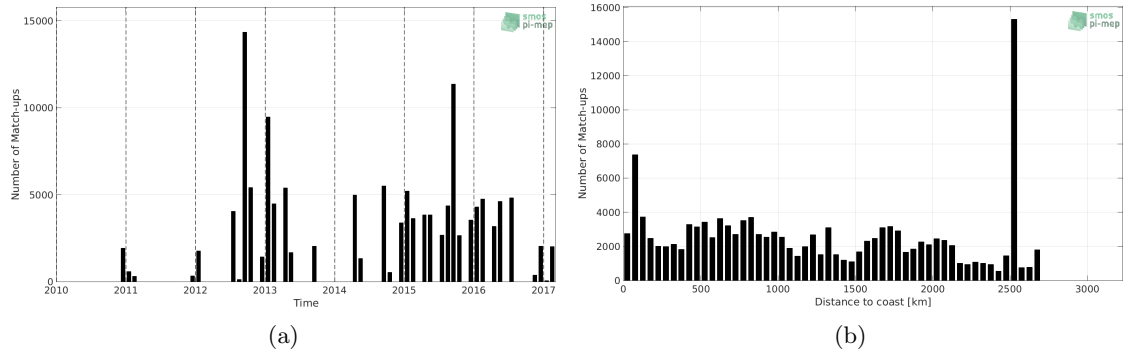
Figure 1: Number of match-ups between TSG (NCEI-0170743) and SMOS SSS L2Q v321 - 0.25 Deg (CATDS-CPDC) SSS as a function of time (a) and as function of the distance to coast (b) over the Global Ocean Pi-MEP region and for the full satellite product period.
