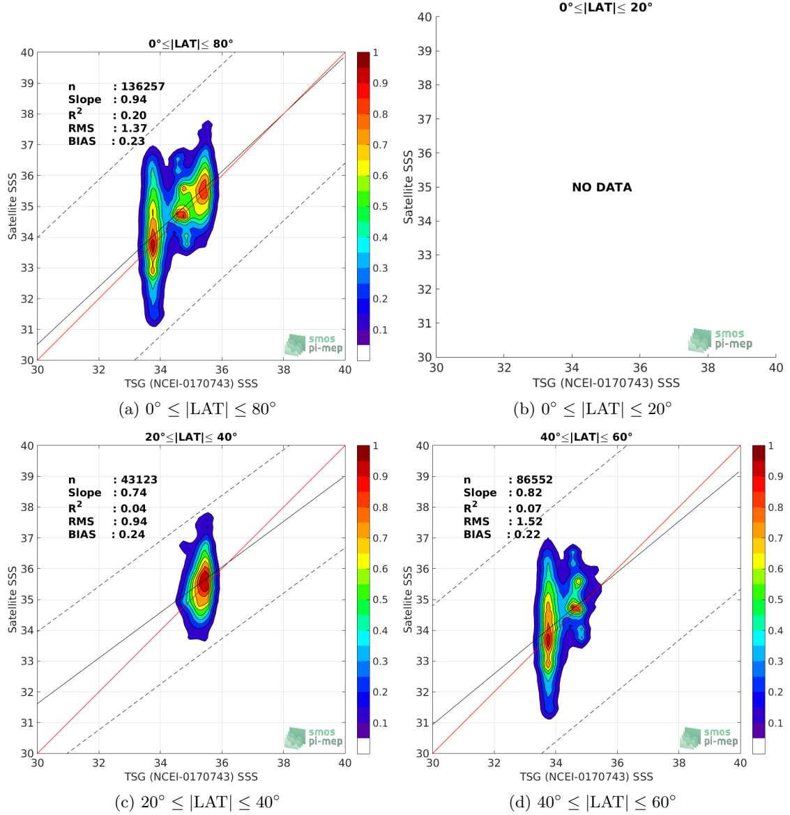
Figure 9: Contour maps of the concentration of SMOS SSS L2Q v321 - 0.25 Deg (CATDS-CPDC) SSS (y-axis) versus TSG (NCEI-0170743) SSS (x-axis) at match-up pairs for different latitude bands. For each plot, the red line shows x=y . The black thin and dashed lines indicate a linear fit through the data cloud and the \pm 95\% confidence levels, respectively. The number match-up pairs n , the slope and R^2 coefficient of the linear fit, the root mean square (RMS) and the mean bias between satellite and in situ data are indicated for each latitude band in each plots.
