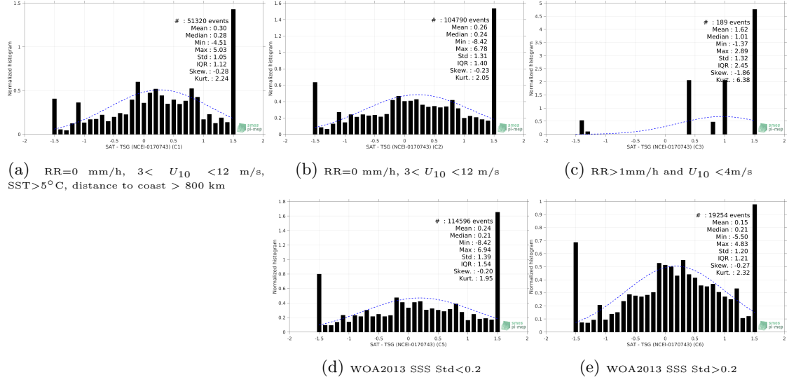
Figure 13: Normalized histogram of \Delta SSS (SMOS SSS L2Q v321 - 0.25 Deg (CATDS-CPDC) - TSG (NCEI-0170743)) for 5 different subdatasets corresponding to: RR=0 mm/h, 3 < U_{10} < 12 m/s, SST>5°C, distance to coast > 800 km (a), RR=0 mm/h, 3 < U_{10} < 12 m/s (b), RR>1mm/h and U_{10} < 4 m/s (c), WOA2013 SSS Std<0.2 (d), WOA2013 SSS Std>0.2 (e).
