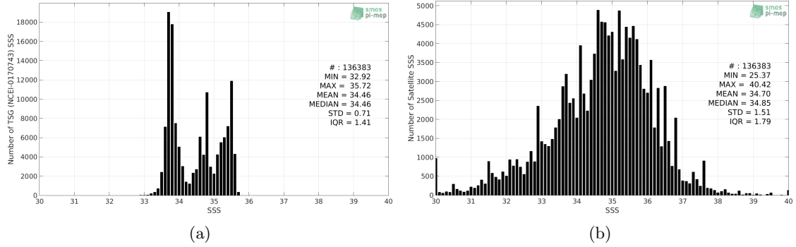
Figure 2: Histograms of SSS from TSG (NCEI-0170743) (a) and SMOS SSS L2Q v321 - 0.25 Deg (CATDS-CPDC) (b) considering all match-up pairs per bins of 0.1 over the Global Ocean Pi-MEP region and for the full satellite product period.
