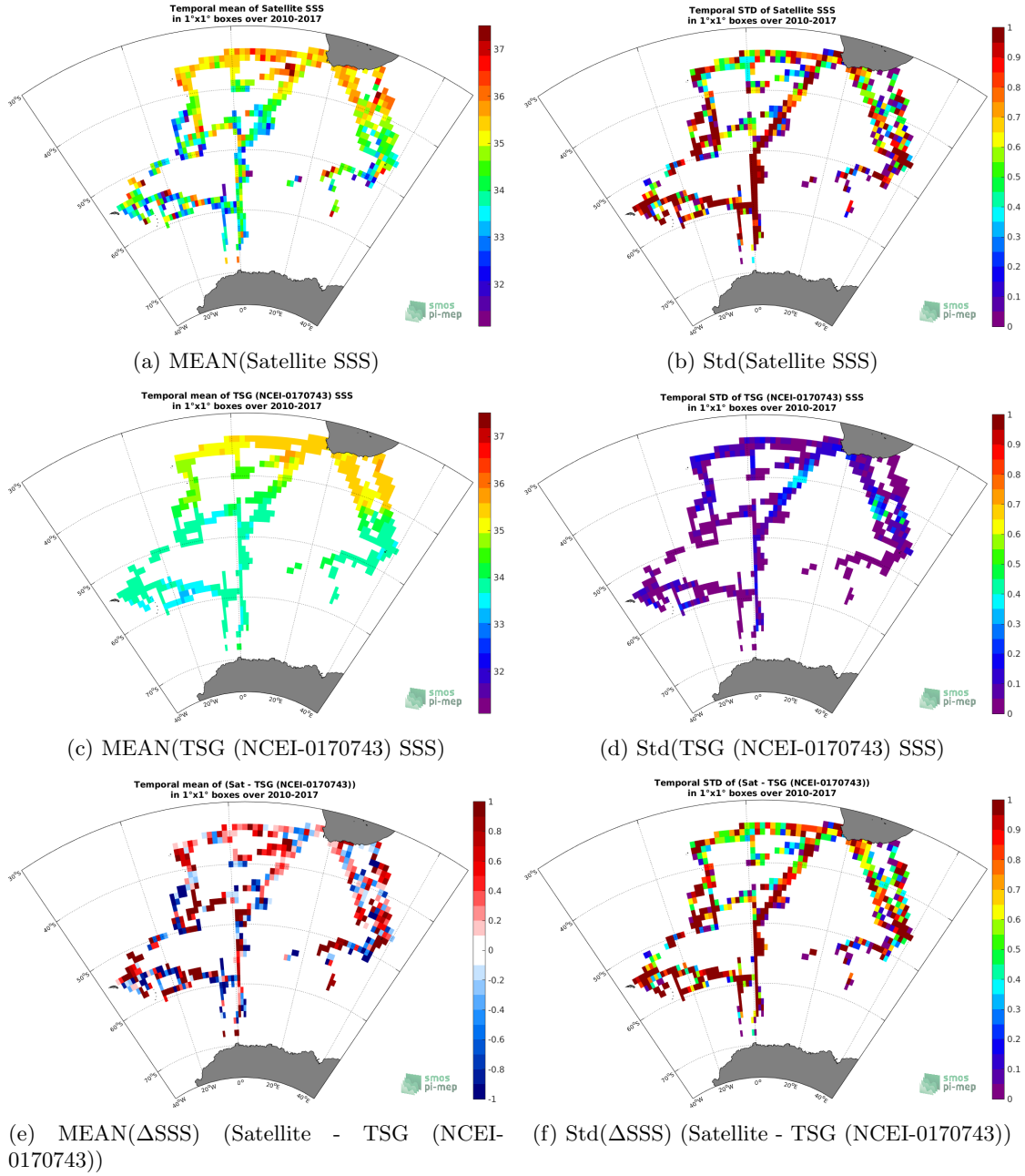
Figure 6: Temporal mean (left) and Std (right) of SSS from SMOS SSS L2Q v321 - 0.25 Deg (CATDS-CPDC) (top), TSG (NCEI-0170743) (middle), and of \Delta SSS (Satellite - TSG (NCEI-0170743)). Only match-up pairs are used to generate these maps.
