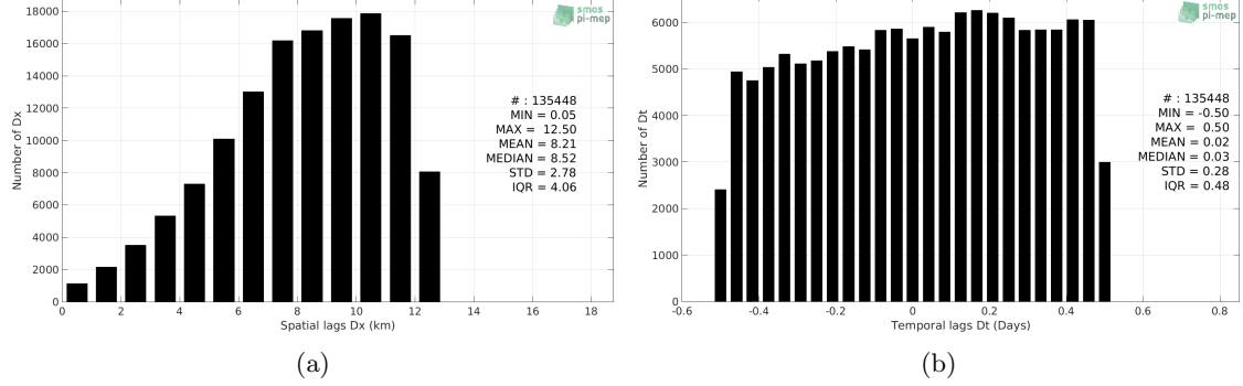
Figure 5: Histograms of the spatial (a) and temporal (b) lags between the time of the TSG (NCEI-0170743) measurements and the date of the corresponding SMOS SSS L2Q v321 - 0.25 Deg (CATDS-CPDC) SSS product.
