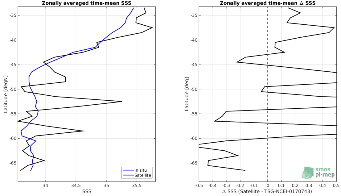
Figure 8: Left panel: Zonal mean SSS from SMOS L2Q v321 - 0.25 Deg (CATDS-CPDC) satellite product (black) and from TSG-NCEI-0170743 (blue). Right panel: Zonal mean of \Delta SSS (Satellite - TSG-NCEI-0170743) for all the collected Pi-MEP match-up pairs estimated over the full satellite product period.
