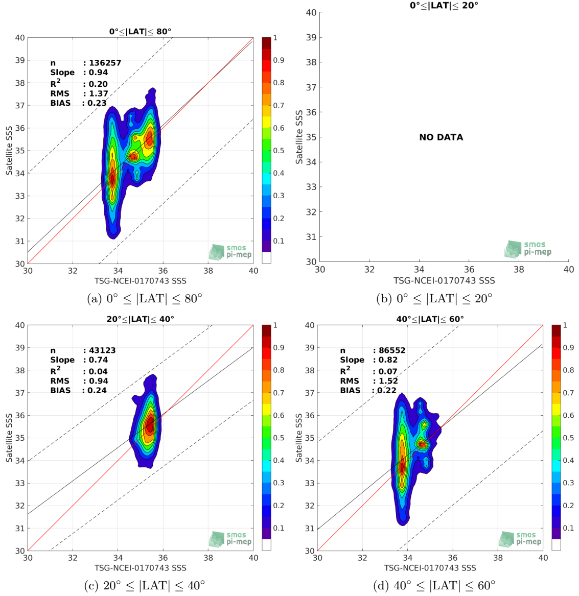
Figure 9: Contour maps of the concentration of SMOS L2Q v321 - 0.25 Deg (CATDS-CPDC) SSS (y-axis) versus TSG-NCEI-0170743 SSS (x-axis) at match-up pairs for different latitude bands. For each plot, the red line shows x=y . The black thin and dashed lines indicate a linear fit through the data cloud and the \pm 95\% confidence levels, respectively. The number match-up pairs n , the slope and R^2 coefficient of the linear fit, the root mean square (RMS) and the mean bias between satellite and in situ data are indicated for each latitude band in each plots.
