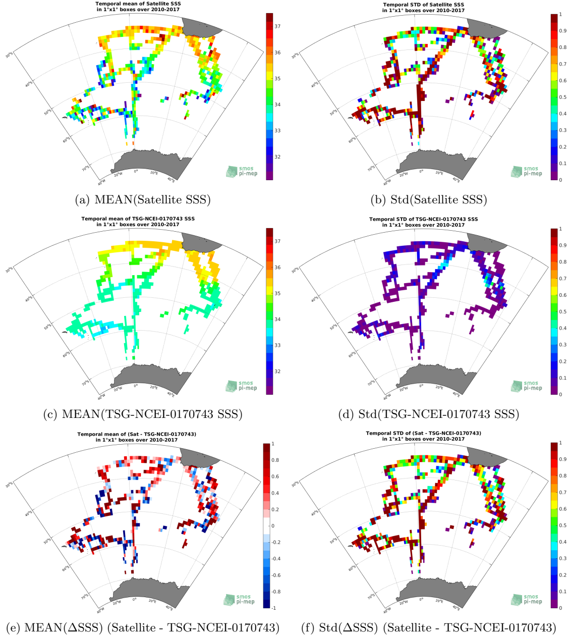
Figure 6: Temporal mean (left) and Std (right) of SSS from SMOS L2Q v321 - 0.25 Deg (CATDS-CPDC) (top), TSG-NCEI-0170743 (middle), and of \Delta SSS (Satellite - TSG-NCEI-0170743). Only match-up pairs are used to generate these maps.
