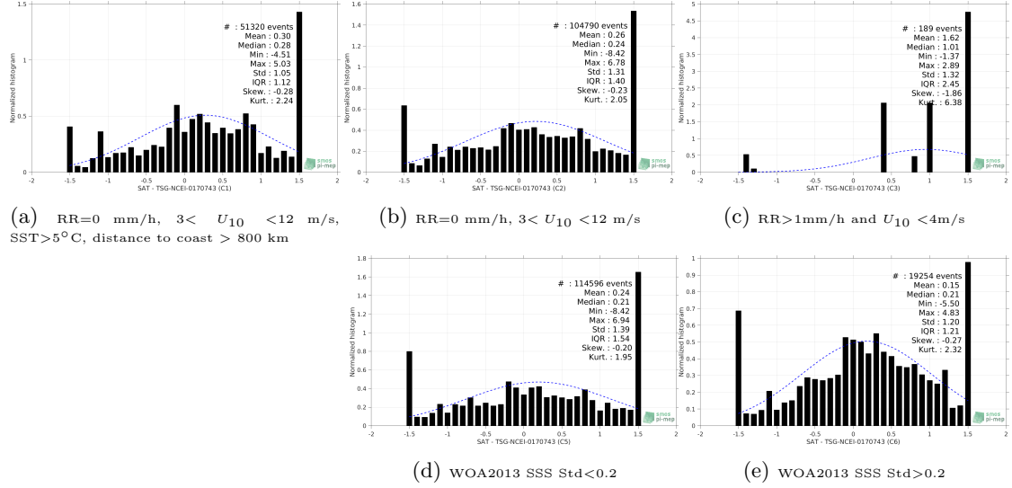
Figure 13: Normalized histogram of \Delta SSS (SMOS L2Q v321 - 0.25 Deg (CATDS-CPDC) - TSG-NCEI-0170743) for 5 different subdatasets corresponding to: RR=0 mm/h, 3 < U_{10} < 12 m/s, SST>5°C, distance to coast > 800 km (a), RR=0 mm/h, 3 < U_{10} < 12 m/s (b), RR>1mm/h and U_{10} < 4 m/s (c), WOA2013 SSS Std<0.2 (d), WOA2013 SSS Std>0.2 (e).
