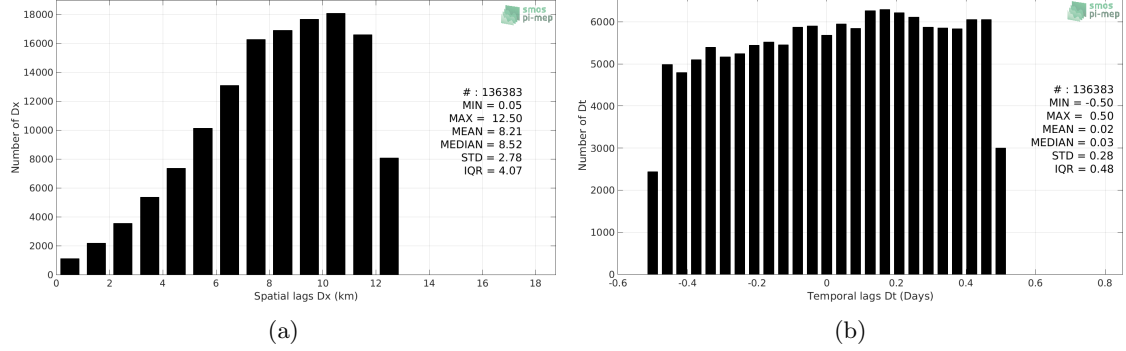
Figure 5: Histograms of the spatial (a) and temporal (b) lags between the time of the TSG-NCEI-0170743 measurements and the date of the corresponding SMOS L2Q v321 - 0.25 Deg (CATDS-CPDC) SSS product.
