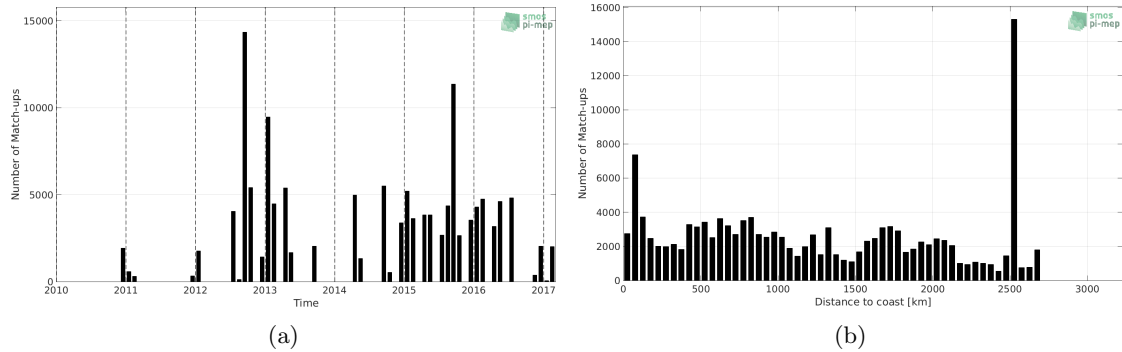
Figure 1: Number of match-ups between TSG-NCEI-0170743 and SMOS L2Q v321 - 0.25 Deg (CATDS-CPDC) SSS as a function of time (a) and as function of the distance to coast (b) over the Global Ocean Pi-MEP region and for the full satellite product period.
