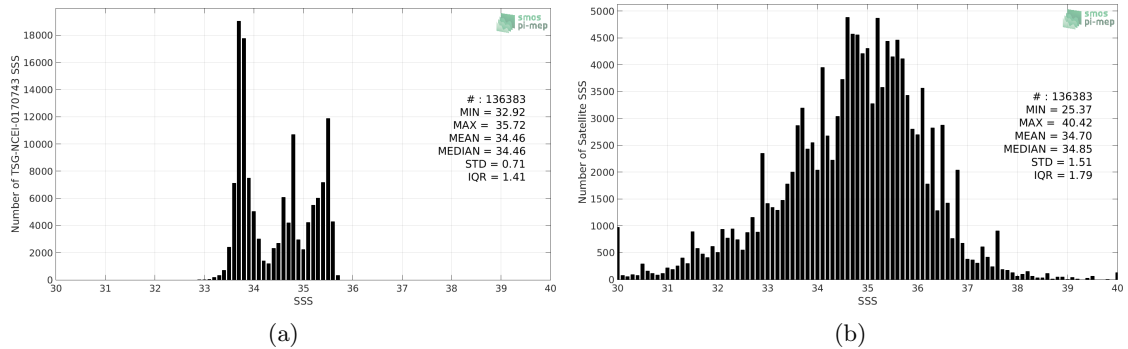
Figure 2: Histograms of SSS from TSG-NCEI-0170743 (a) and SMOS L2Q v321 - 0.25 Deg (CATDS-CPDC) (b) considering all match-up pairs per bins of 0.1 over the Global Ocean Pi-MEP region and for the full satellite product period.
