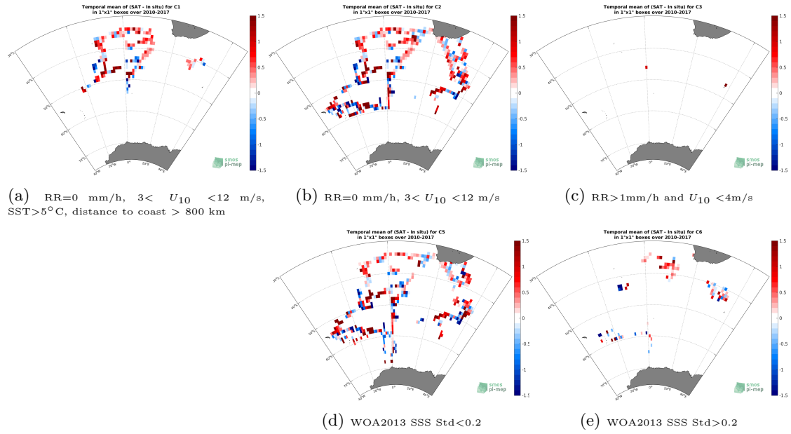
Figure 12: Temporal mean gridded over spatial boxes of size 1^\circ \times 1^\circ of \Delta SSS (SMOS L2Q v321 - 0.25 Deg (CATDS-CPDC) - TSG-NCEI-0170743) for 5 different subdatasets corresponding to:RR=0 mm/h, 3 < U_{10} < 12 m/s, SST >5^\circ\text{C} , distance to coast > 800 km (a), RR=0 mm/h, 3 < U_{10} < 12 m/s (b), RR >1 mm/h and U_{10} < 4 m/s (c), WOA2013 SSS Std <0.2 (d), WOA2013 SSS Std >0.2 (e).
