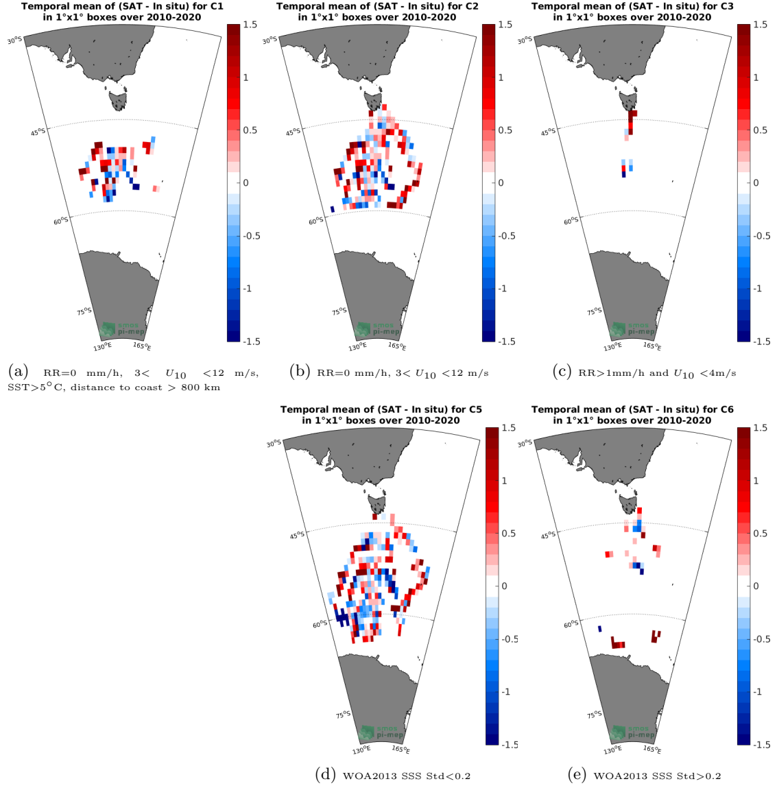
Figure 12: Temporal mean gridded over spatial boxes of size 1^\circ \times 1^\circ of \Delta\text{SSS} (SMOS SSS L2Q v321 - 0.25 Deg (CATDS-CPDC) - TSG (LEGOS-Survostral)) for 5 different subdatasets corresponding to: RR=0 mm/h, 3 < U_{10} < 12 m/s, SST > 5^\circ\text{C} , distance to coast > 800 km (a), RR=0 mm/h, 3 < U_{10} < 12 m/s (b), RR > 1 mm/h and U_{10} < 4 m/s (c), WOA2013 SSS Std < 0.2 (d), WOA2013 SSS Std > 0.2 (e).
