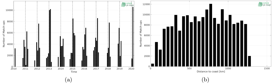
Figure 1: Number of match-ups between TSG (LEGOS-Survostral) and SMOS SSS L2Q v321 - 0.25 Deg (CATDS-CPDC) SSS as a function of time (a) and as function of the distance to coast (b) over the Global Ocean Pi-MEP region and for the full satellite product period.
