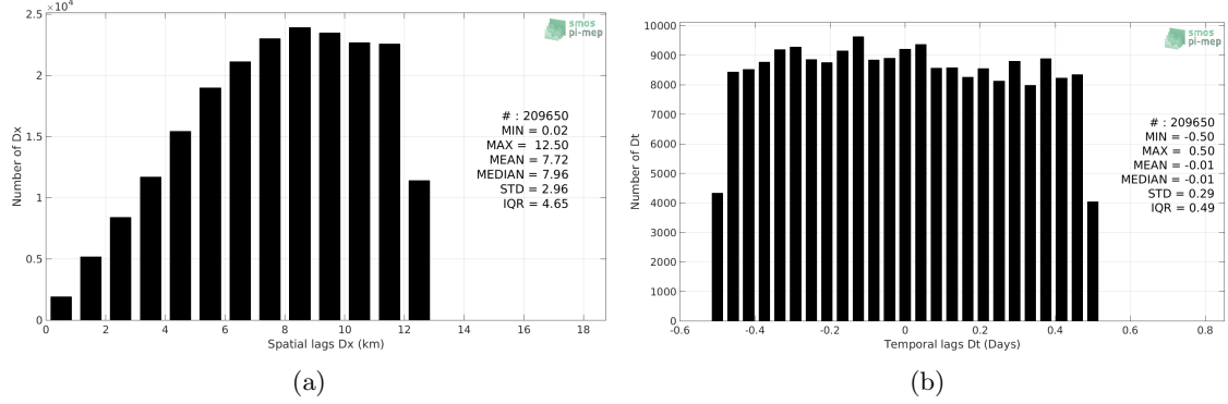
Figure 5: Histograms of the spatial (a) and temporal (b) lags between the location/time of the TSG (LEGOS-Survostral) measurement and the date of the corresponding SMOS SSS L2Q v321 - 0.25 Deg (CATDS-CPDC) SSS pixel.
