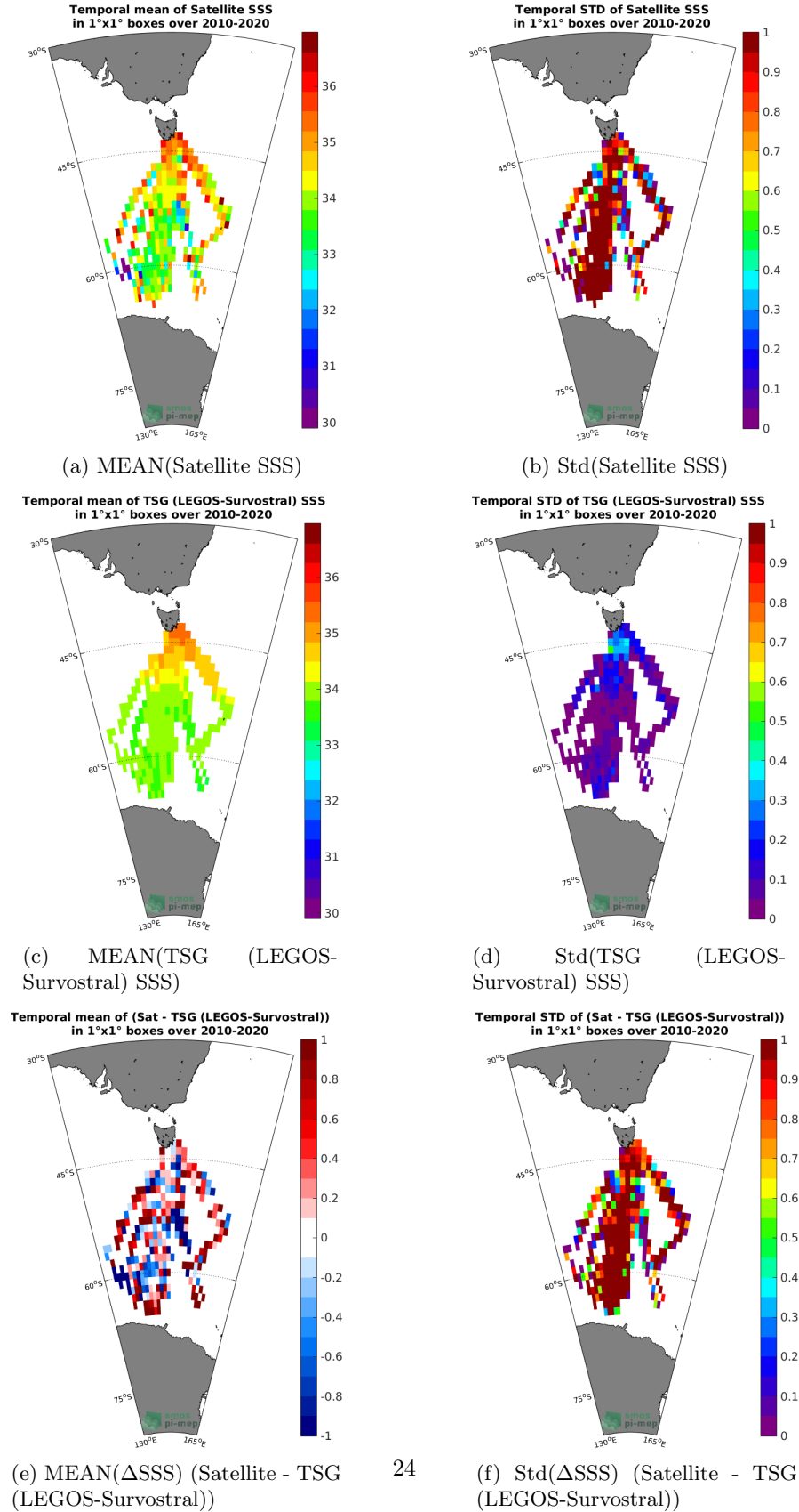
Figure 6: Temporal mean (left) and Std (right) of SSS from SMOS SSS L2Q v321 - 0.25 Deg (CATDS-CPDC) (top), TSG (LEGOS-Survostral) (middle), and of \Delta SSS (Satellite - TSG (LEGOS-Survostral)). Only match-up pairs are used to generate these maps.
