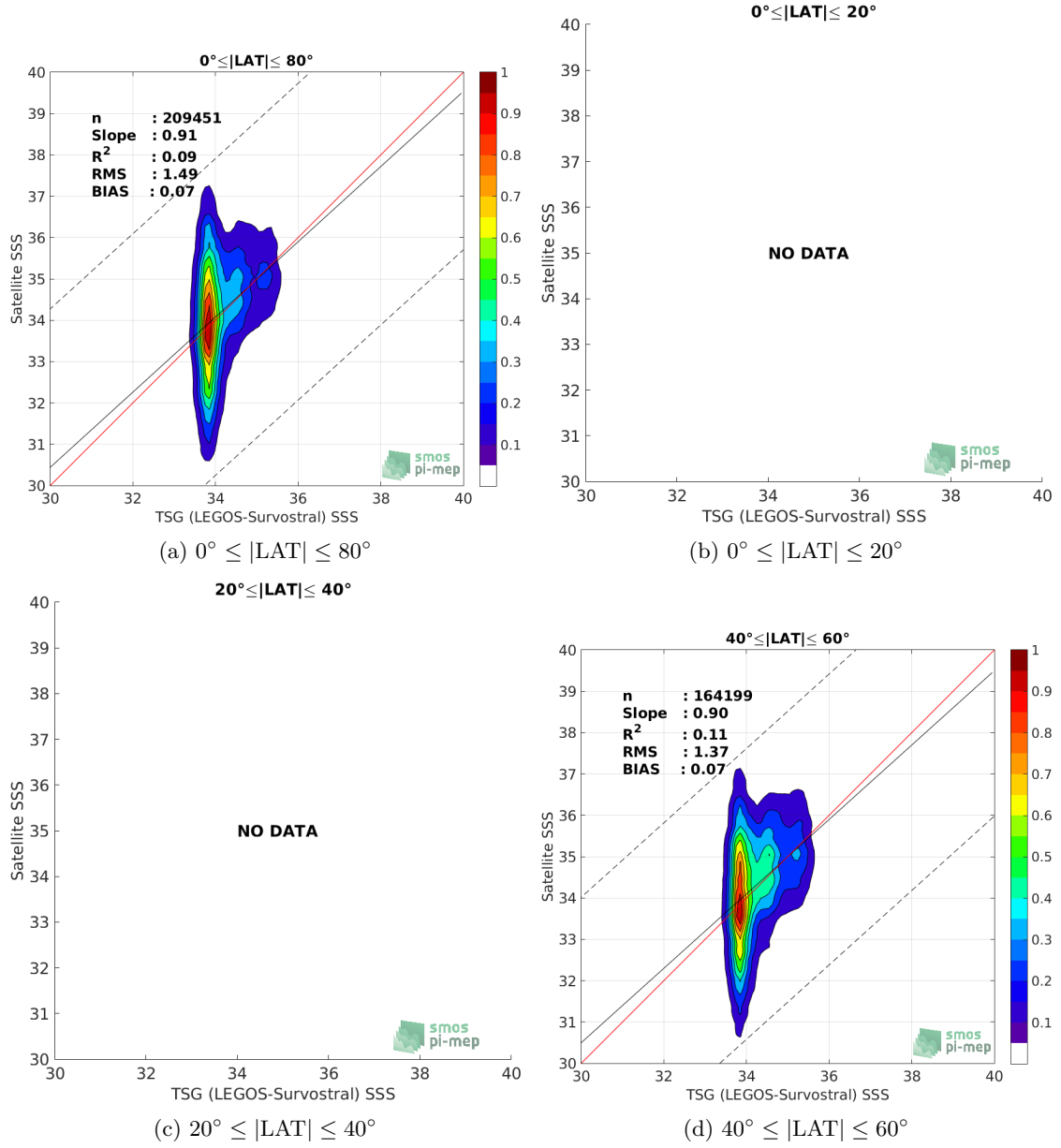
Figure 9: Contour maps of the concentration of SMOS SSS L2Q v321 - 0.25 Deg (CATDS-CPDC) SSS (y-axis) versus TSG (LEGOS-Survostral) SSS (x-axis) at match-up pairs for different latitude bands. For each plot, the red line shows x=y . The black thin and dashed lines indicate a linear fit through the data cloud and the \pm 95\% confidence levels, respectively. The number match-up pairs n , the slope and R^2 coefficient of the linear fit, the root mean square (RMS) and the mean bias between satellite and in situ data are indicated for each latitude band in each plots.
