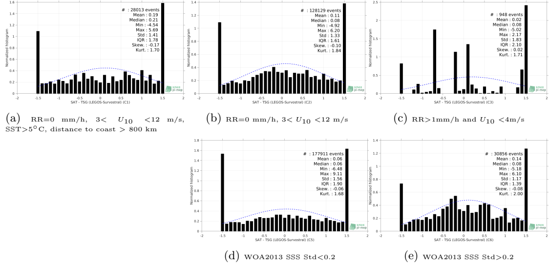
Figure 13: Normalized histogram of \Delta SSS (SMOS SSS L2Q v321 - 0.25 Deg (CATDS-CPDC) - TSG (LEGOS-Survostral)) for 5 different subdatasets corresponding to: RR=0 mm/h, 3 < U_{10} < 12 m/s, SST>5°C, distance to coast > 800 km (a), RR=0 mm/h, 3 < U_{10} < 12 m/s (b), RR>1mm/h and U_{10} < 4 m/s (c), WOA2013 SSS Std<0.2 (d), WOA2013 SSS Std>0.2 (e).
