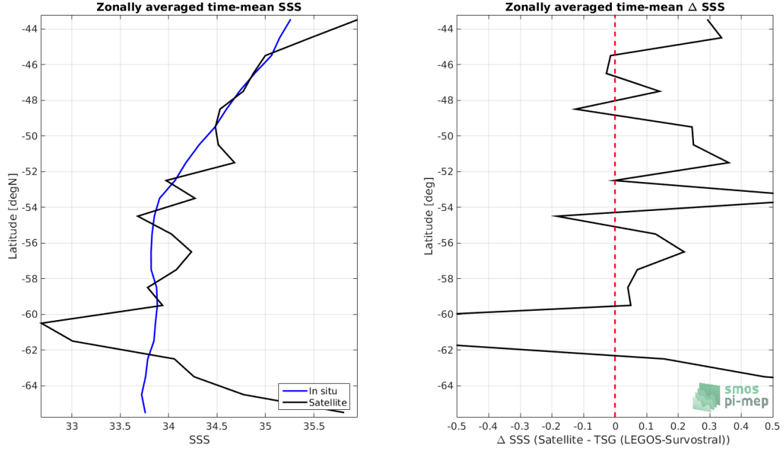
Figure 8: Left panel: Zonal mean SSS from SMOS SSS L2Q v321 - 0.25 Deg (CATDS-CPDC) satellite product (black) and from TSG (LEGOS-Survostral) (blue). Right panel: Zonal mean of \Delta SSS (Satellite - TSG (LEGOS-Survostral)) for all the collected Pi-MEP match-up pairs estimated over the full satellite product period.
