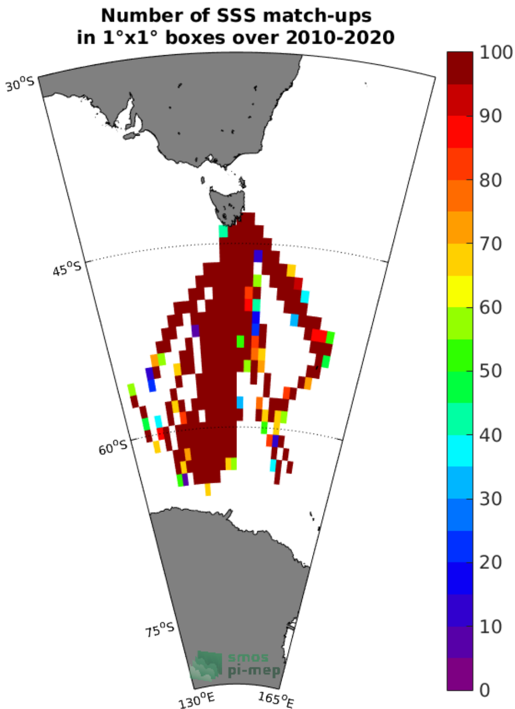
Figure 4: Number of SSS match-ups between TSG (LEGOS-Survostral) SSS and the SMOS SSS L2Q v321 - 0.25 Deg (CATDS-CPDC) SSS product for the Global Ocean Pi-MEP region over 1°x1° boxes and for the full satellite product period.
