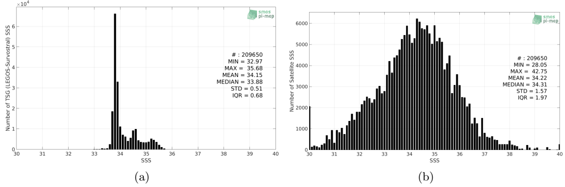
Figure 2: Histograms of SSS from TSG (LEGOS-Survostral) (a) and SMOS SSS L2Q v321 - 0.25 Deg (CATDS-CPDC) (b) considering all match-up pairs per bins of 0.1 over the Global Ocean Pi-MEP region and for the full satellite product period.
