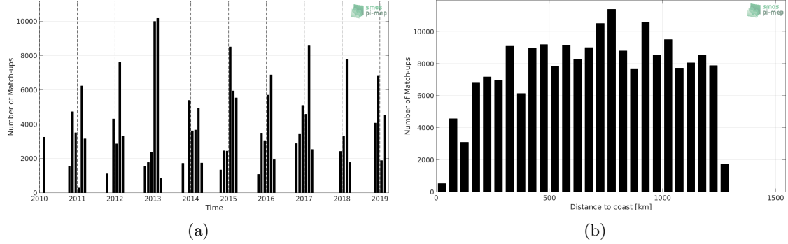
Figure 1: Number of match-ups between TSG-LEGOS-Survostral and SMOS L2Q v321 - 0.25 Deg (CATDS-CPDC) SSS as a function of time (a) and as function of the distance to coast (b) over the Global Ocean Pi-MEP region and for the full satellite product period.
