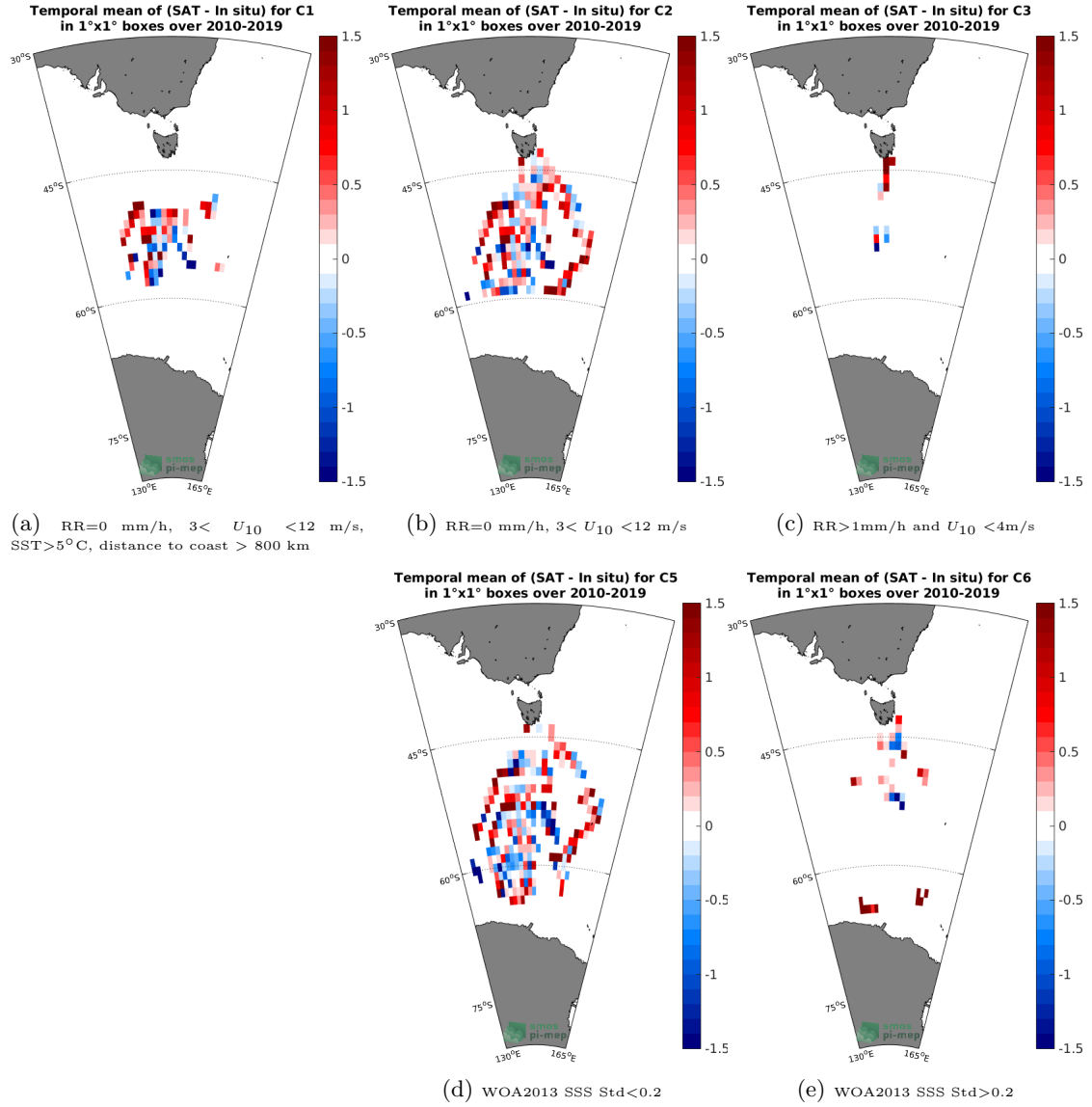
Figure 12: Temporal mean gridded over spatial boxes of size 1°x1° of \Delta\text{SSS} (SMOS L2Q v321 - 0.25 Deg (CATDS-CPDC) - TSG-LEGOS-Survostral) for 5 different subdatasets corresponding to: RR=0 mm/h, 3 < U_{10} < 12 m/s, SST > 5^\circ\text{C} , distance to coast > 800 km (a), RR=0 mm/h, 3 < U_{10} < 12 m/s (b), RR > 1\text{mm/h} and U_{10} < 4\text{m/s} (c), WOA2013 SSS Std < 0.2 (d), WOA2013 SSS Std > 0.2 (e).
