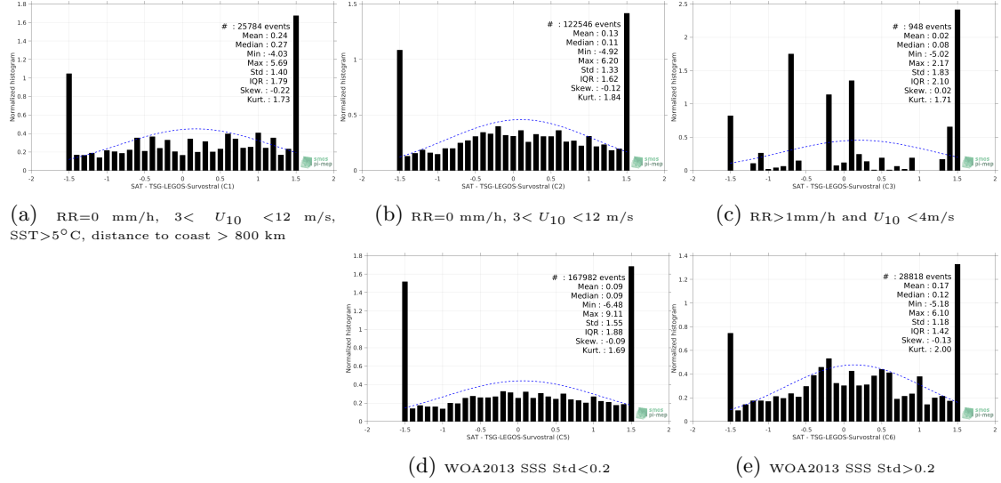
Figure 13: Normalized histogram of \Delta SSS (SMOS L2Q v321 - 0.25 Deg (CATDS-CPDC) - TSG-LEGOS-Survostral) for 5 different subdatasets corresponding to: RR=0 mm/h, 3 < U_{10} < 12 m/s, SST > 5°C, distance to coast > 800 km (a), RR=0 mm/h, 3 < U_{10} < 12 m/s (b), RR > 1mm/h and U_{10} < 4 m/s (c), WOA2013 SSS Std < 0.2 (d), WOA2013 SSS Std > 0.2 (e).
