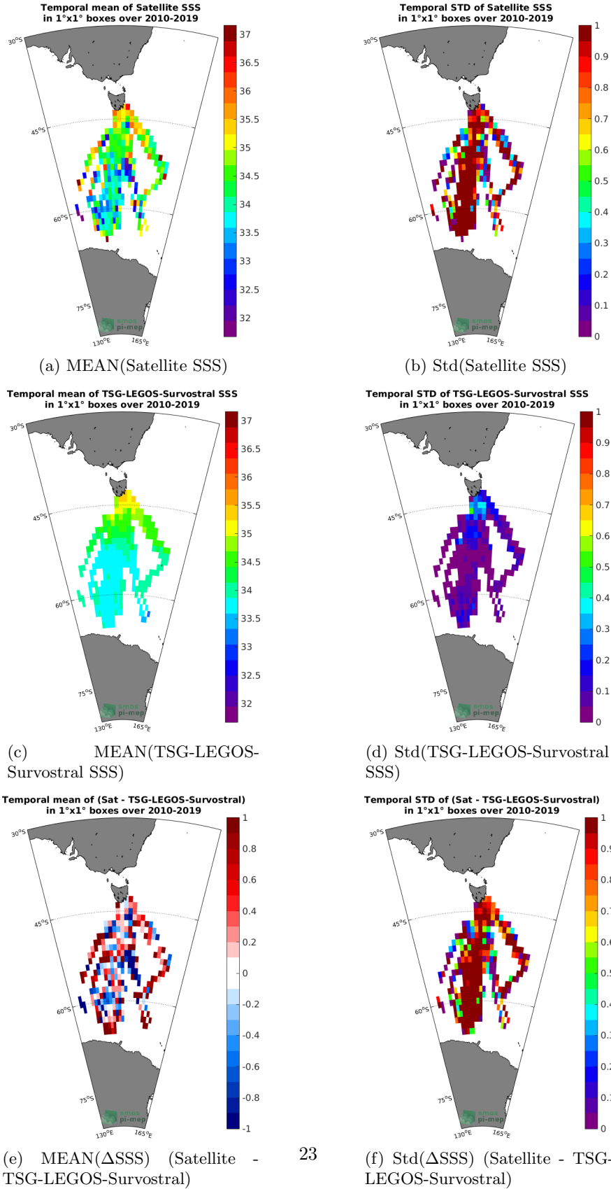
Figure 6: Temporal mean (left) and Std (right) of SSS from SMOS L2Q v321 - 0.25 Deg (CATDS-CPDC) (top), TSG-LEGOS-Survostral (middle), and of \Delta SSS (Satellite - TSG-LEGOS-Survostral). Only match-up pairs are used to generate these maps.
