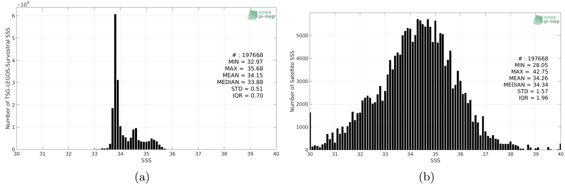
Figure 2: Histograms of SSS from TSG-LEGOS-Survostral (a) and SMOS L2Q v321 - 0.25 Deg (CATDS-CPDC) (b) considering all match-up pairs per bins of 0.1 over the Global Ocean Pi-MEP region and for the full satellite product period.
