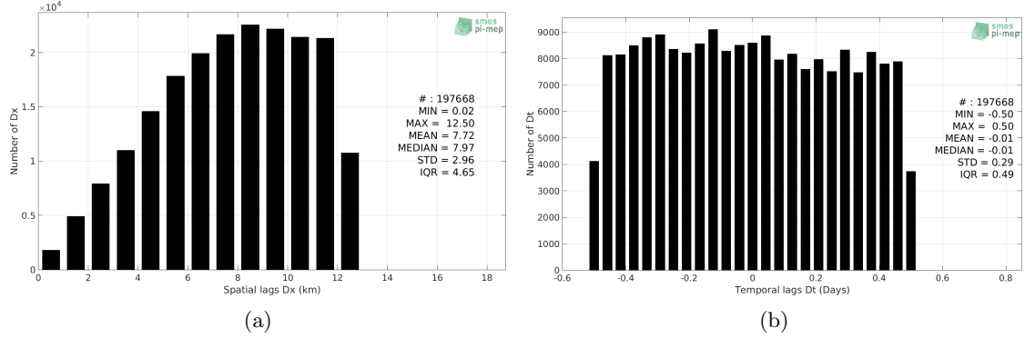
Figure 5: Histograms of the spatial (a) and temporal (b) lags between the time of the TSG-LEGOS-Survostral measurements and the date of the corresponding SMOS L2Q v321 - 0.25 Deg (CATDS-CPDC) SSS product.
