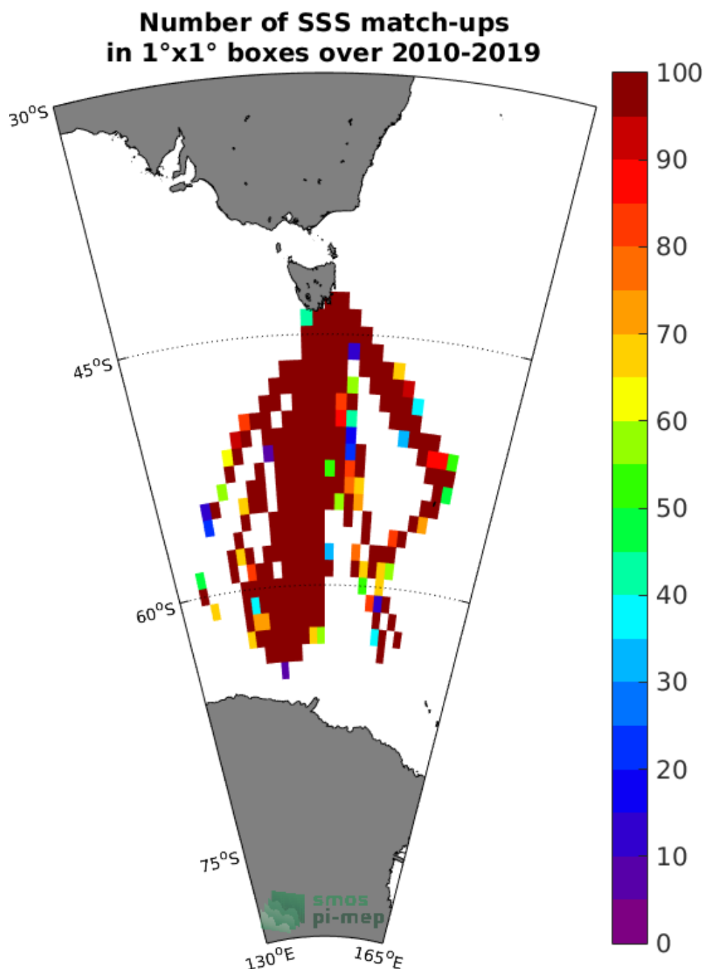
Figure 4: Number of SSS match-ups between TSG-LEGOS-Survostral SSS and the SMOS L2Q v321 - 0.25 Deg (CATDS-CPDC) SSS product for the Global Ocean Pi-MEP region over 1°x1° boxes and for the full satellite product period.
