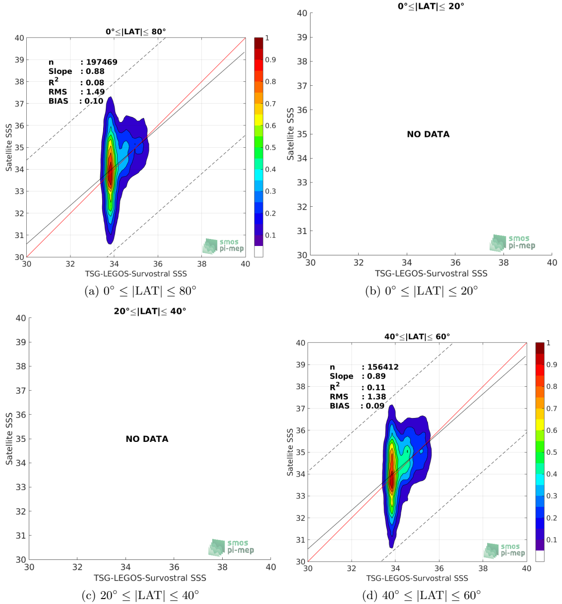
Figure 9: Contour maps of the concentration of SMOS L2Q v321 - 0.25 Deg (CATDS-CPDC') SSS (y-axis) versus TSG-LEGOS-Survostral SSS (x-axis) at match-up pairs for different latitude bands. For each plot, the red line shows x=y . The black thin and dashed lines indicate a linear fit through the data cloud and the \pm 95\% confidence levels, respectively. The number match-up pairs n , the slope and R^2 coefficient of the linear fit, the root mean square (RMS) and the mean bias between satellite and in situ data are indicated for each latitude band in each plots.
