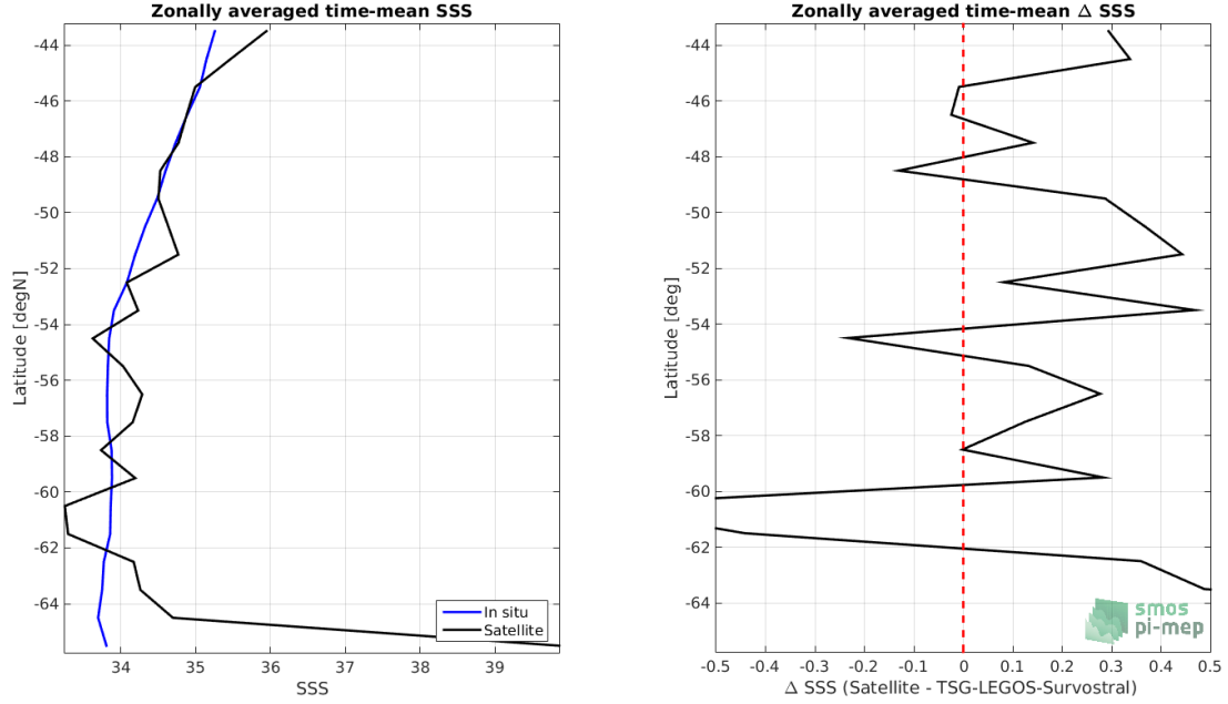
Figure 8: Left panel: Zonal mean SSS from SMOS L2Q v321 - 0.25 Deg (CATDS-CPDC) satellite product (black) and from TSG-LEGOS-Survostral (blue). Right panel: Zonal mean of \Delta SSS (Satellite - TSG-LEGOS-Survostral) for all the collected Pi-MEP match-up pairs estimated over the full satellite product period.
