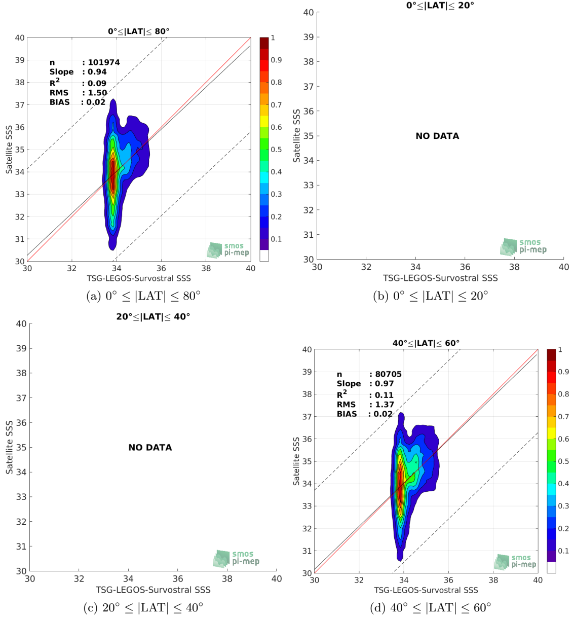
Figure 9: Contour maps of the concentration of SMOS-L3-CATDS-CPDC-V321-L2Q SSS (y-axis) versus TSG-LEGOS-Survostral SSS (x-axis) at match-up pairs for different latitude bands. For each plot, the red line shows x=y . The black thin and dashed lines indicate a linear fit through the data cloud and the \pm 95\% confidence levels, respectively. The number match-up pairs n , the slope and R^2 coefficient of the linear fit, the root mean square (RMS) and the mean bias between satellite and in situ data are indicated for each latitude band in each plots.
