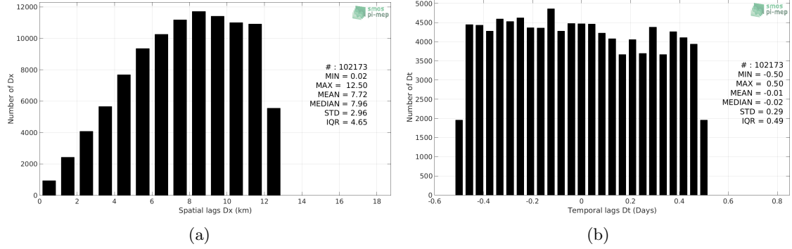
Figure 5: Histograms of the spatial (a) and temporal (b) lags between the time of the TSG-LEGOS-Survostral measurements and the date of the corresponding SMOS-L3-CATDS-CPDC-V321-L2Q SSS product.
