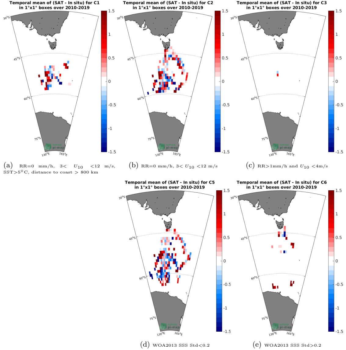
Figure 12: Temporal mean gridded over spatial boxes of size 1°x1° of \Delta\text{SSS} (SMOS-L3-CATDS-CPDC-V321-L2Q - TSG-LEGOS-Survostral) for 5 different subdatasets corresponding to: RR=0 mm/h, 3 < U_{10} < 12 m/s, SST > 5^\circ\text{C} , distance to coast > 800 km (a), RR=0 mm/h, 3 < U_{10} < 12 m/s (b), RR > 1 mm/h and U_{10} < 4 m/s (c), WOA2013 SSS Std < 0.2 (d), WOA2013 SSS Std > 0.2 (e).
