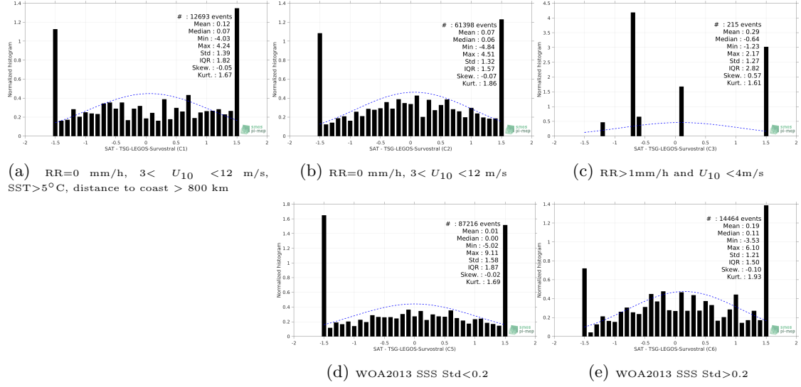
Figure 13: Normalized histogram of \Delta SSS (SMOS-L3-CATDS-CPDC-V321-L2Q - TSG-LEGOS-Survostral) for 5 different subdatasets corresponding to: RR=0 mm/h, 3 < U_{10} < 12 m/s, SST > 5°C, distance to coast > 800 km (a), RR=0 mm/h, 3 < U_{10} < 12 m/s (b), RR > 1mm/h and U_{10} < 4 m/s (c), WOA2013 SSS Std < 0.2 (d), WOA2013 SSS Std > 0.2 (e).
