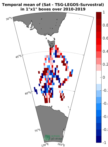
(e) MEAN( \Delta SSS) (Satellite - TSG-LEGOS-Survostral)
