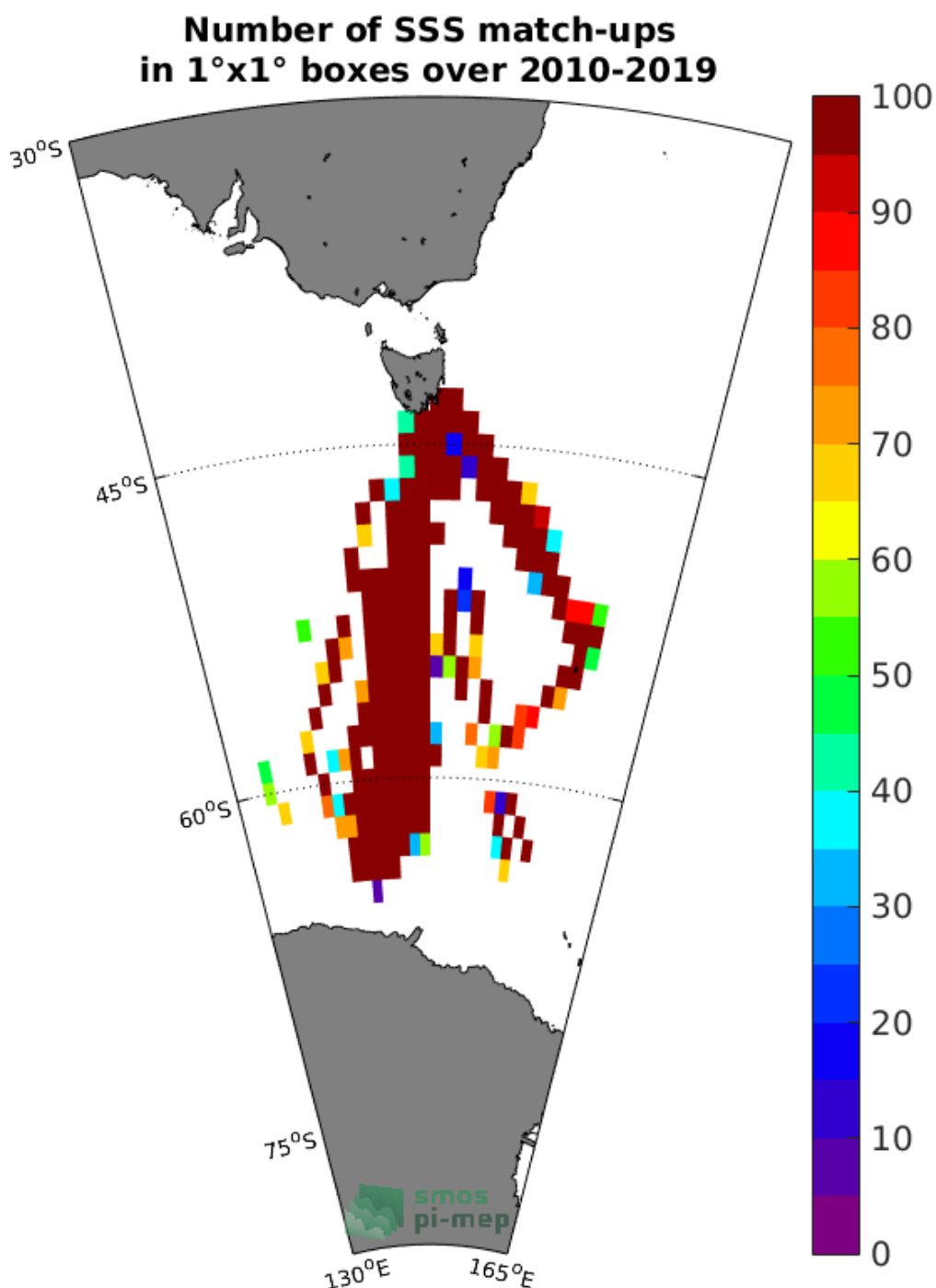
Figure 4: Number of SSS match-ups between TSG-LEGOS-Survostral SSS and the SMOS-L3-CATDS-CPDC-V321-L2Q SSS product for the Global Ocean Pi-MEP region over 1°x1° boxes and for the full satellite product period.
