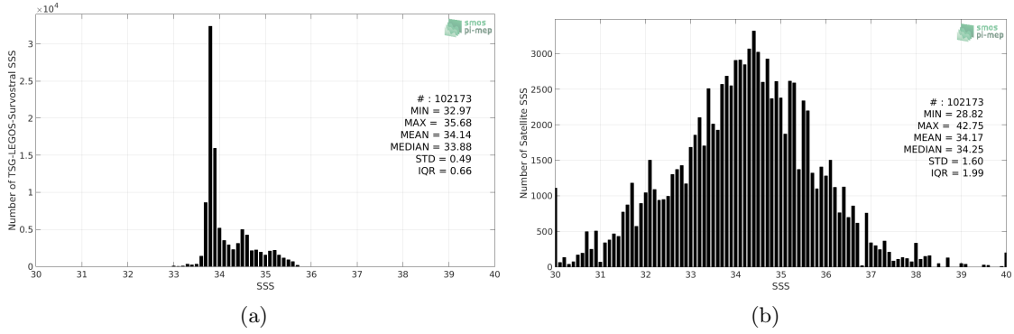
Figure 2: Histograms of SSS from TSG-LEGOS-Survostral (a) and SMOS-L3-CATDS-CPDC-V321-L2Q (b) considering all match-up pairs per bins of 0.1 over the Global Ocean Pi-MEP region and for the full satellite product period.
