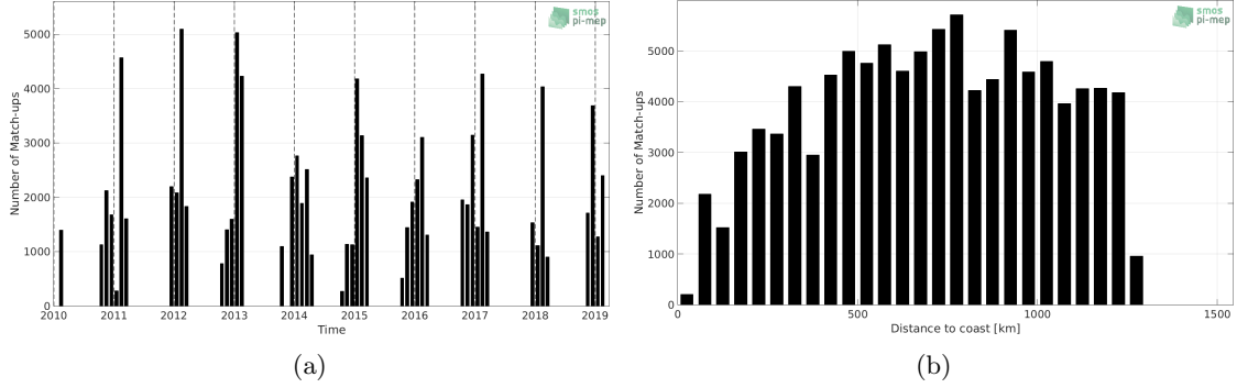
Figure 1: Number of match-ups between TSG-LEGOS-Survostral and SMOS-L3-CATDS-CPDC-V321-L2Q SSS as a function of time (a) and as function of the distance to coast (b) over the Global Ocean Pi-MEP region and for the full satellite product period.
