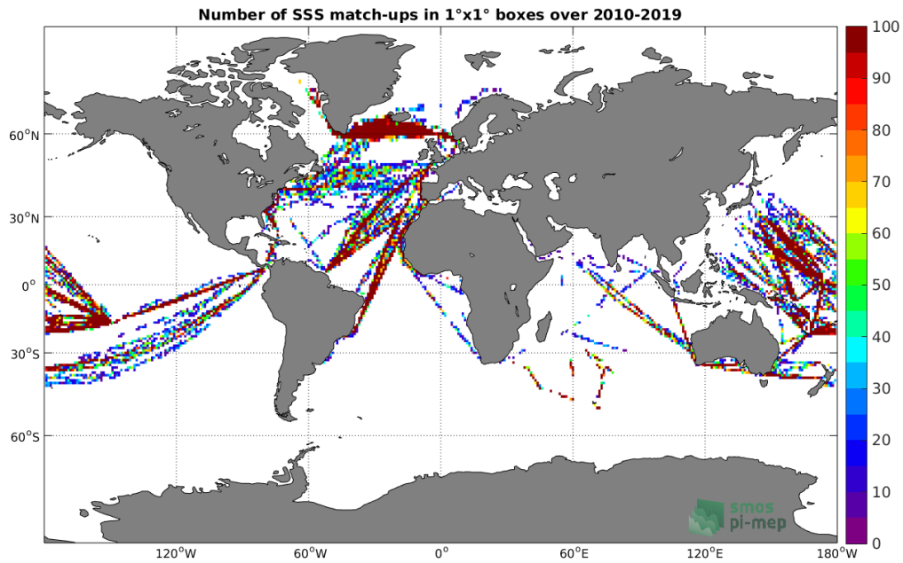
Figure 4: Number of SSS match-ups between TSG (LEGOS-DM) SSS and the SMOS SSS L2Q v321 - 0.25 Deg (CATDS-CPDC) SSS product for the Global Ocean Pi-MEP region over 1^\circ \times 1^\circ boxes and for the full satellite product period.
