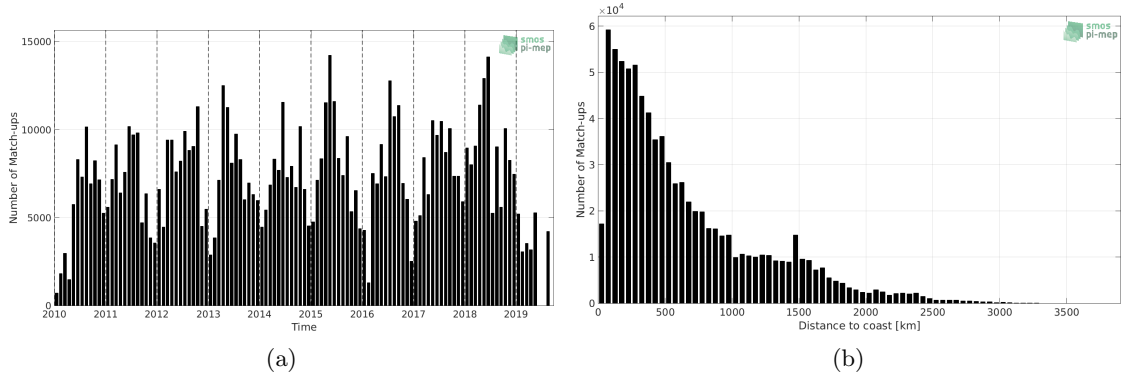
Figure 1: Number of match-ups between TSG-LEGOS-DM and SMOS L2Q v321 - 0.25 Deg (CATDS-CPDC) SSS as a function of time (a) and as function of the distance to coast (b) over the Global Ocean Pi-MEP region and for the full satellite product period.
