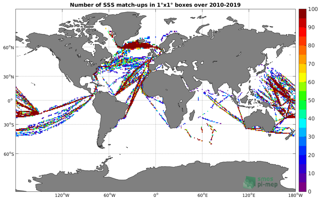
Figure 4: Number of SSS match-ups between TSG-LEGOS-DM SSS and the SMOS L2Q v321 - 0.25 Deg (CATDS-CPDC) SSS product for the Global Ocean Pi-MEP region over 1°x1° boxes and for the full satellite product period.
