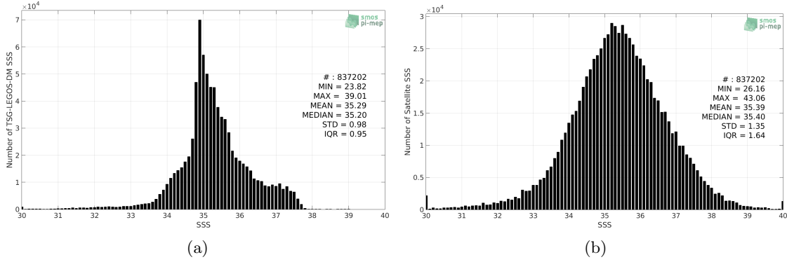
Figure 2: Histograms of SSS from TSG-LEGOS-DM (a) and SMOS L2Q v321 - 0.25 Deg (CATDS-CPDC) (b) considering all match-up pairs per bins of 0.1 over the Global Ocean Pi-MEP region and for the full satellite product period.
