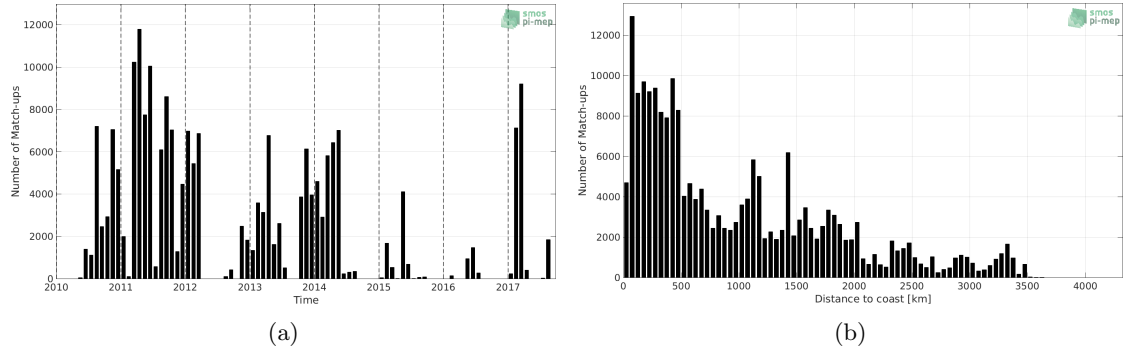
Figure 1: Number of match-ups between TSG (GOSUD-Sailing-ship) and SMOS SSS L2Q v321 - 0.25 Deg (CATDS-CPDC) SSS as a function of time (a) and as function of the distance to coast (b) over the Global Ocean Pi-MEP region and for the full satellite product period.
