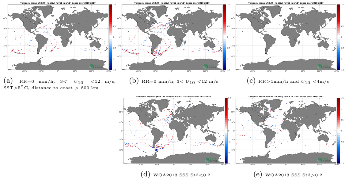
Figure 12: Temporal mean gridded over spatial boxes of size 1^\circ \times 1^\circ of \Delta SSS (SMOS SSS L2Q v321 - 0.25 Deg (CATDS-CPDC) - TSG (GOSUD-Sailing-ship)) for 5 different subdatasets corresponding to: RR=0 mm/h, 3 < U_{10} < 12 m/s, SST>5°C, distance to coast > 800 km (a), RR=0 mm/h, 3 < U_{10} < 12 m/s (b), RR>1mm/h and U_{10} < 4 m/s (c), WOA2013 SSS Std<0.2 (d), WOA2013 SSS Std>0.2 (e).
