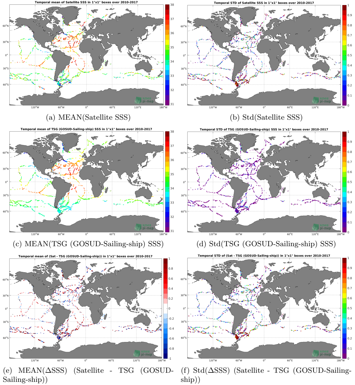
Figure 6: Temporal mean (left) and Std (right) of SSS from SMOS SSS L2Q v321 - 0.25 Deg (CATDS-CPDC) (top), TSG (GOSUD-Sailing-ship) (middle), and of \Delta SSS (Satellite - TSG (GOSUD-Sailing-ship)). Only match-up pairs are used to generate these maps.
