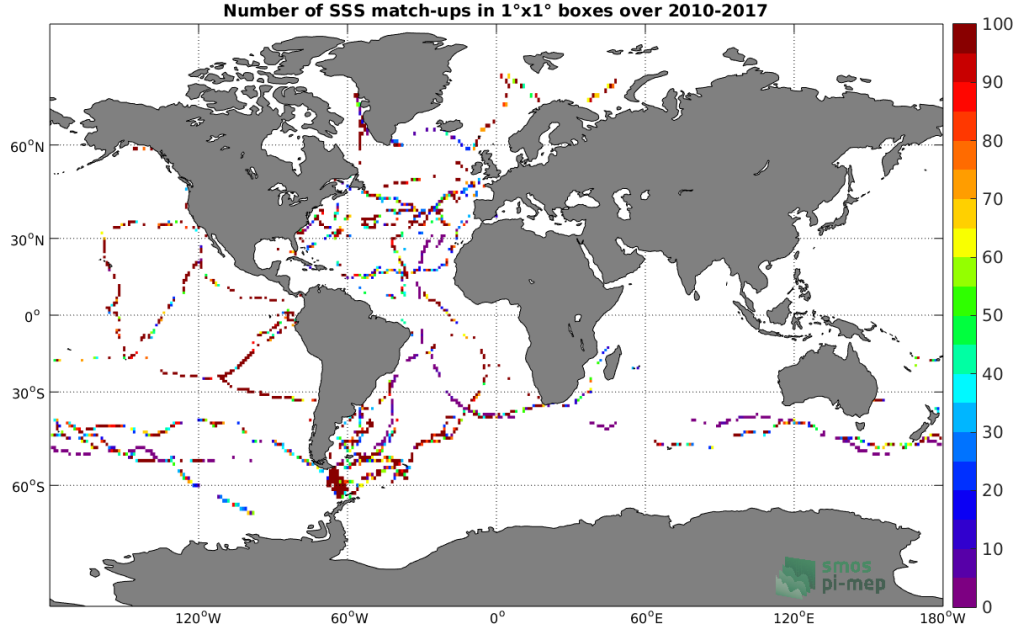
Figure 4: Number of SSS match-ups between TSG (GOSUD-Sailing-ship) SSS and the SMOS SSS L2Q v321 - 0.25 Deg (CATDS-CPDC) SSS product for the Global Ocean Pi-MEP region over 1^\circ \times 1^\circ boxes and for the full satellite product period.
