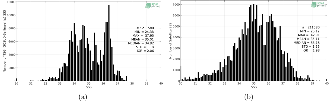
Figure 2: Histograms of SSS from TSG (GOSUD-Sailing-ship) (a) and SMOS SSS L2Q v321 - 0.25 Deg (CATDS-CPDC) (b) considering all match-up pairs per bins of 0.1 over the Global Ocean Pi-MEP region and for the full satellite product period.
